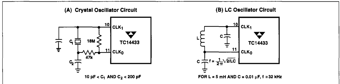
Figure 9. Alternate Oscillator Circuits
