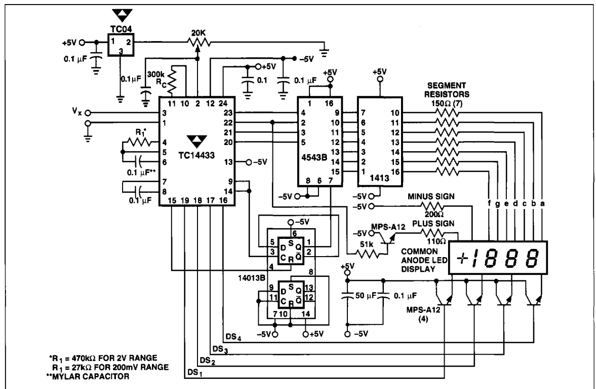
Figure 10. 3-1/2 Digit Voltmeter Common-Anode Displays, Flashing Overrange
