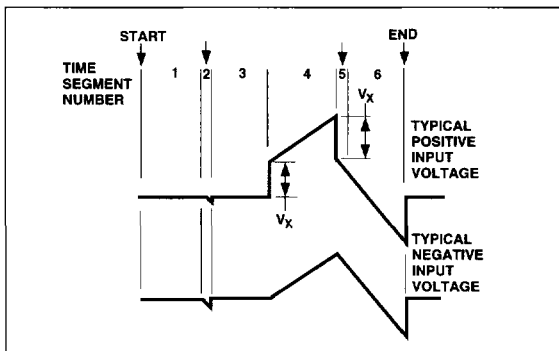
Figure 7. Integrator Waveforms at Pin 6
