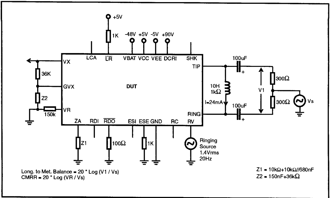
Figure 11 - Longitudinal to Metallic Balance & CMRR Test Circuit
