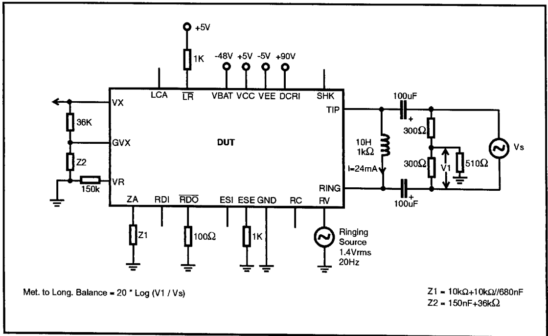
Figure 12 - Metallic to Longitudinal Balance
