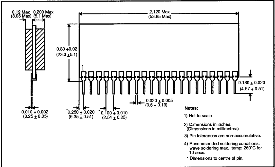
Figure 13 - Mechanical Data for 21 Pin SIL Hybrid
