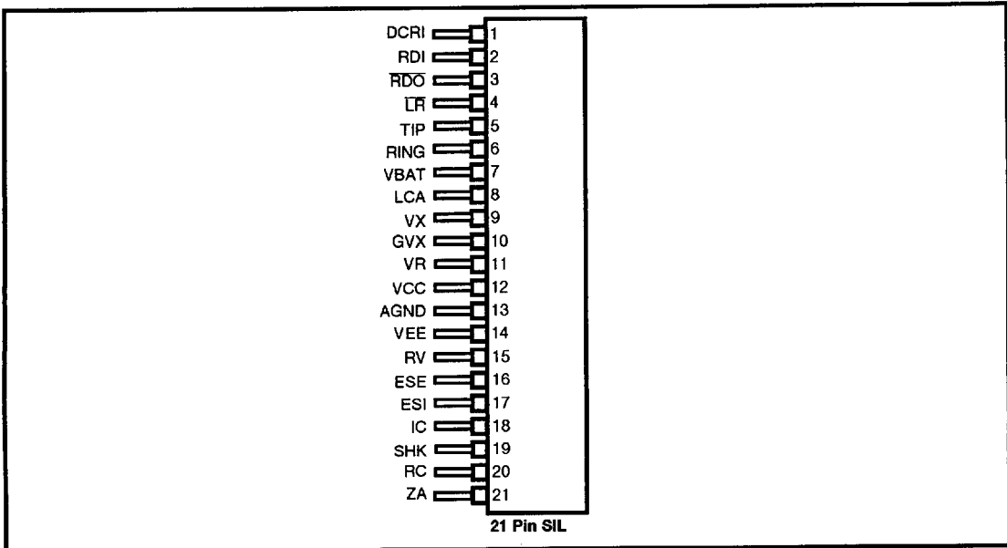
Figure 2 - Pin Connections
