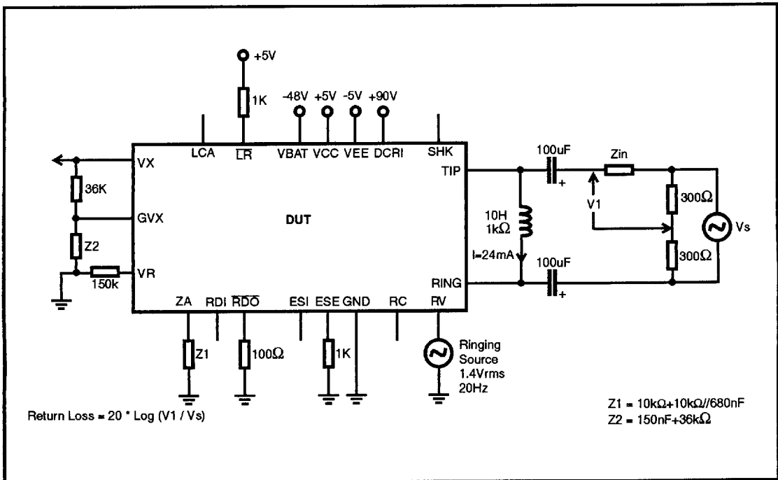
Figure 10 - Return Loss
