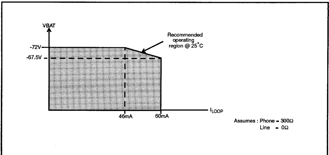
Figure 5 - Safe Operating Region
