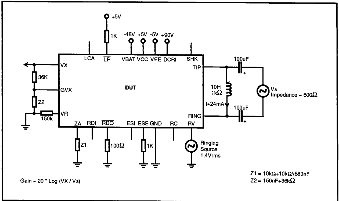
Figure 8 - 2-4 Gain Wire Test Circuit
