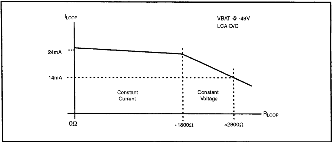
Figure 6 - Loop Current v Line Resistance
