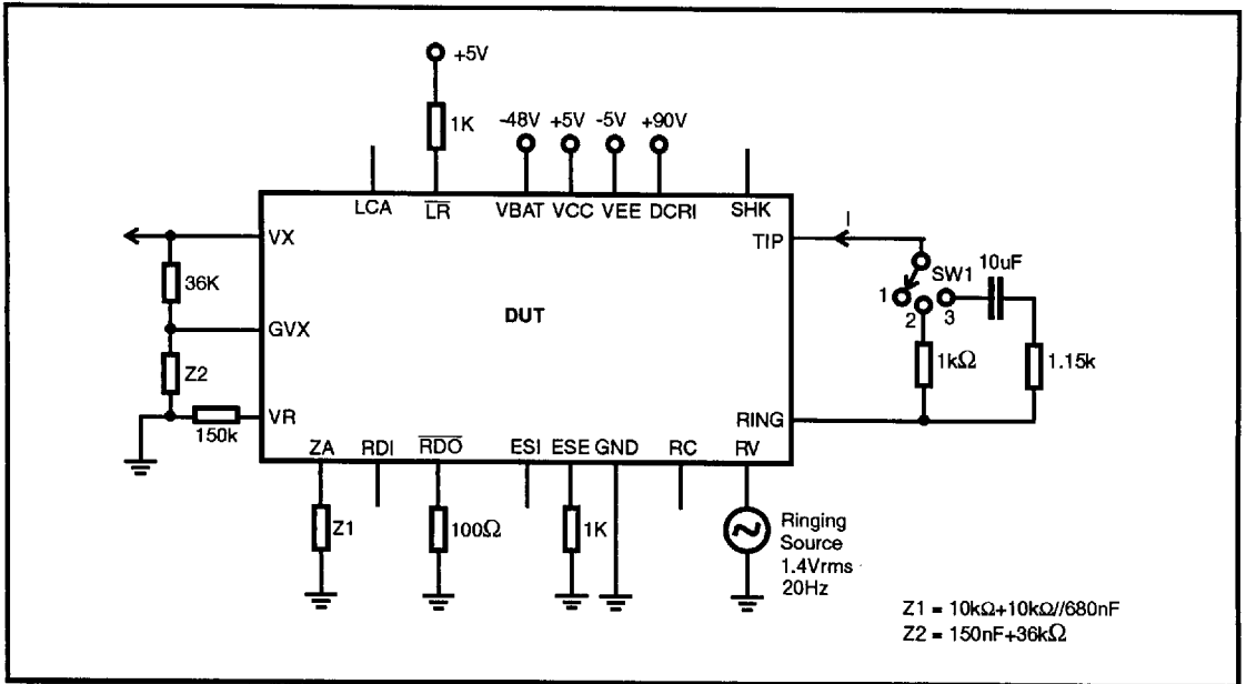
Figure 7 - DC Condition Test
