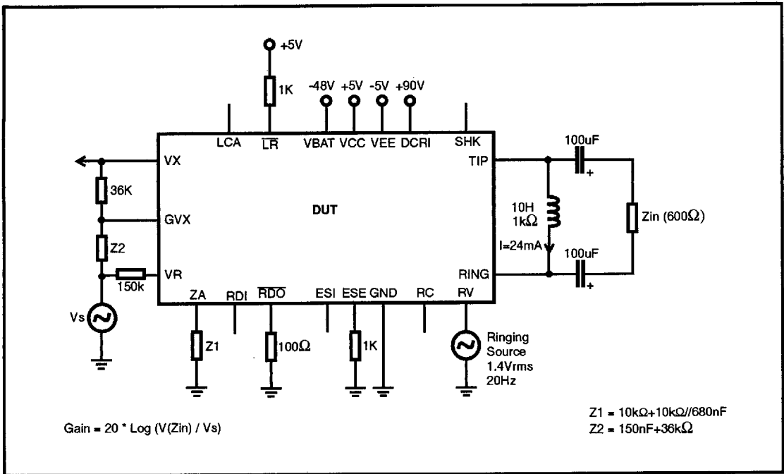
Figure 9 - 4-2 Wire Gain Test Circuit
