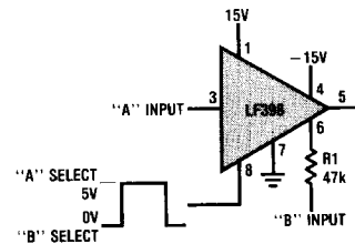
2-Channel Switch
