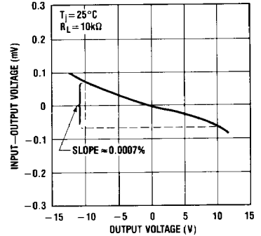
Gain Error
