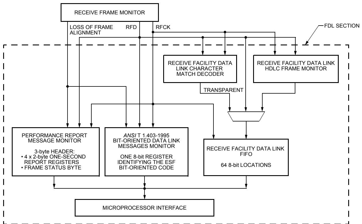
Figure 25. Block Diagram of the Receive Facility Data Link
