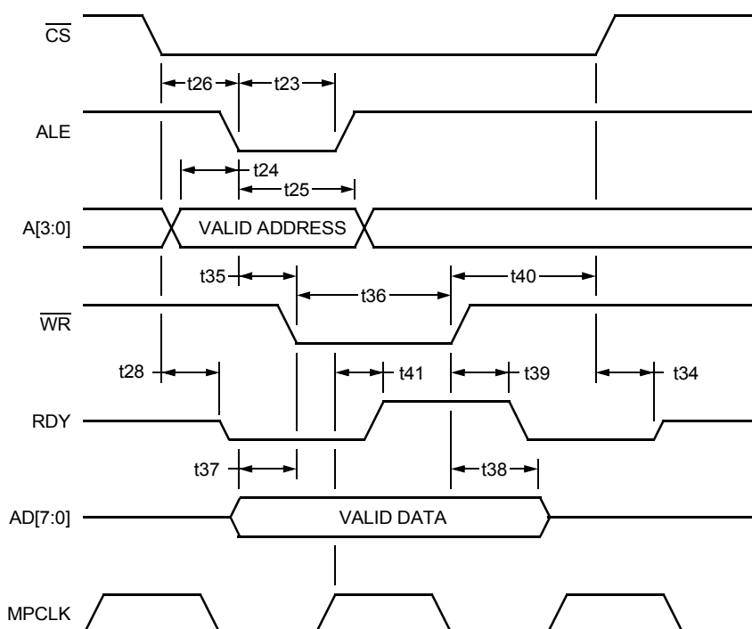
Figure 32. Mode 3—Write Cycle Timing (MPMODE = 1, MPMUX = 0)
