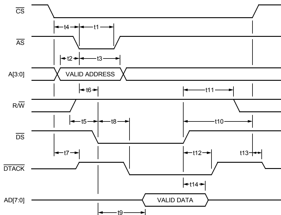
Figure 27. Mode 1—Read Cycle Timing (MPMODE = 0, MPMUX = 0)
