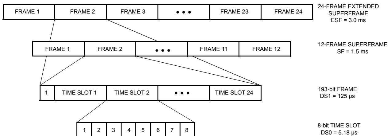
Figure 19. T1 Frame Structure
