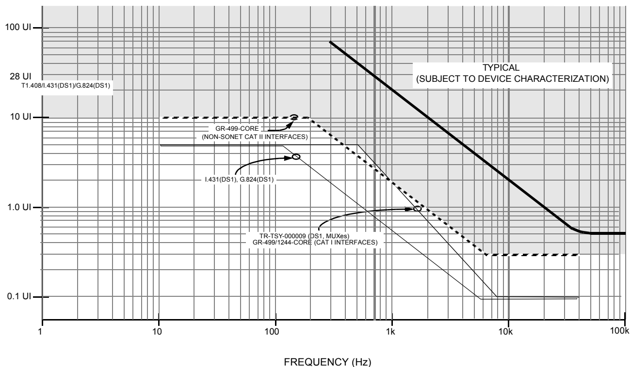
Figure 6. DS1/T1 Receiver Jitter Accommodation Without Jitter Attenuator
