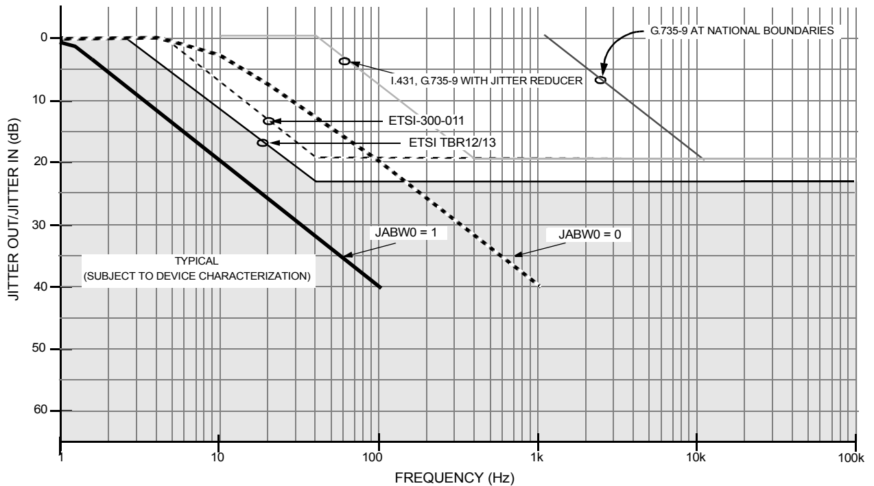
Figure 15. CEPT/E1 Jitter Transfer of the Jitter Attenuator
