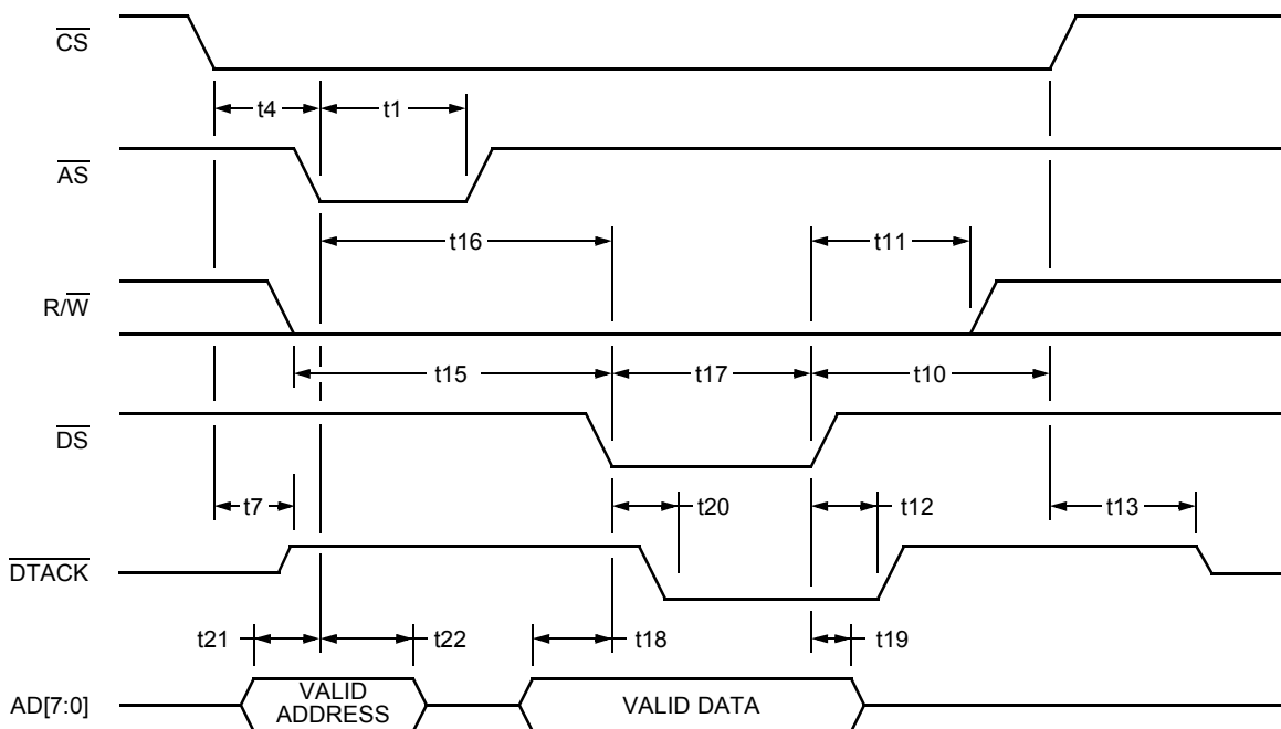
Figure 30. Mode 2—Write Cycle Timing (MPMODE = 0, MPMUX = 1)
