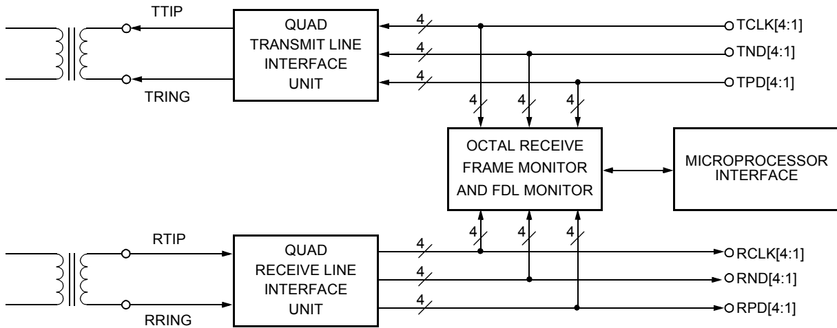
Figure 16. Block Diagram of the Receive Frame Monitor Section
