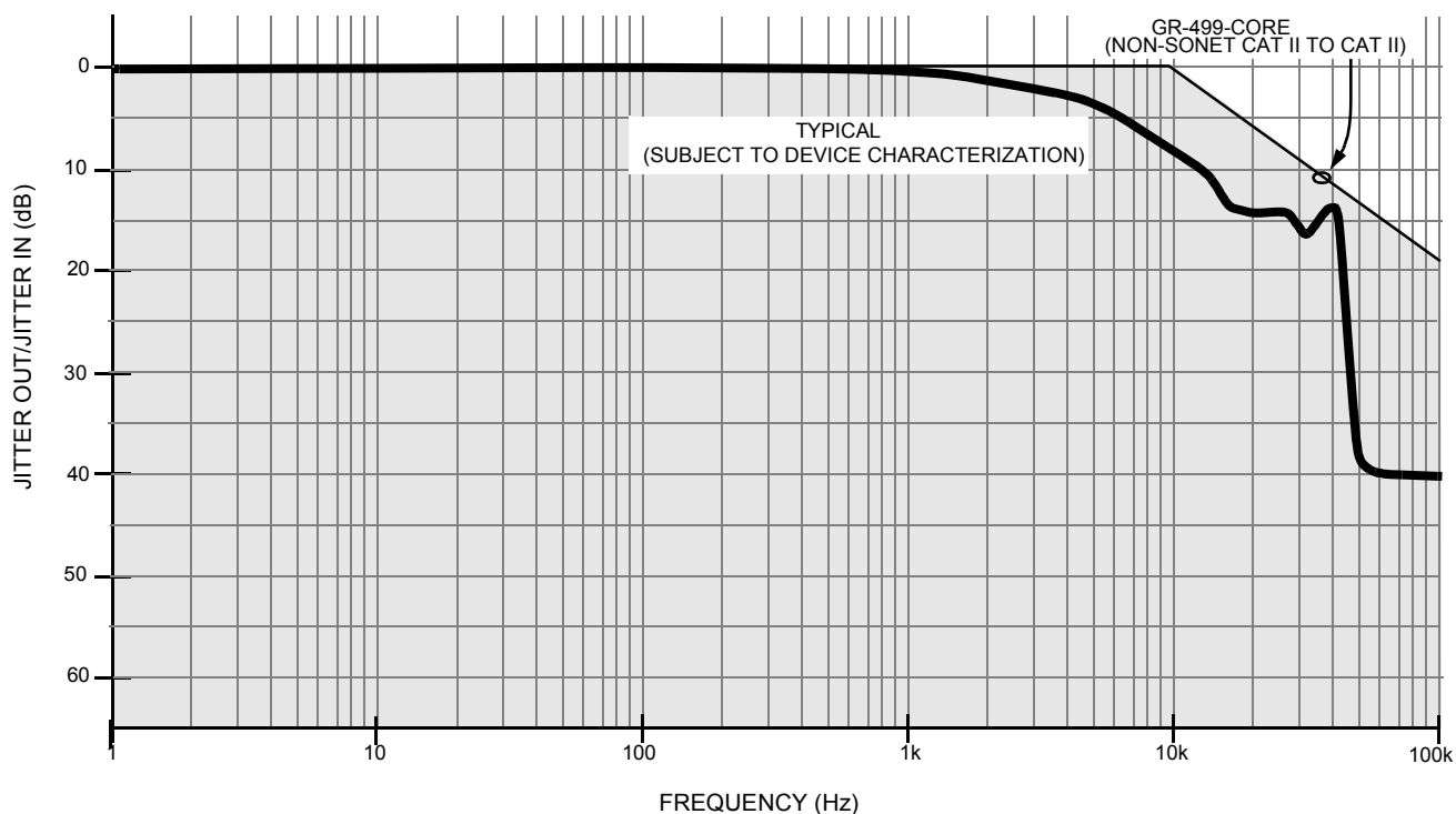
Figure 7. DS1/T1 Receiver Jitter Transfer Without Jitter Attenuator
