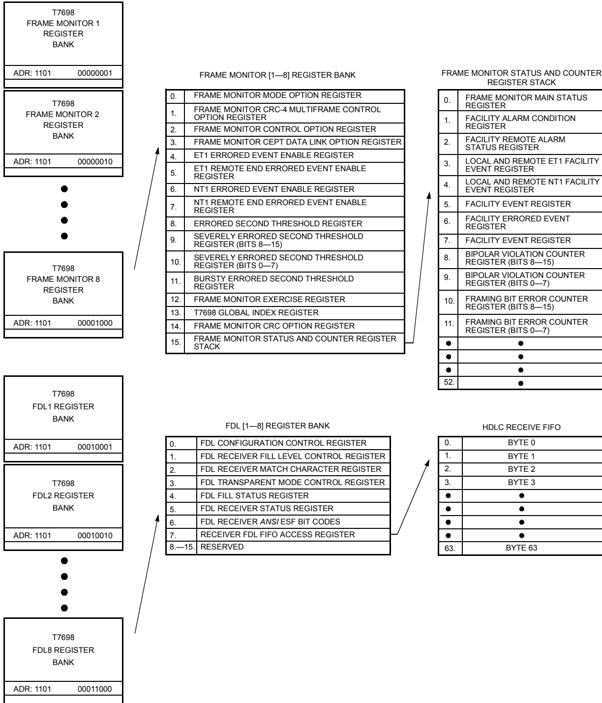
Figure 4. T7698's Secondary Register Bank Architecture
