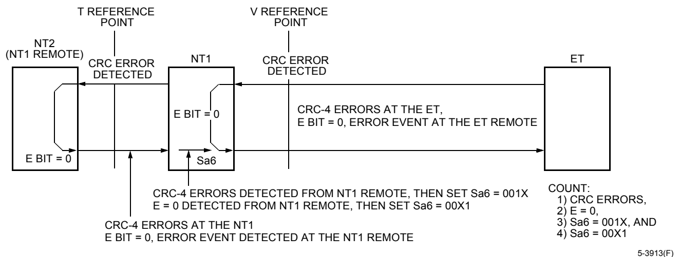
Figure 24. The T and V Reference Points for a Typical CEPT E1 Application
