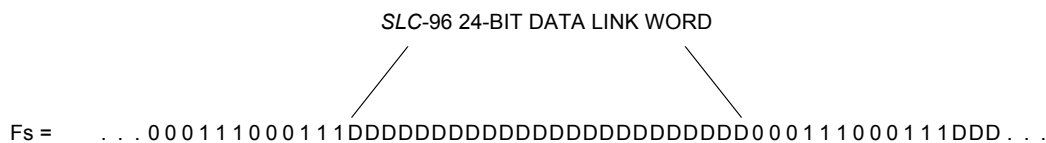
Figure 20. SLC-96 Frame Format
