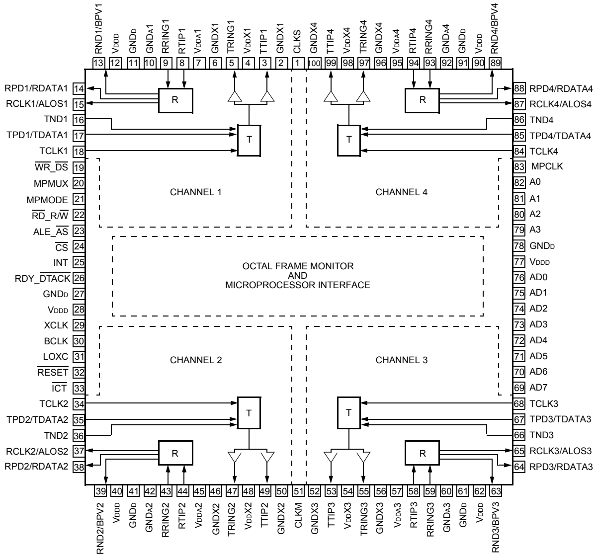
Figure 2. T7698 Pin Diagram (BQFP)
