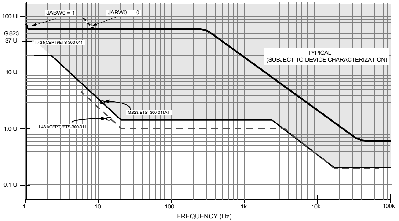
Figure 14. CEPT/E1 Receiver Jitter Accommodation with Jitter Attenuator
