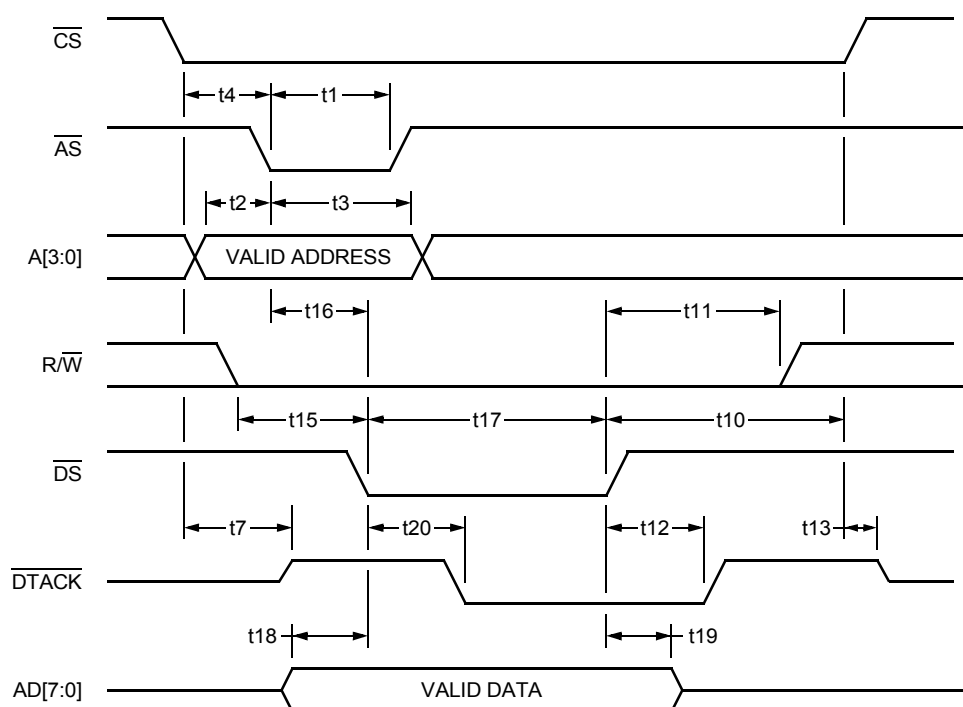
Figure 28. Mode 1—Write Cycle Timing (MPMODE = 0, MPMUX = 0)
