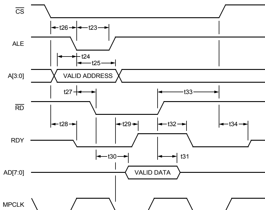
Figure 31. Mode 3—Read Cycle Timing (MPMODE = 1, MPMUX = 0)
