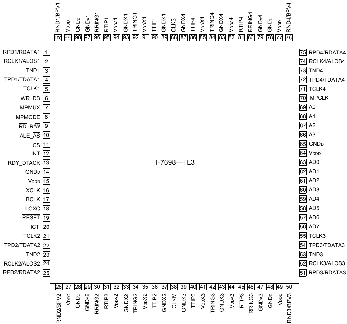
Figure 3. T7698 Pin Diagram (TQFP)
