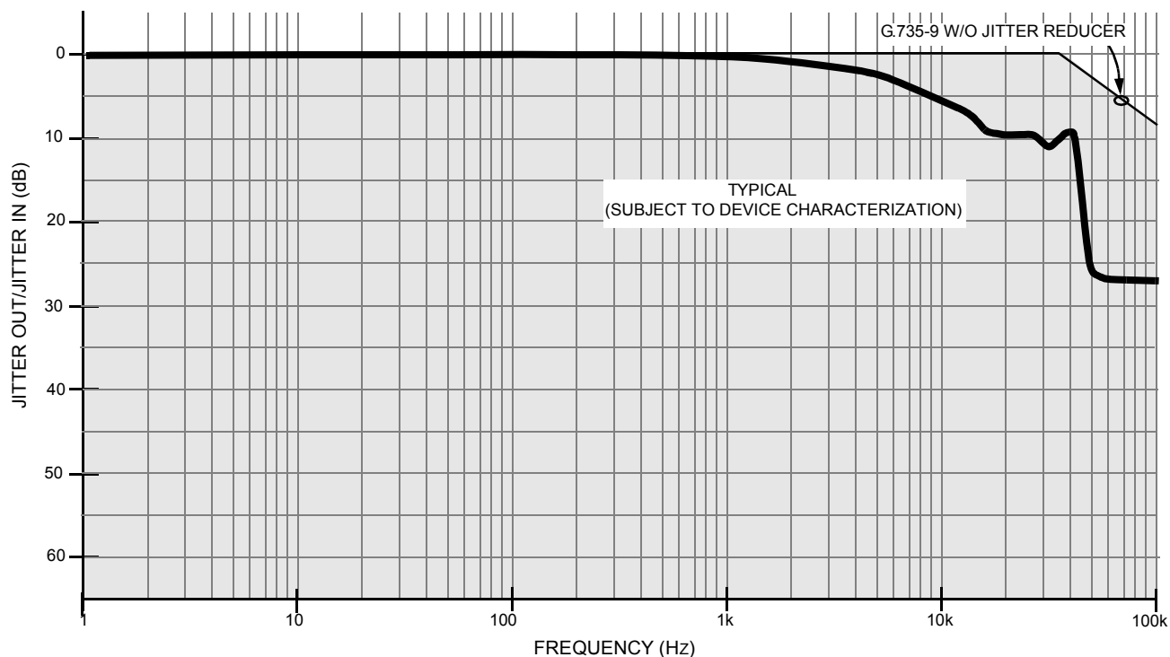
Figure 9. CEPT/E1 Receiver Jitter Transfer Without Jitter Attenuator
