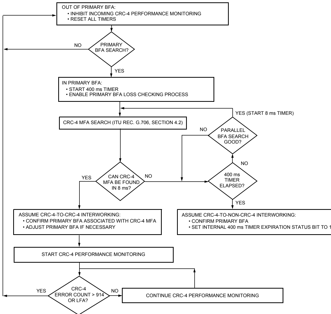
Figure 23. CEPT Loss of CRC-4 Multiframe Alignment Recovery Algorithms: T7698 Receive CRC-4 Multiframe Search Algorithm for Automatic, CRC-4/ Non-CRC-4 Equipment Interworking as Defined by ITU (from ITU Rec. G.706, Annex B.2.2 - 1991)
