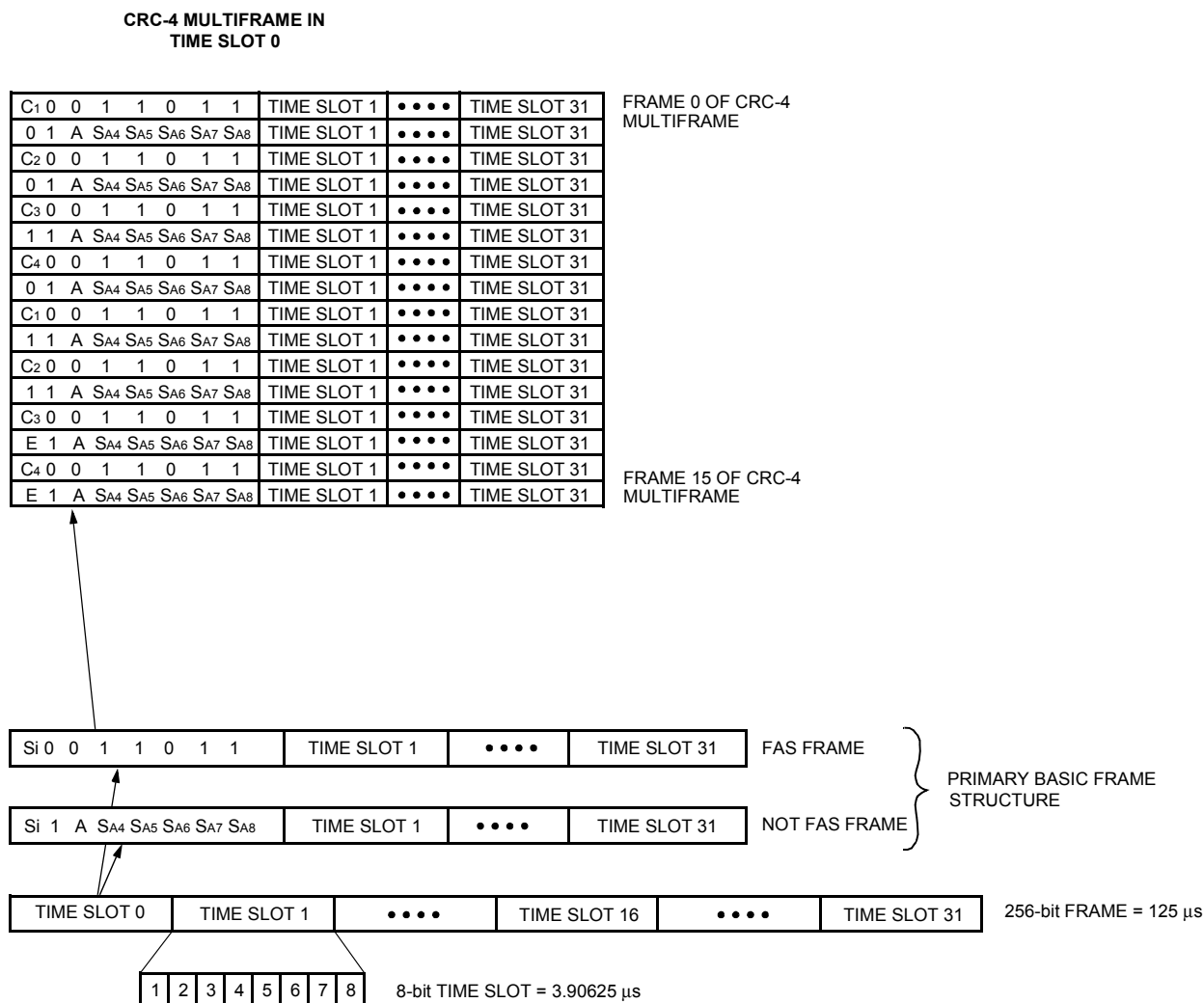
Figure 21. ITU 2.048 Mbits/s Basic Frame and CRC-4 Multiframe Structures
