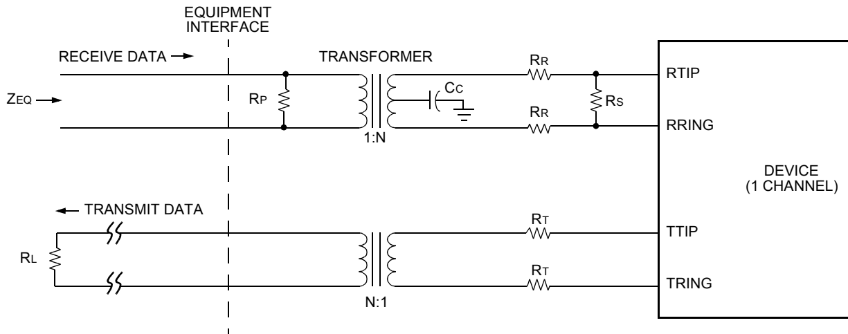
Figure 26. Line Termination Circuitry
