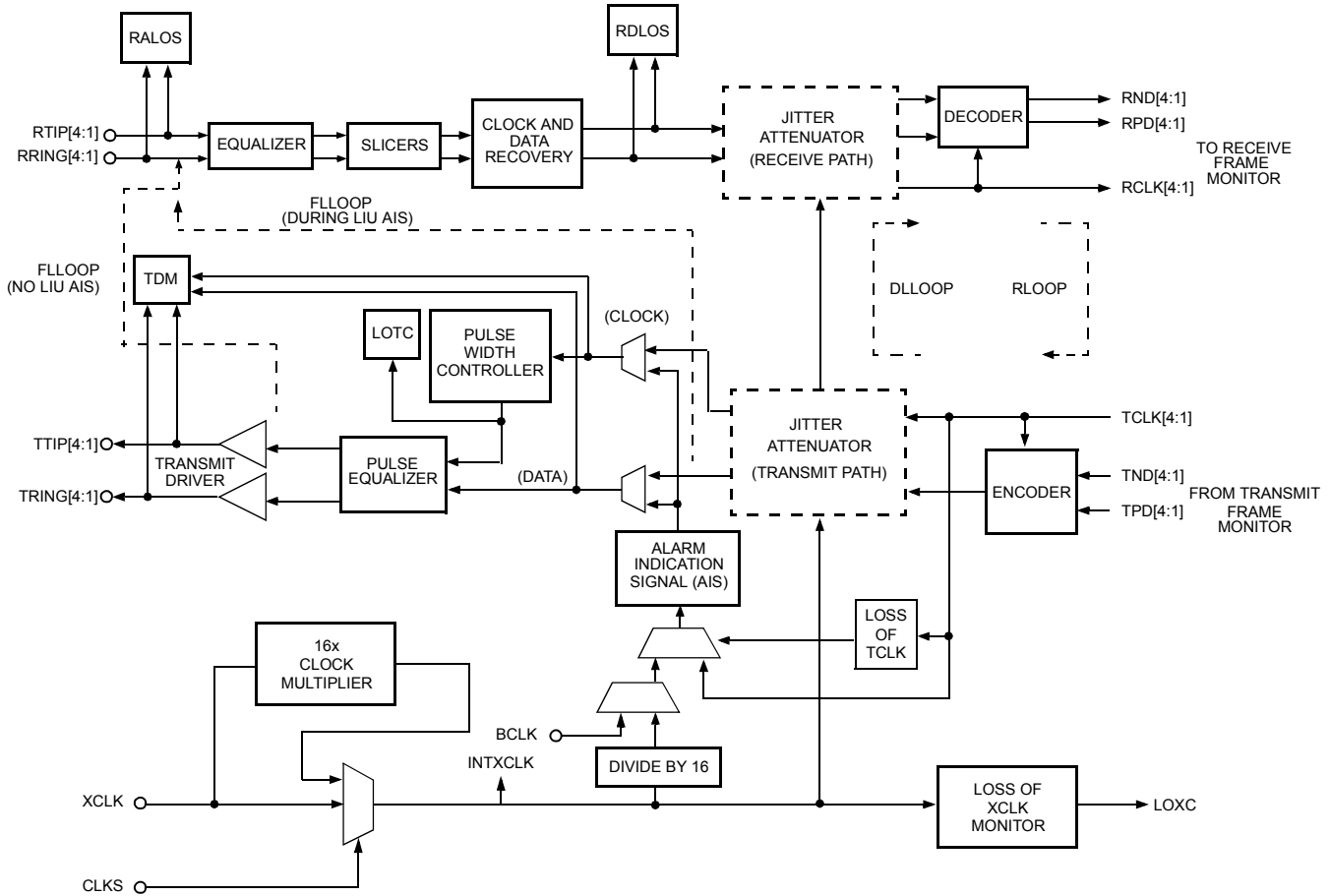
Figure 5. Block Diagram of the Quad Line Interface Unit (Single Channel)
