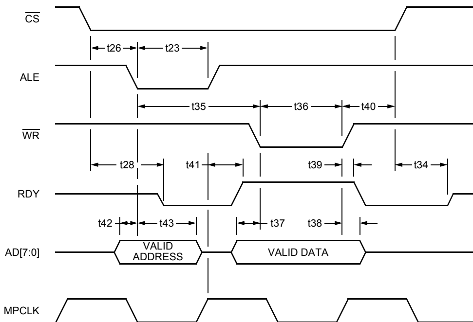
Figure 34. Mode 4—Write Cycle Timing (MPMODE = 1, MPMUX = 1)
