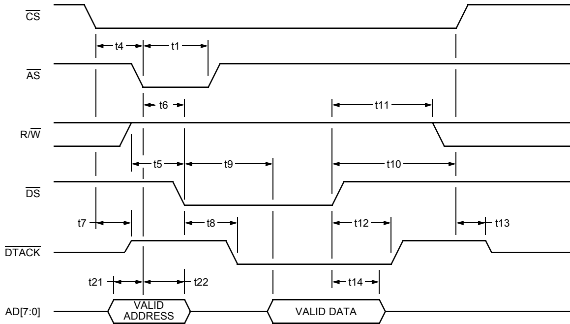
Figure 29. Mode 2—Read Cycle Timing (MPMODE = 0, MPMUX = 1)
