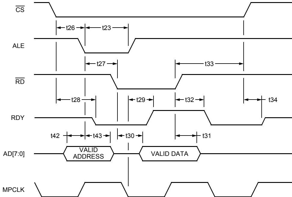
Figure 33. Mode 4—Read Cycle Timing (MPMODE = 1, MPMUX = 1)
