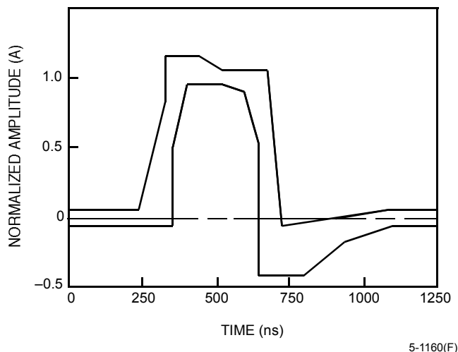
Figure 10. DSX-1 Isolated Pulse Template
