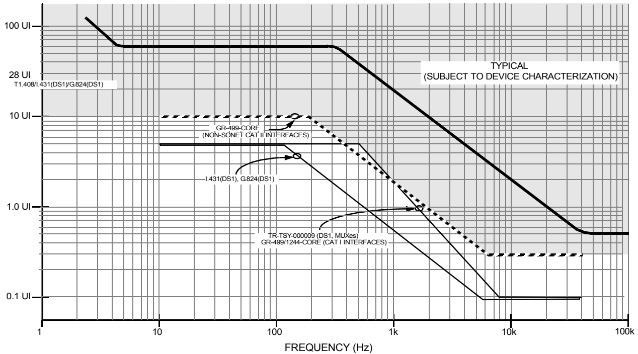
Figure 12. DS1/T1 Receiver Jitter Accommodation with Jitter Attenuator
