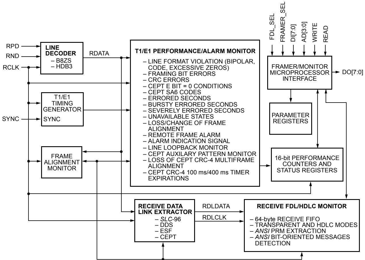
Figure 18. Block Diagram of the Frame Monitor
