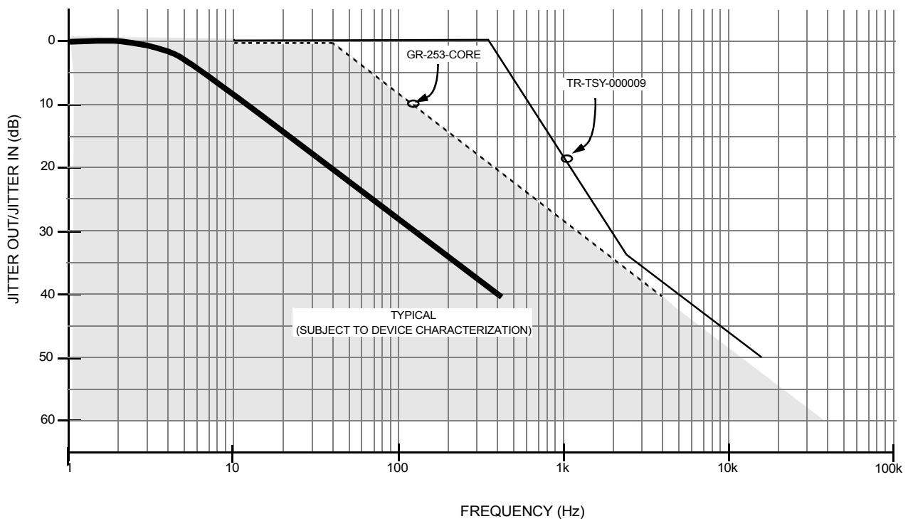
Figure 13. DS1/T1 Jitter Transfer of the Jitter Attenuator
