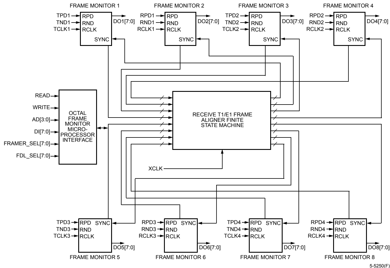
Figure 17. Block Diagram of the Octal Receive Frame Monitor
