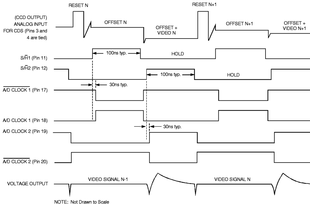
Figure 2. CDS-1402 Typical Timing Diagram
