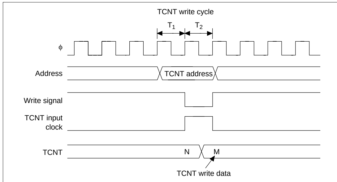
Figure 12.79 TCNT Write and Increment Contention
