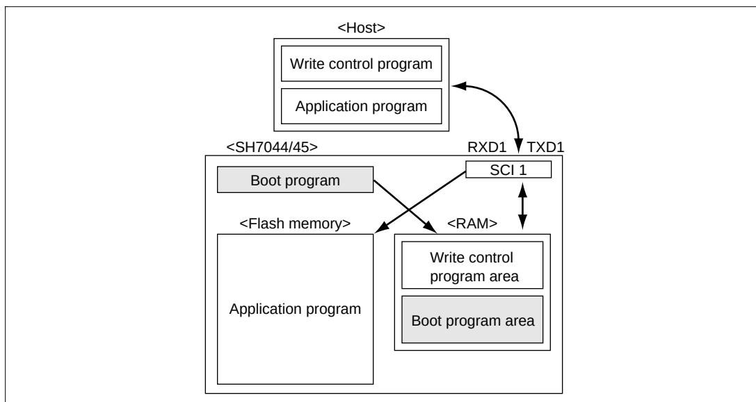
Figure. 1.6 Data transfer during boot mode
