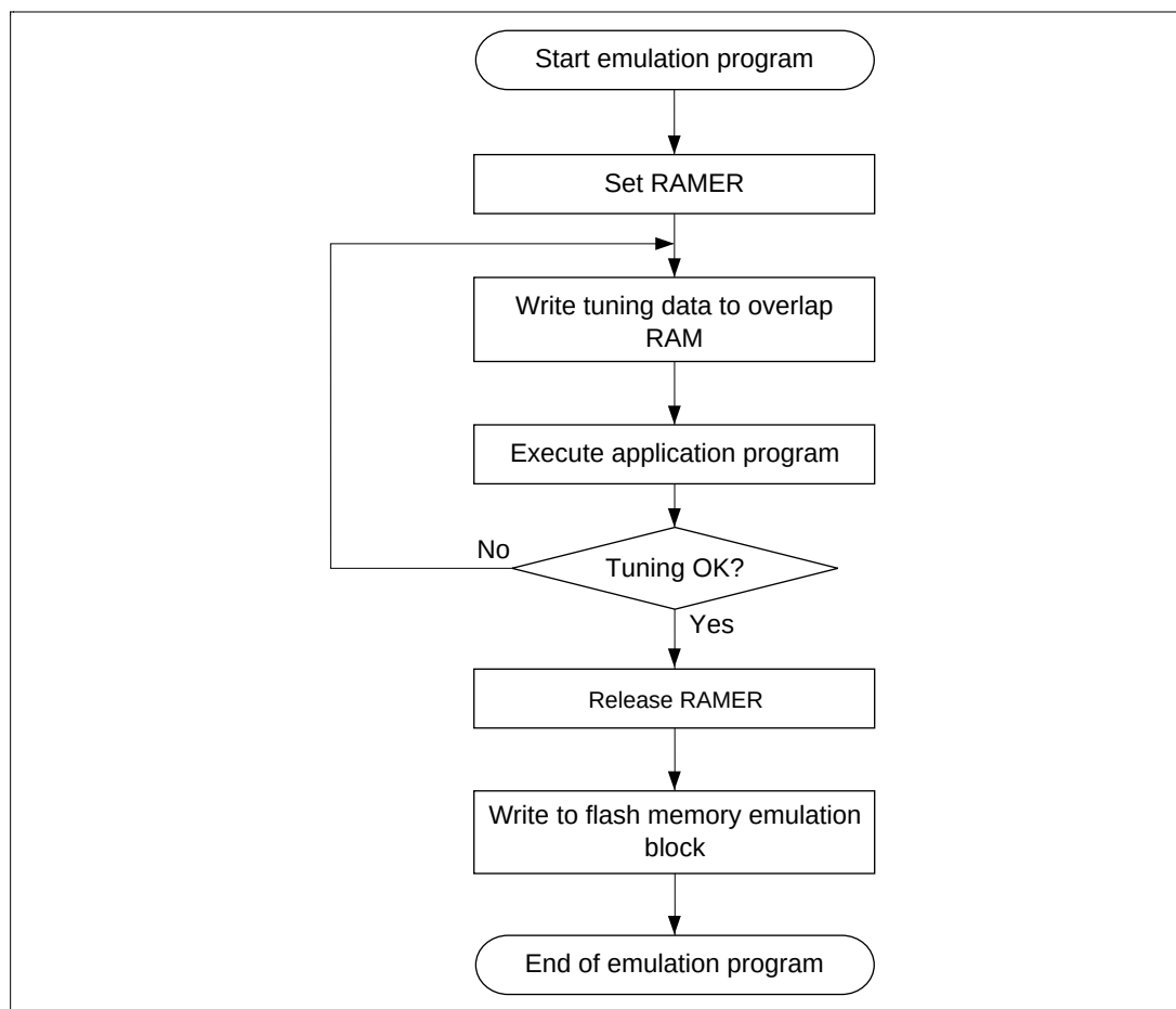
Figure 22.10 Flowchart for Flash Memory Emulation in RAM
