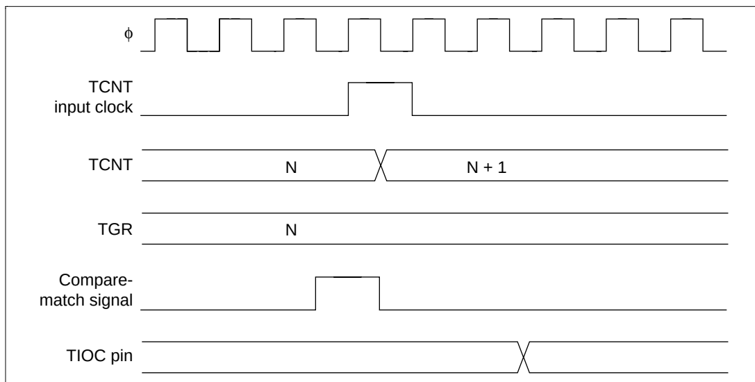
Figure 12.64 Output Compare Output Timing (Complementary PWM Mode/Reset Sync PWM Mode)
