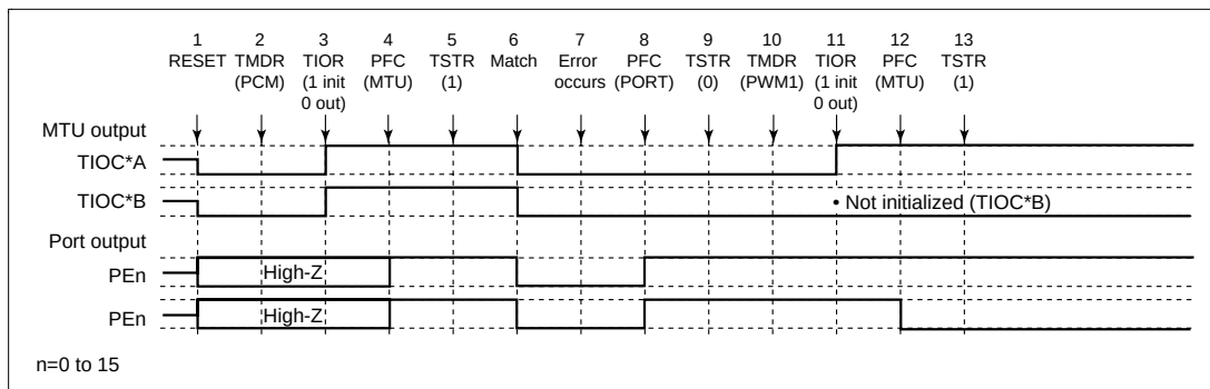
Figure 12.114 Error Occurrence in Phase Counting Mode, Recovery in PWM Mode 1
