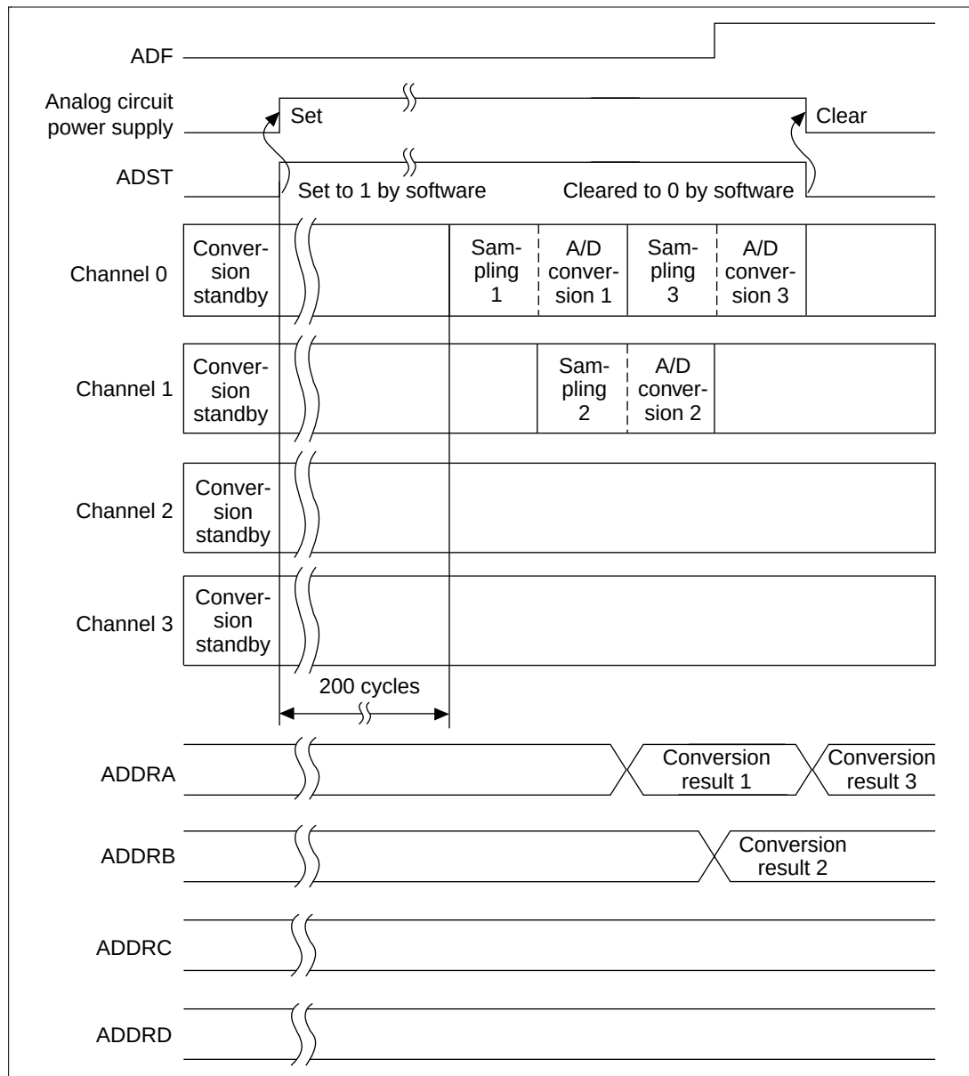
Figure 15.9 Conversion Start Operation (Low-Power Conversion Mode)
