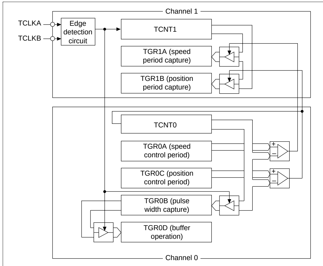
Figure 12.35 Phase Count Mode Application Example
