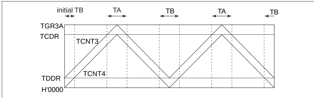
Figure. 12.96 Temporary Register Comparison Execution Time
