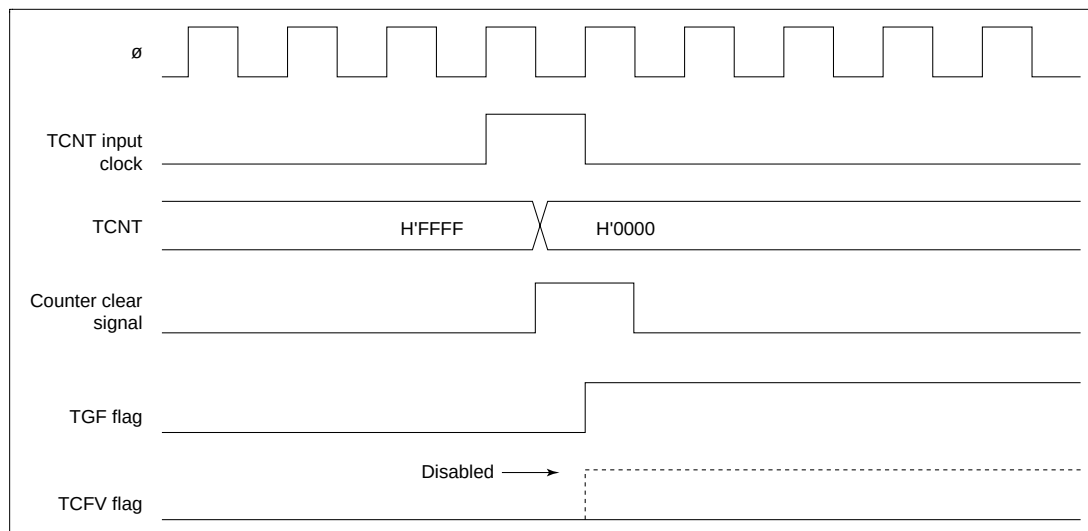
Figure 12.94 Contention between Overflow and Counter Clearing
