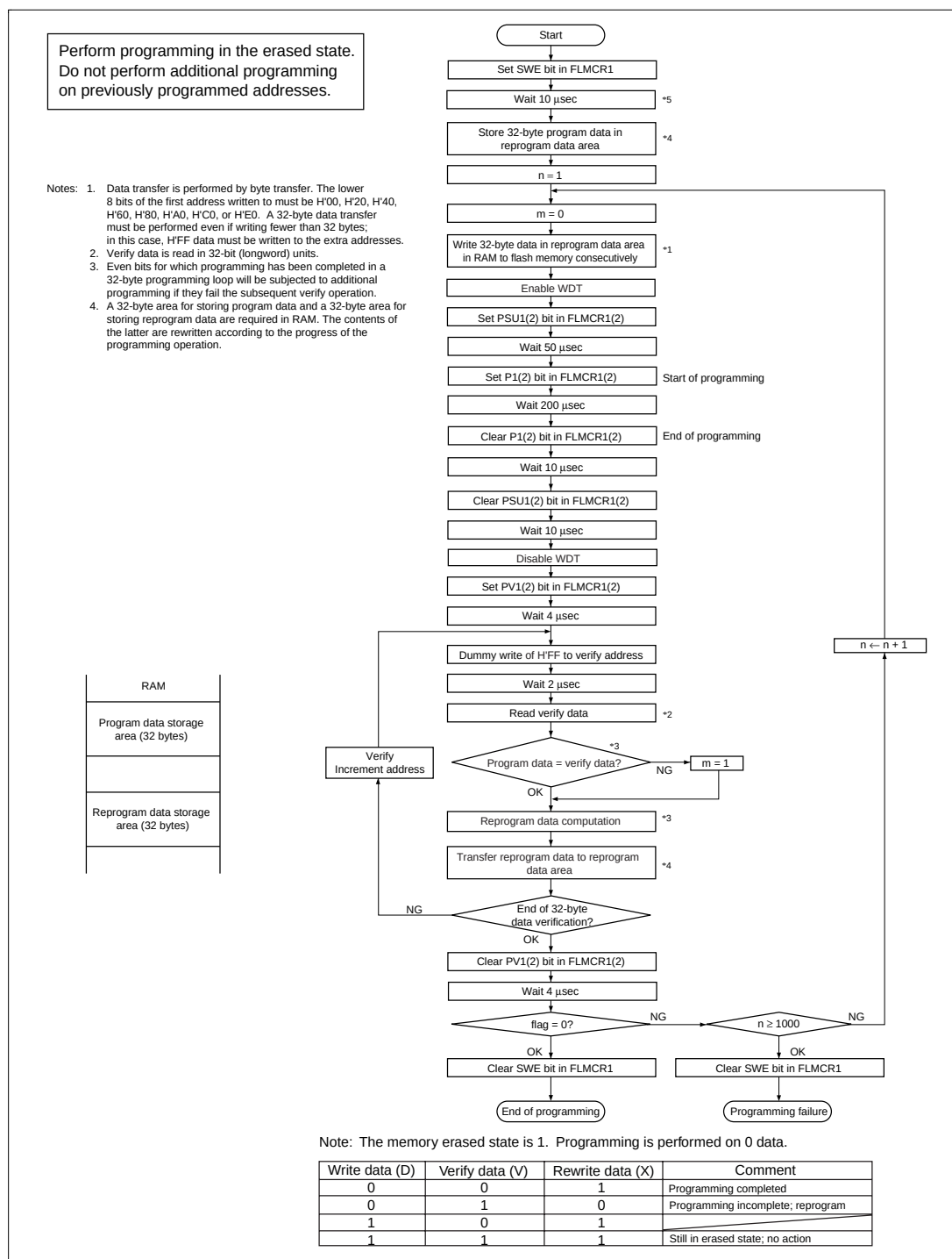
Figure 22.7 Program/Program Verify Flow
