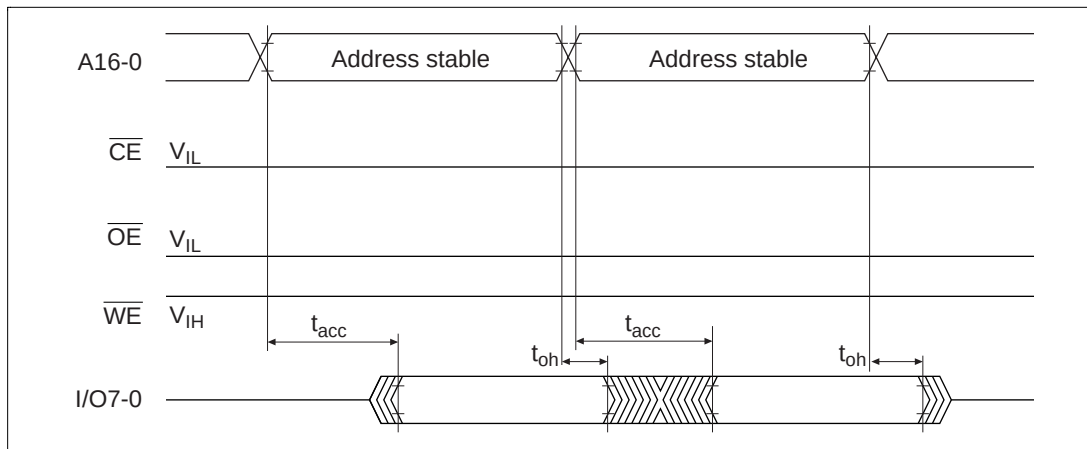
Figure 22.17 \overline{CE} and \overline{OE} Enable State Read Timing Waveforms
