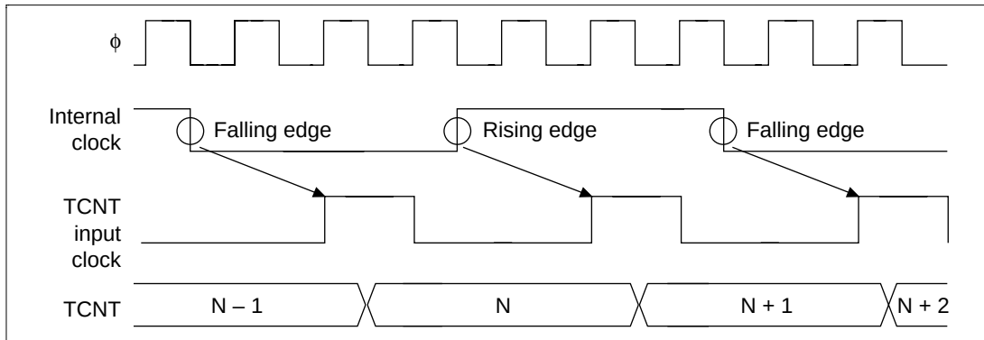
Figure 12.60 TCNT Count Timing during Internal Clock Operation
