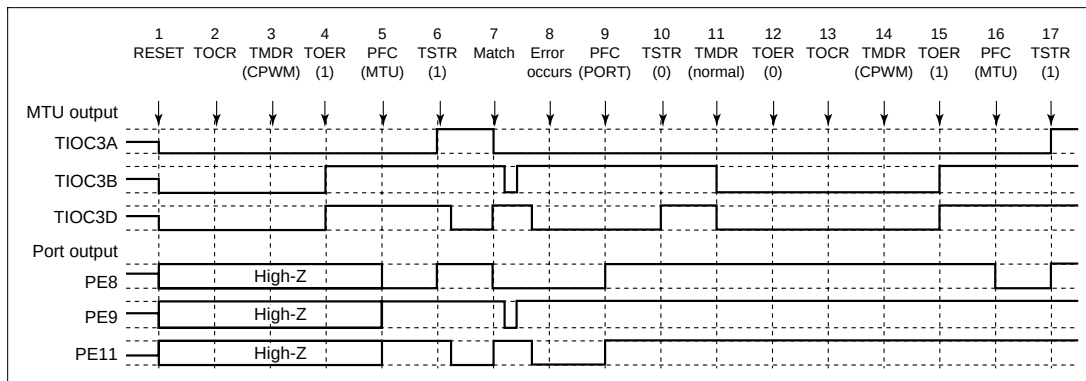
Figure 12.120 Error Occurrence in Complementary PWM Mode, Recovery in Complementary PWM Mode
