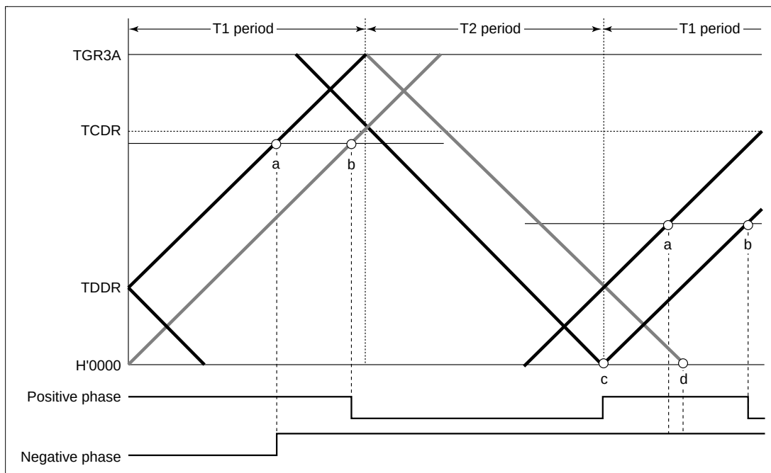
Figure 12.50 Example of Complementary PWM Mode 0% and 100% Waveform Output (2)
