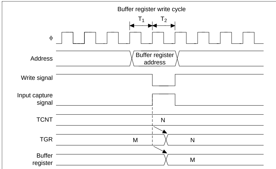
Figure 12.84 Buffer Register Write and Input Capture Contention
