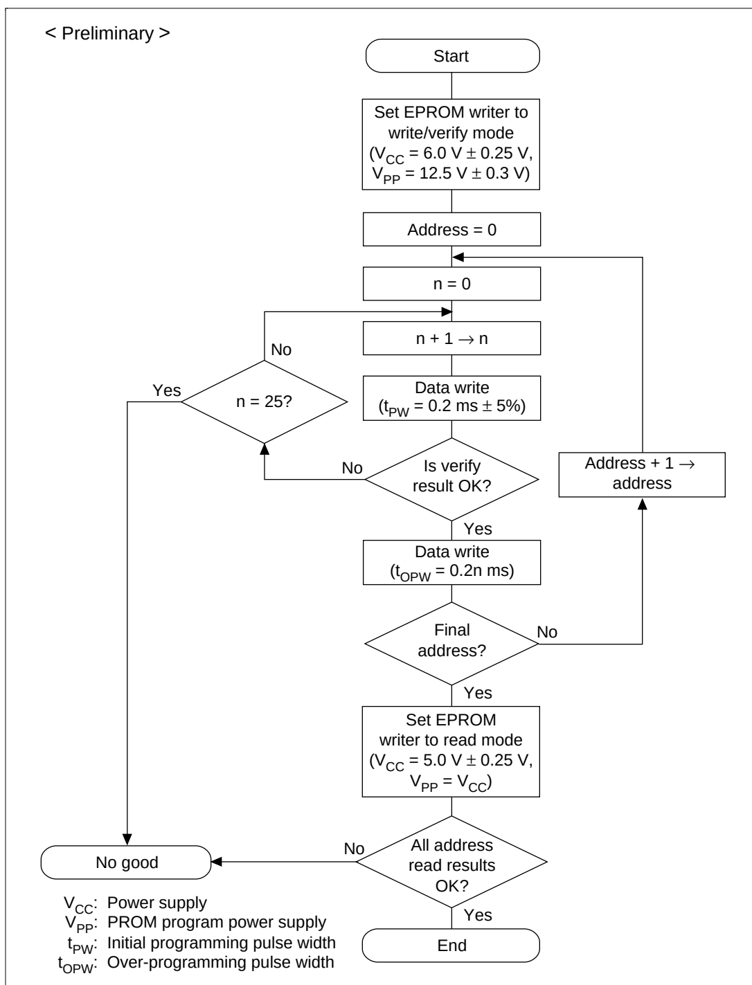
Figure 21.5 High-Speed, High-Reliability Programming Basic Flow
