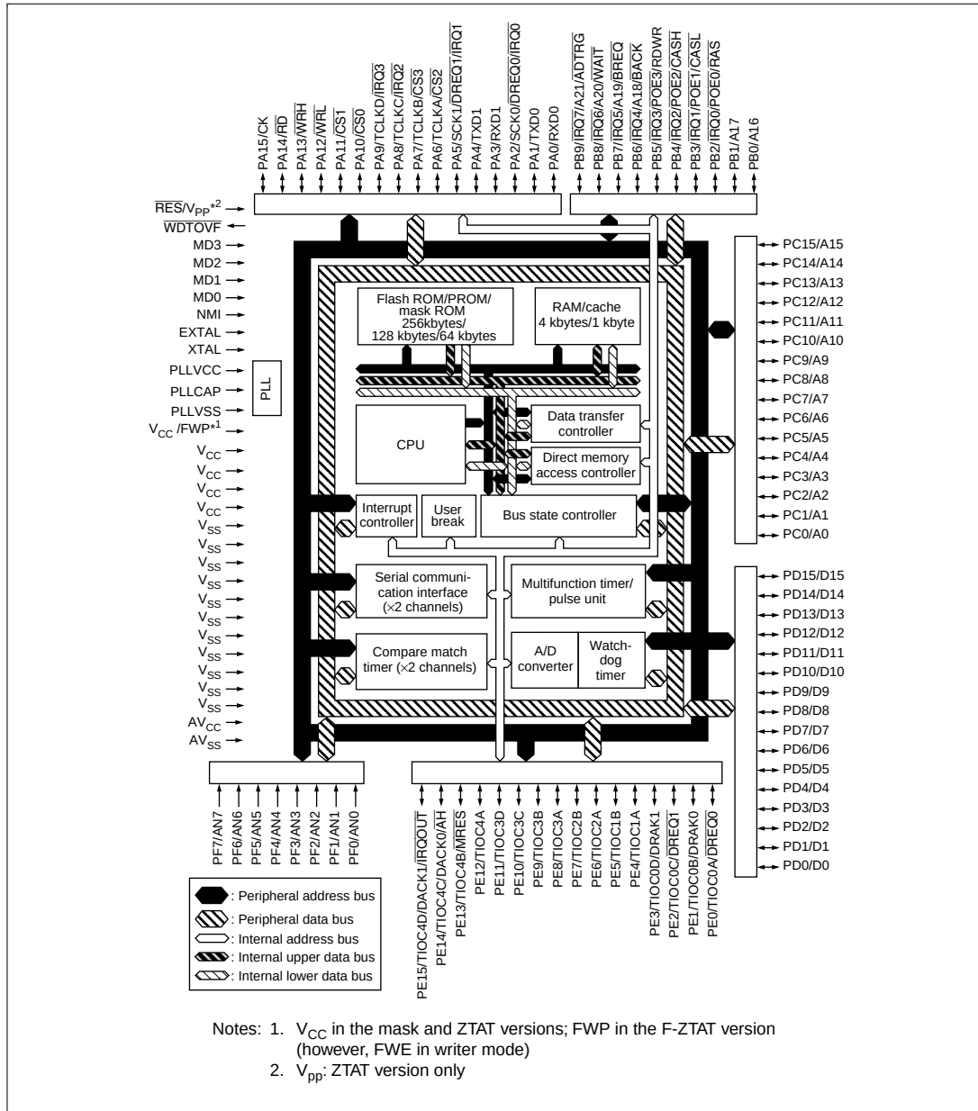
Figure 1.1 Block Diagram of the SH7040, SH7042, SH7044 (QFP-112 Pin)
