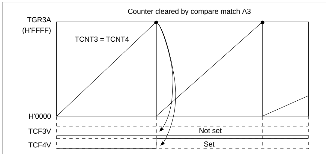
Figure 12.90 Reset Sync PWM Mode Overflow Flag
