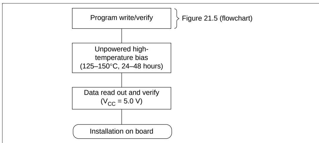
Figure 21.7 Screening Flow
