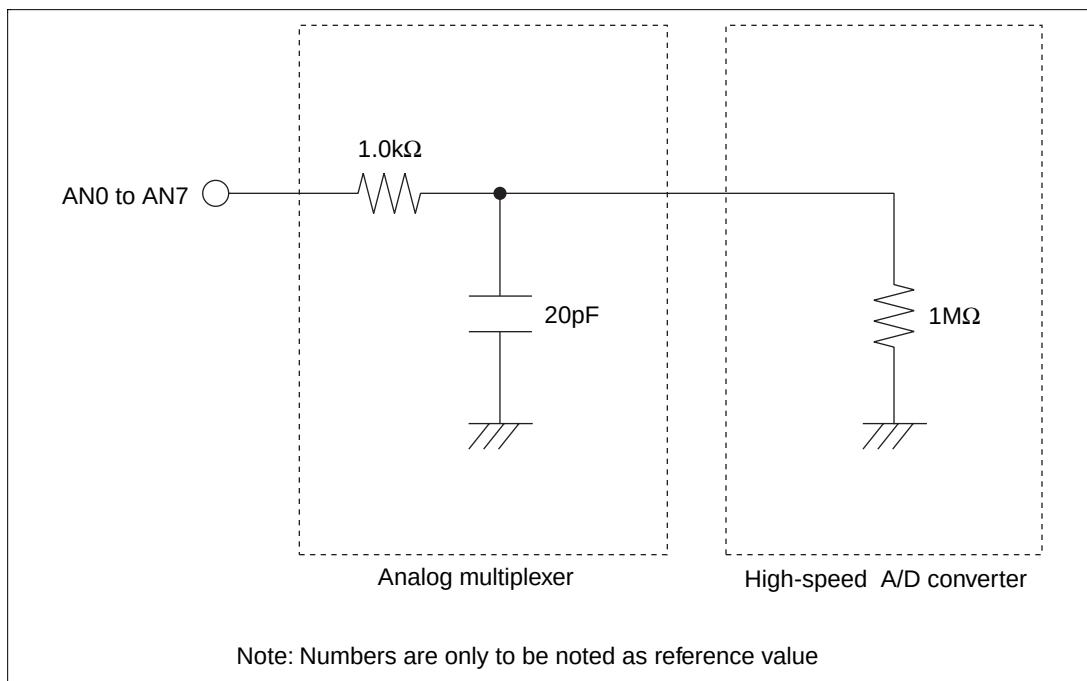
Figure 15.14 Equivalent Circuit of Analog Input Pins
