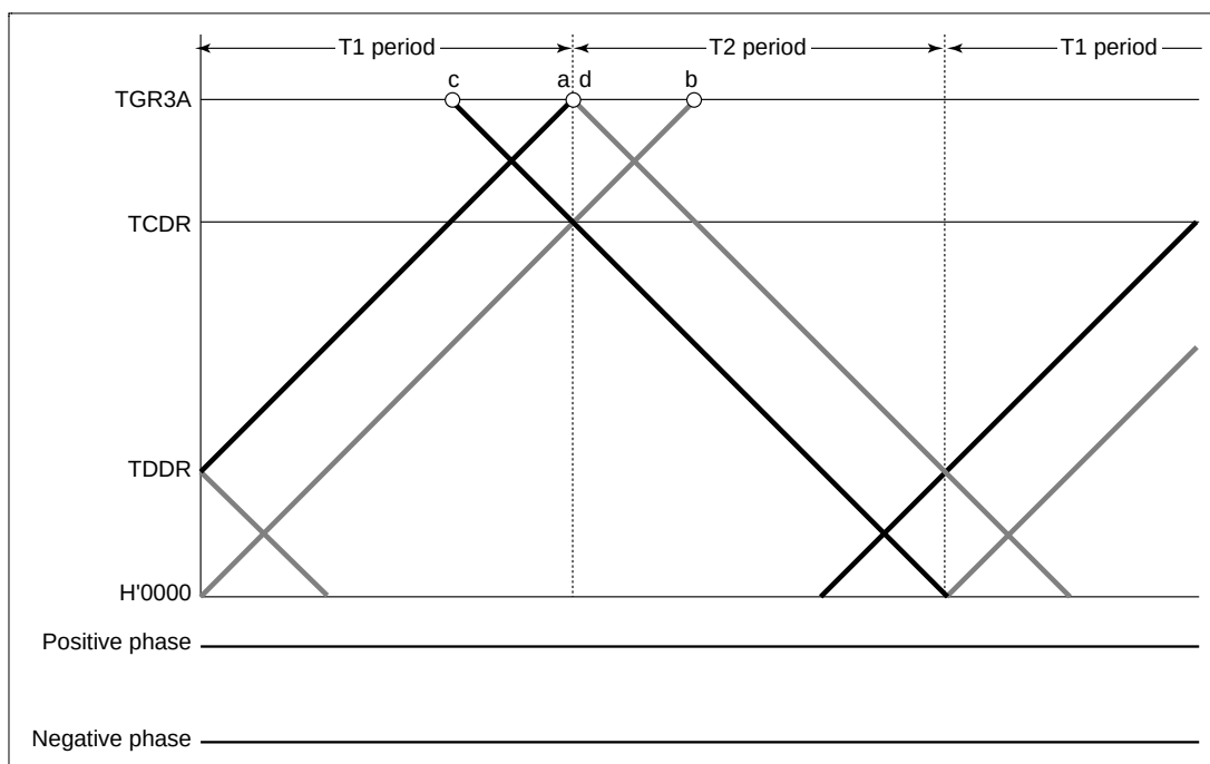
Figure 12.53 Example of Complementary PWM Mode 0% and 100% Waveform Output (5)
