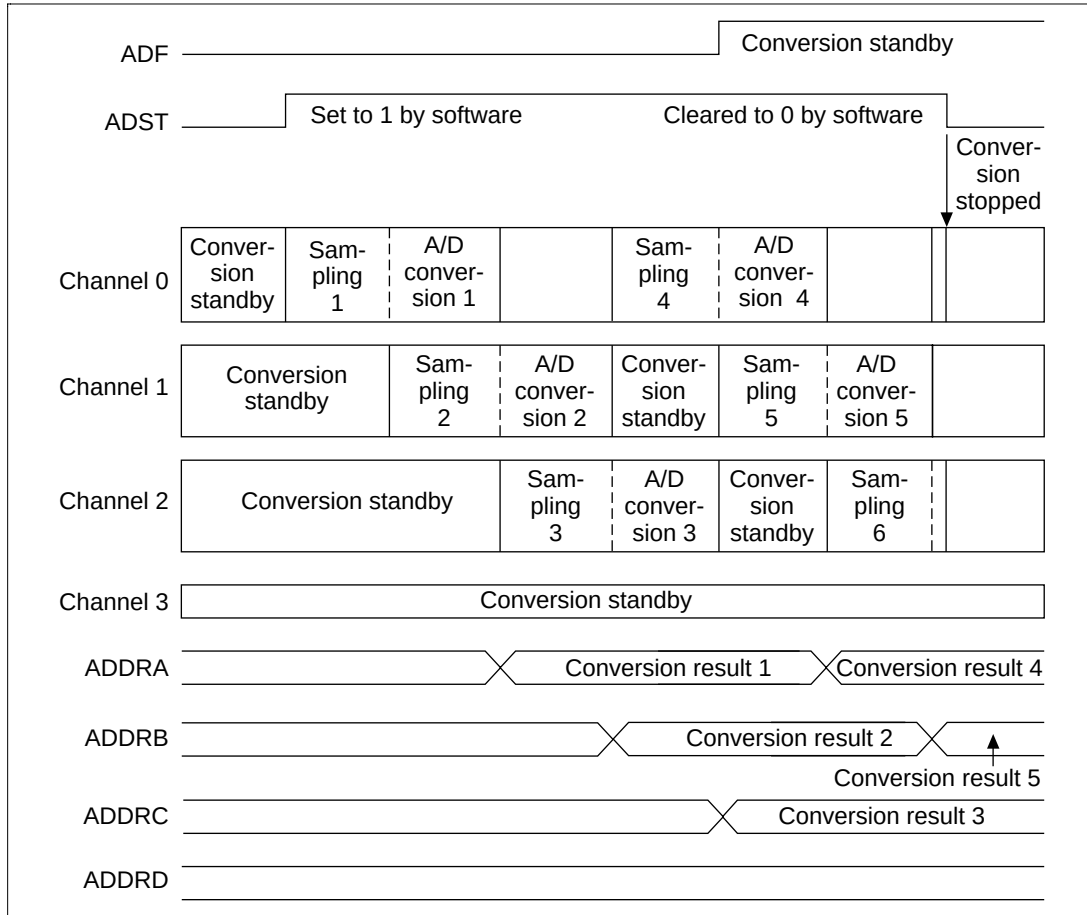
Figure 15.6 A/D Converter Operation Example (Group-Scan Mode)
