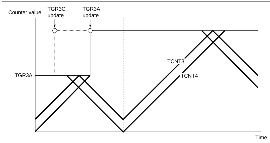
Figure 12.42 Example of PWM Cycle Updating
