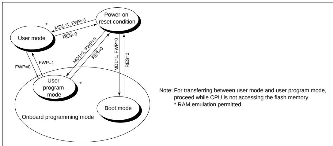
Figure 1.5 Condition Transfer for Flash Memory
