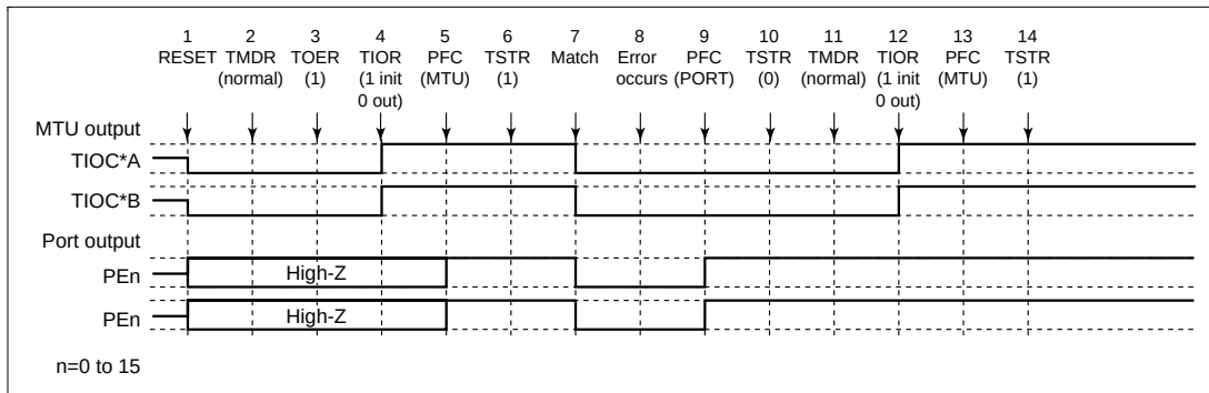
Figure 12.97 Error Occurrence in Normal Mode, Recovery in Normal Mode
