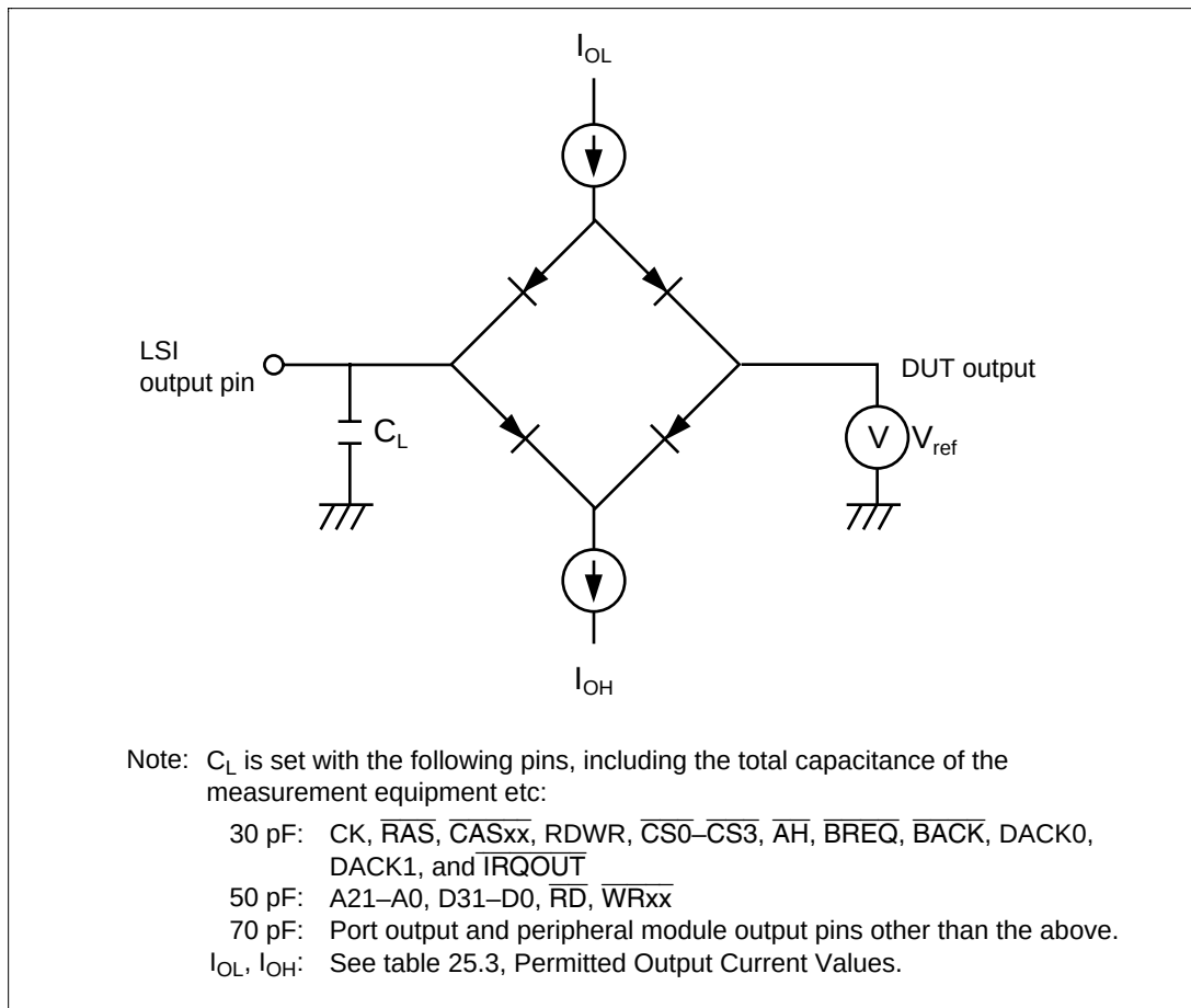
Figure 25.31 Output Test Circuit
