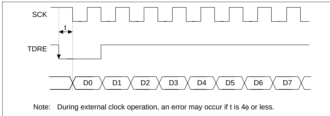
Figure 14.24 Example of Clock Synchronous Transmission with DMAC
