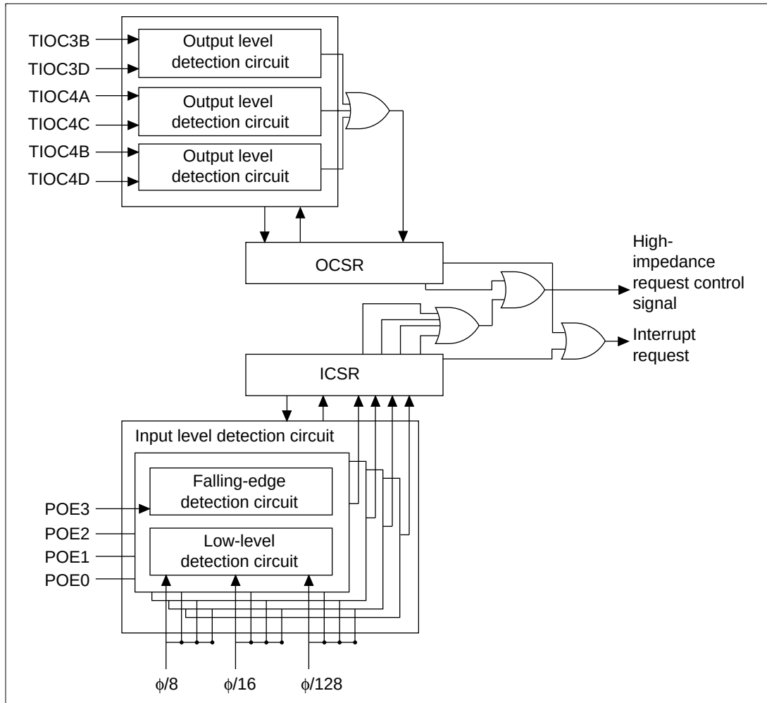
Figure 12.126 POE Block Diagram
