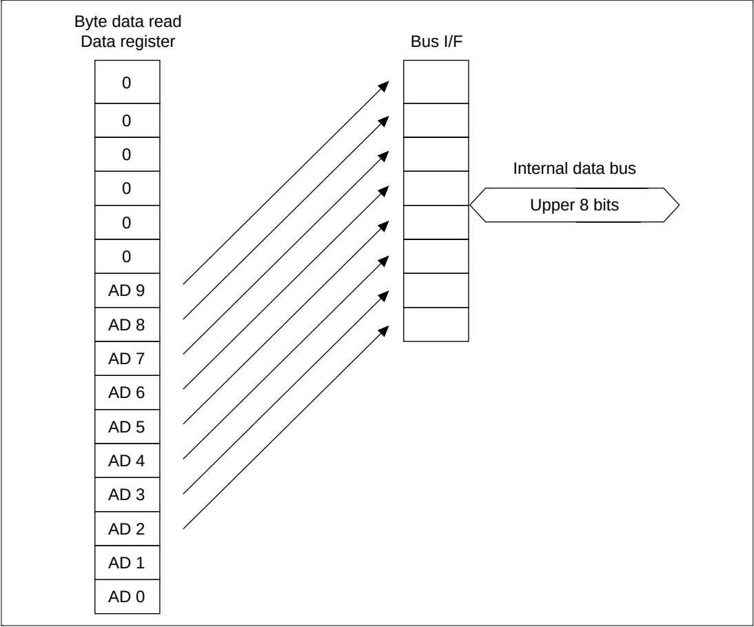
Figure 15.2 ADDR Read Operation (cont)
