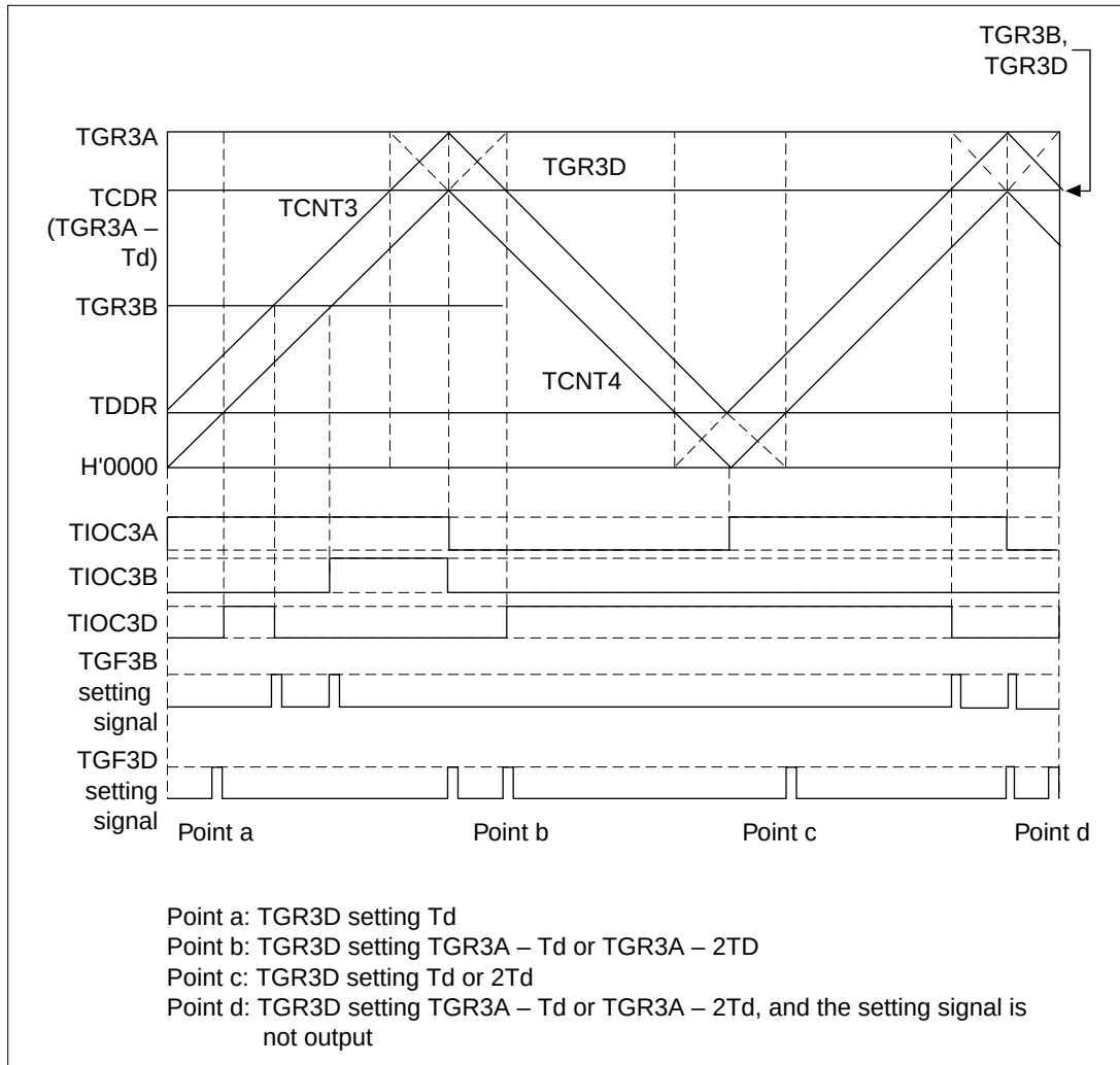
Figure 12.92 Special Properties of Compare Match Flag in Complementary PWM Mode
