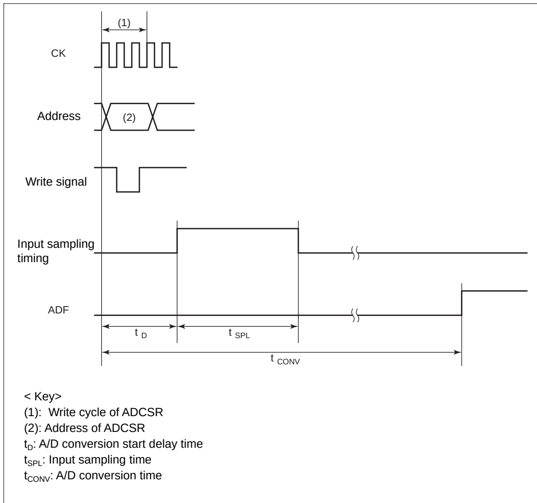
Figure 16.5 A/D Conversion Timing
