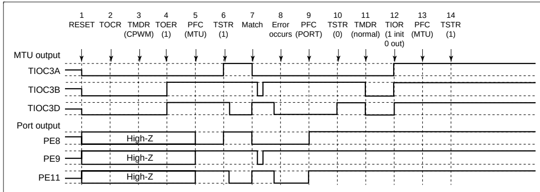
Figure 12.117 Error Occurrence in Complementary PWM Mode, Recovery in Normal Mode
