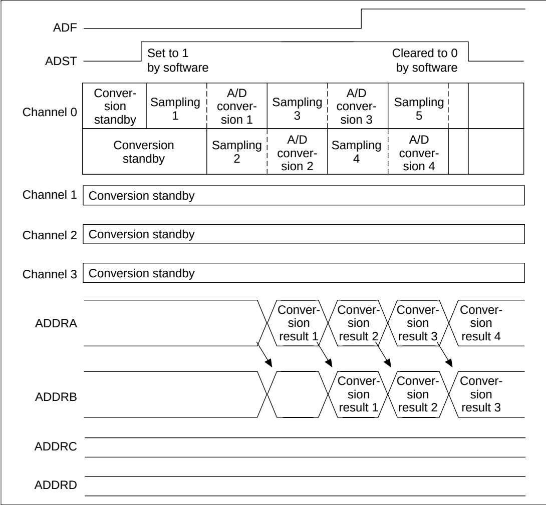
Figure 15.7 Buffer Operation Example (Select Scan Mode: Two-Stage One-Group Operation, When CH2-CH0 = B'001)
