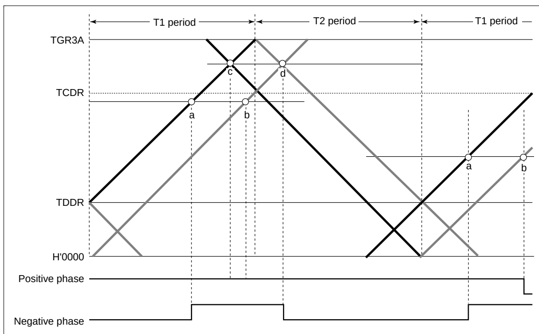
Figure 12.47 Example of Complementary PWM Mode Waveform Output (2)
