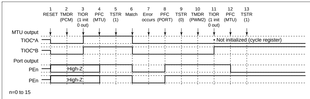
Figure 12.115 Error Occurrence in Phase Counting Mode, Recovery in PWM Mode 2
