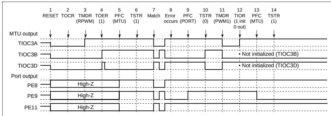
Figure 12.123 Error Occurrence in Reset-Synchronous PWM Mode, Recovery in PWM Mode 1
