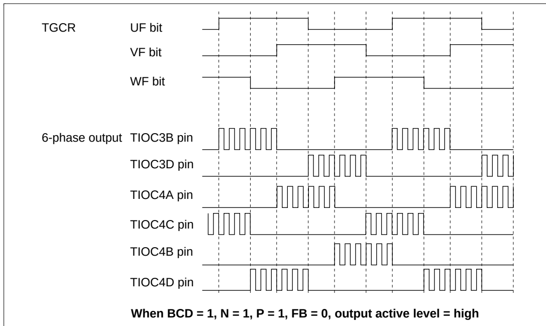
Figure 12.59 Example of Output Phase Switching by Means of UF, VF, WF Bit Settings (2)
