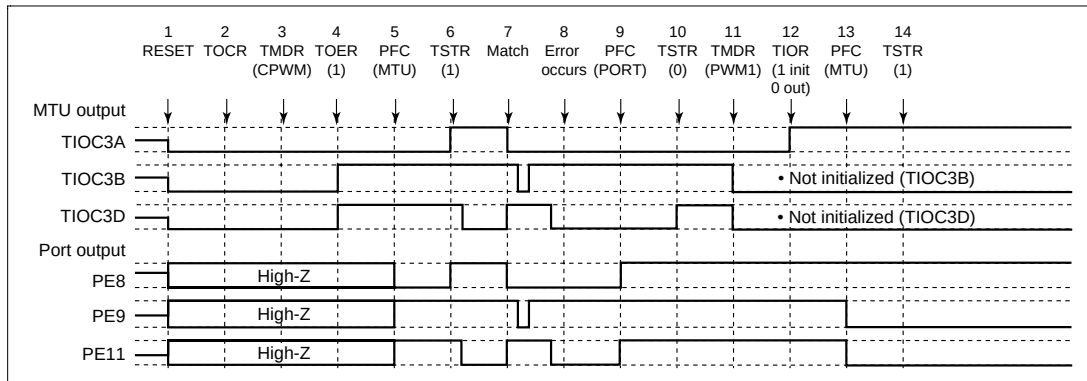
Figure 12.118 Error Occurrence in Complementary PWM Mode, Recovery in PWM Mode 1
