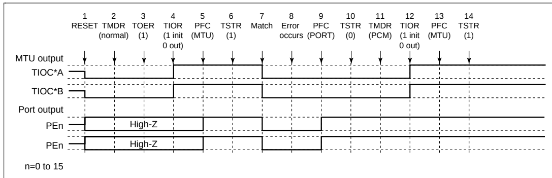
Figure 12.100 Error Occurrence in Normal Mode, Recovery in Phase Counting Mode
