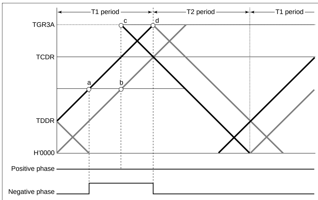
Figure 12.51 Example of Complementary PWM Mode 0% and 100% Waveform Output (3)
