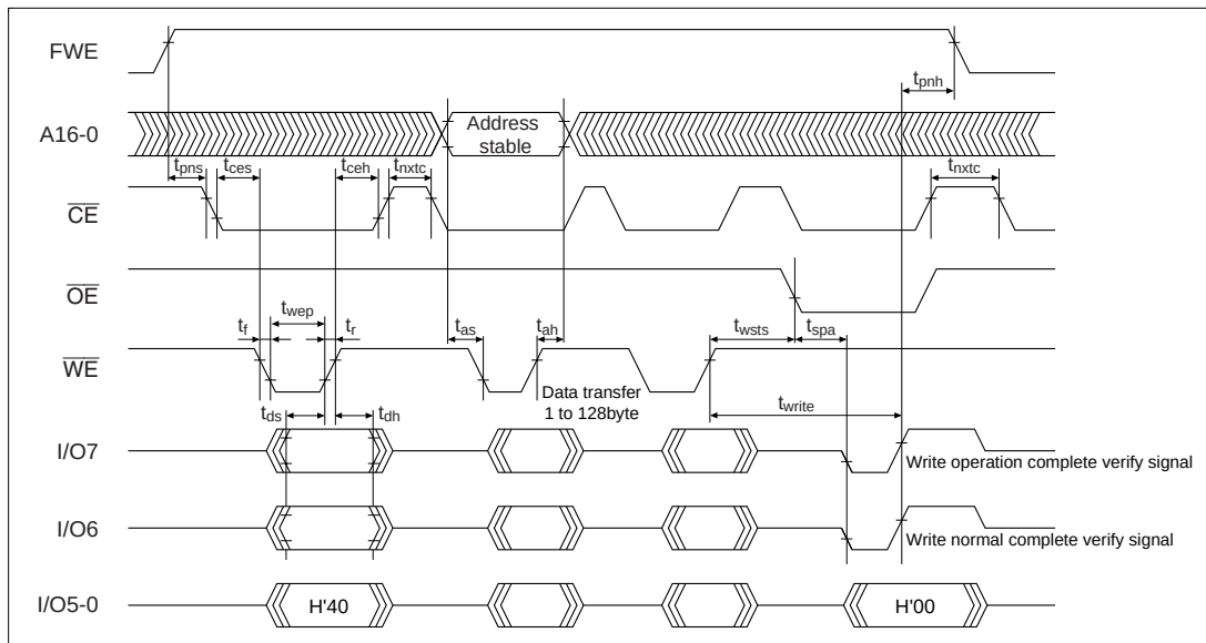
Figure 22.19 Auto-Program Mode Timing Waveforms
