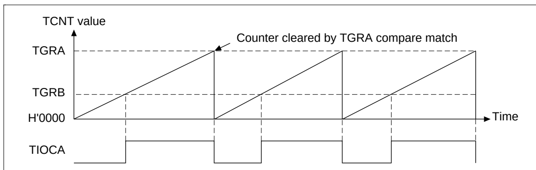
Figure 12.26 PWM Mode Operation Example (Mode 1)
