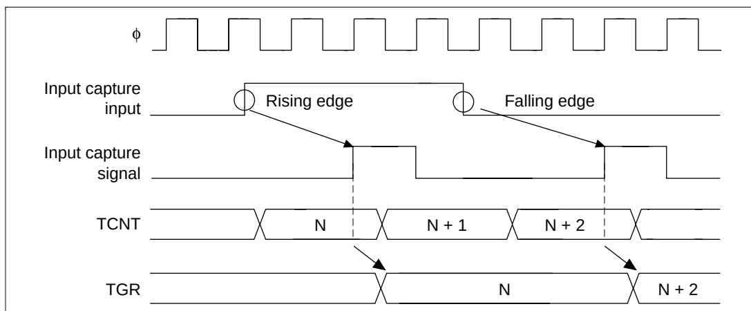
Figure 12.65 Input Capture Input Signal Timing
