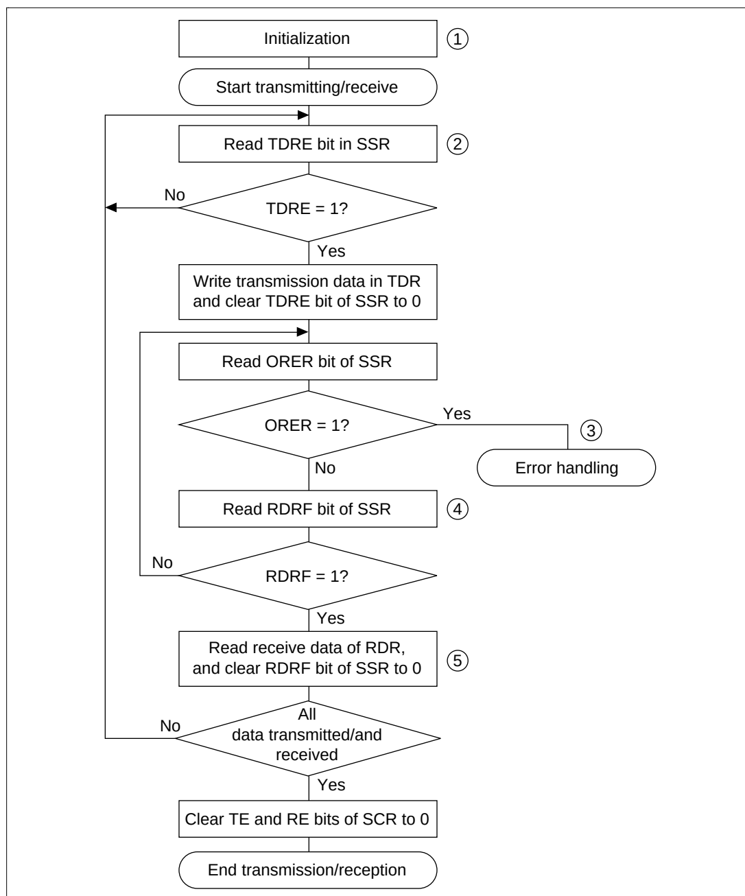
Figure 14.22 Sample Flowchart for Serial Transmission
