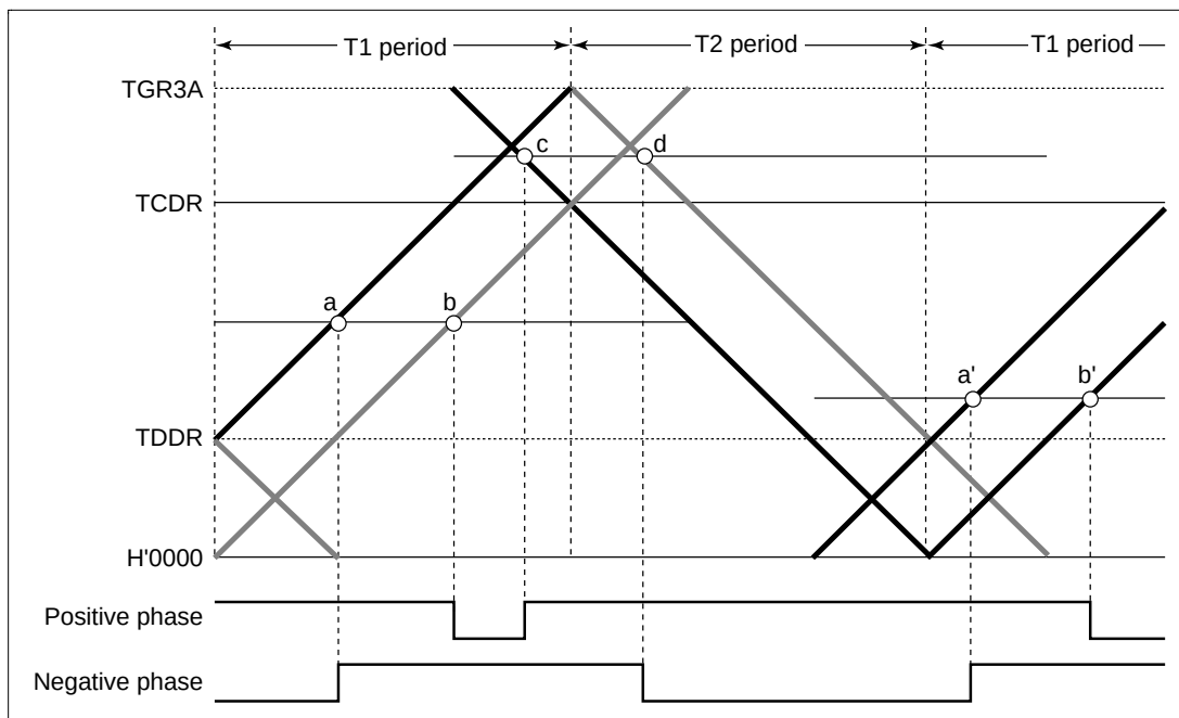
Figure 12.46 Example of Complementary PWM Mode Waveform Output (1)
