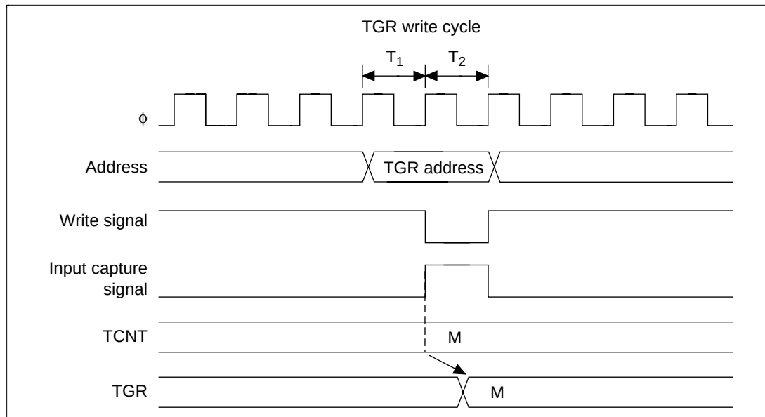
Figure 12.83 TGR Write and Input Capture Contention
