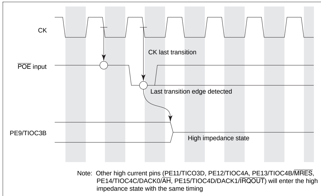
Figure 12.129 Last Transition Edge Detection Operation
