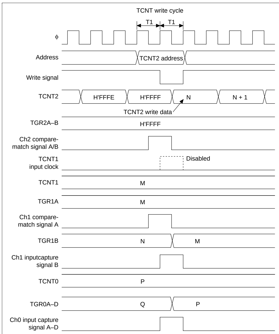
Figure 12.86 TCNT2 Write and Overflow/Underflow Contention with Cascade Connection
