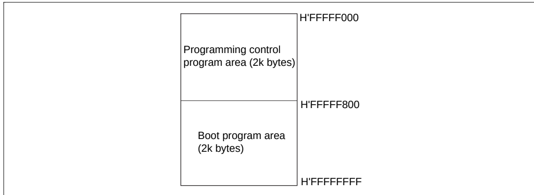
Figure 22.5 RAM Areas in Boot Mode
