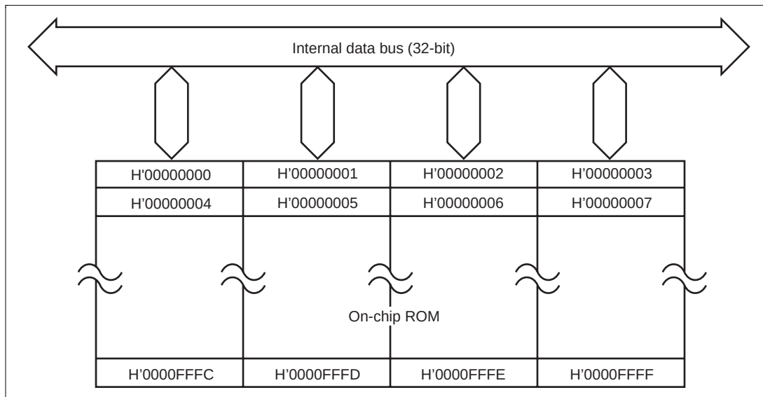
Figure 20.1 Mask ROM Block Diagram (64kbyte version)
