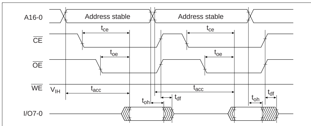
Figure 22.18 \overline{CE} and \overline{OE} Clock System Read Timing Waveforms
