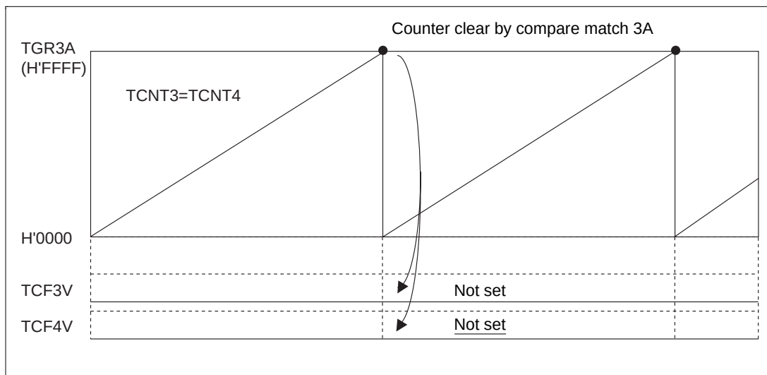
Figure. 12.91 Reset Sync PWM Mode Overflow Flag (for A Mask)
