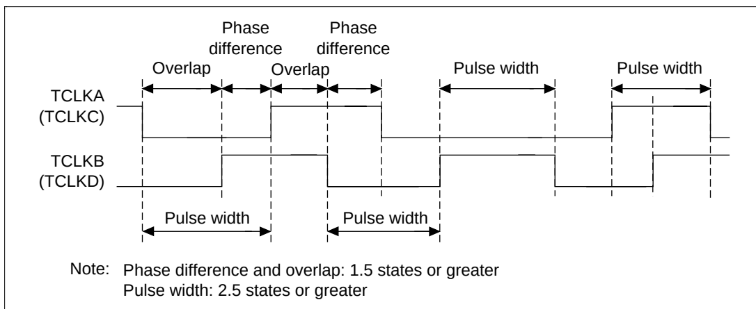
Figure 12.77 Phase Difference, Overlap, and Pulse Width in Phase Count Mode
