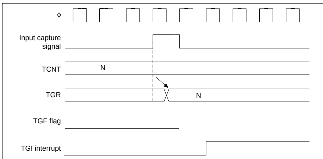
Figure 12.71 TGI Interrupt Timing (Input Capture)
