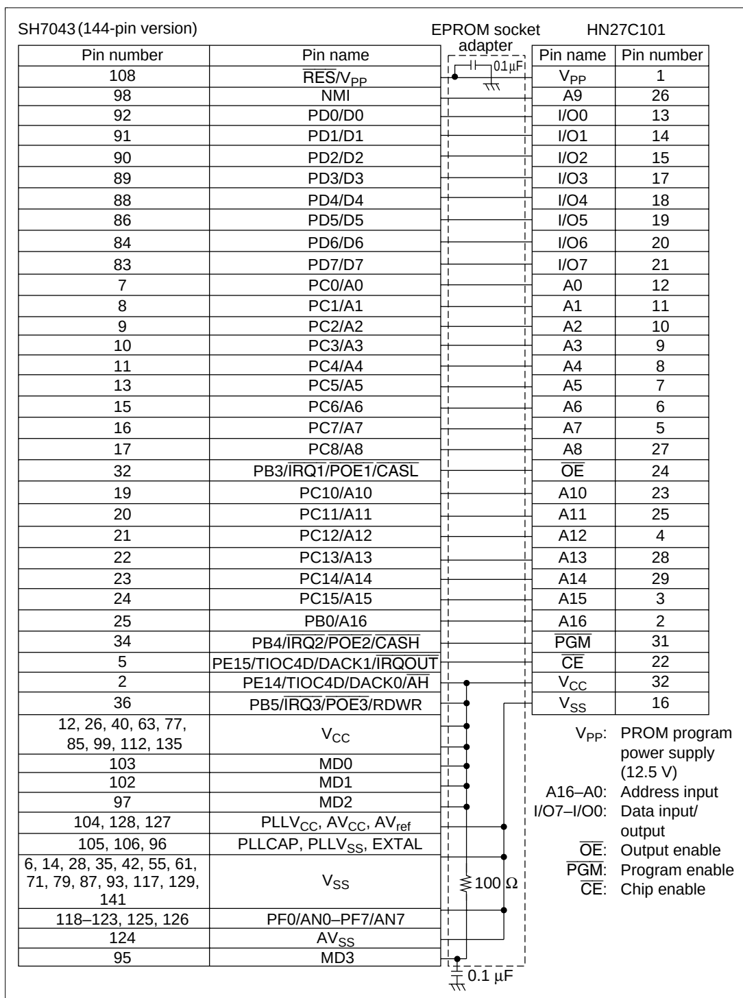
Figure 21.3 SH7043 Pin and HN27C101 Pin Correspondence (144-Pin Version)
