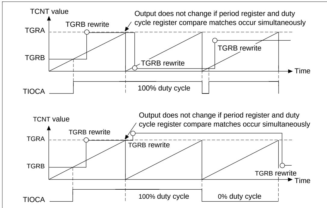
Figure 12.29 PWM Mode Operation Example (100% Duty Cycle)
