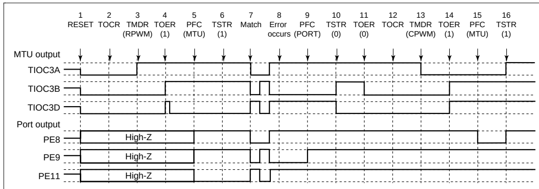
Figure 12.124 Error Occurrence in Reset-Synchronous PWM Mode, Recovery in Complementary PWM Mode
