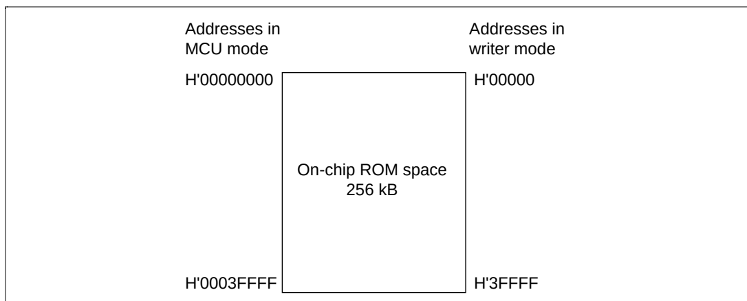
Figure 22.12 On-Chip ROM Memory Map
