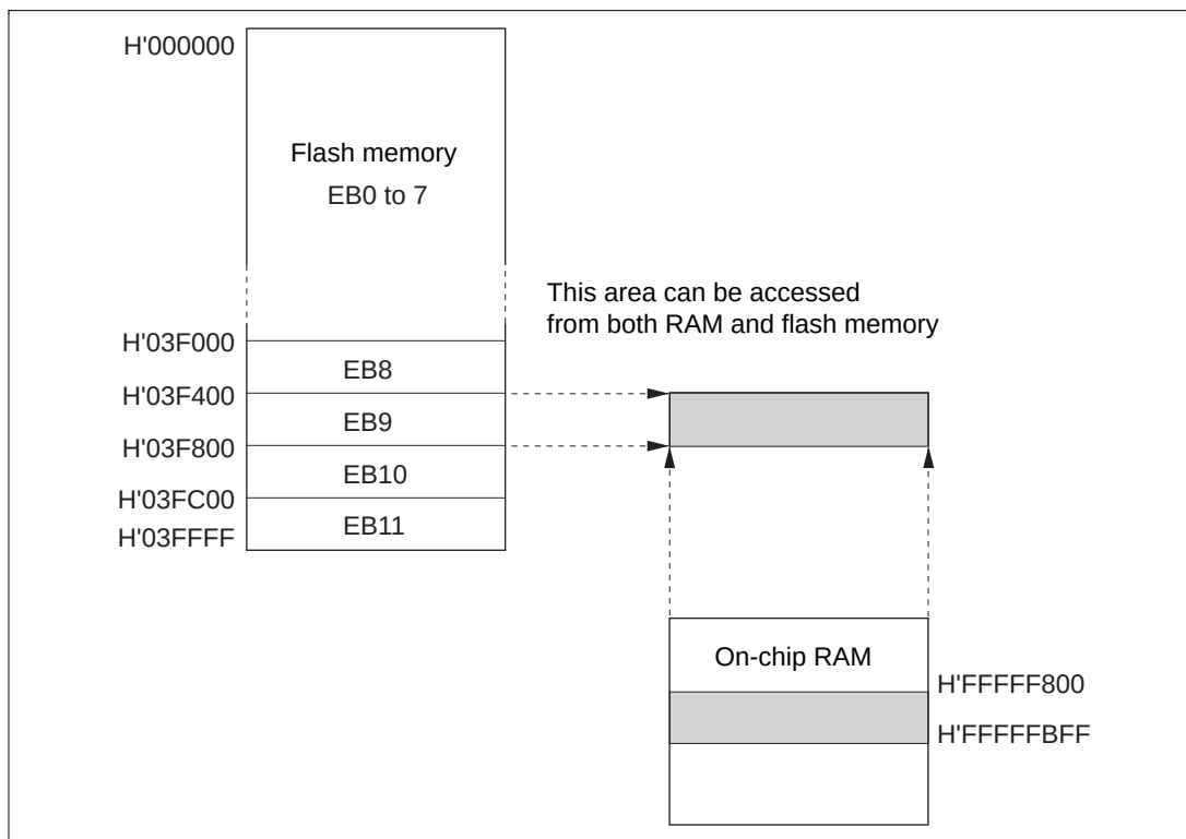
Figure 22.11 Example of RAM Overlap Operation
