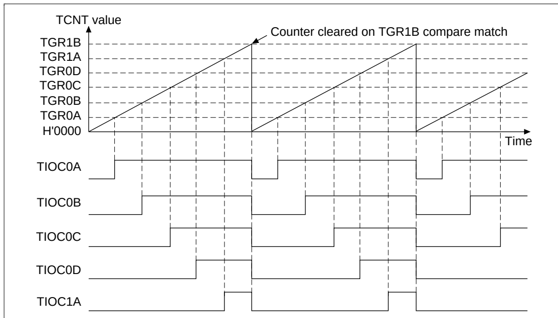
Figure 12.27 PWM Mode Operation Example (Mode 2)
