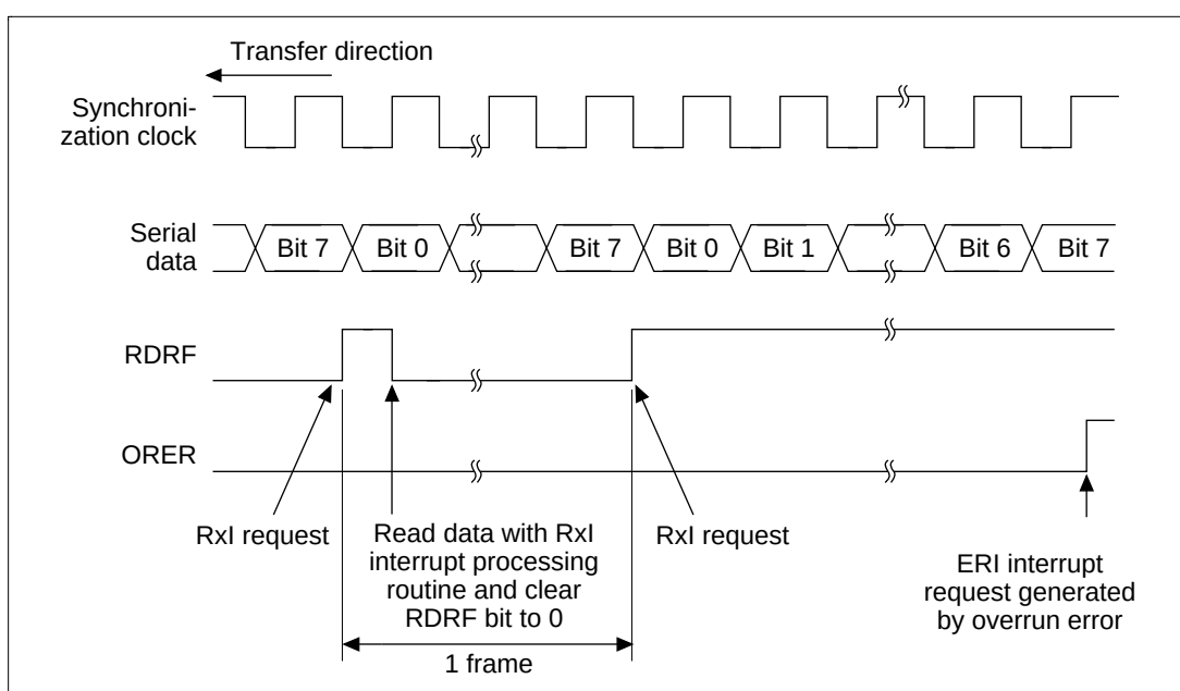
Figure 14.21 Example of SCI Receive Operation
