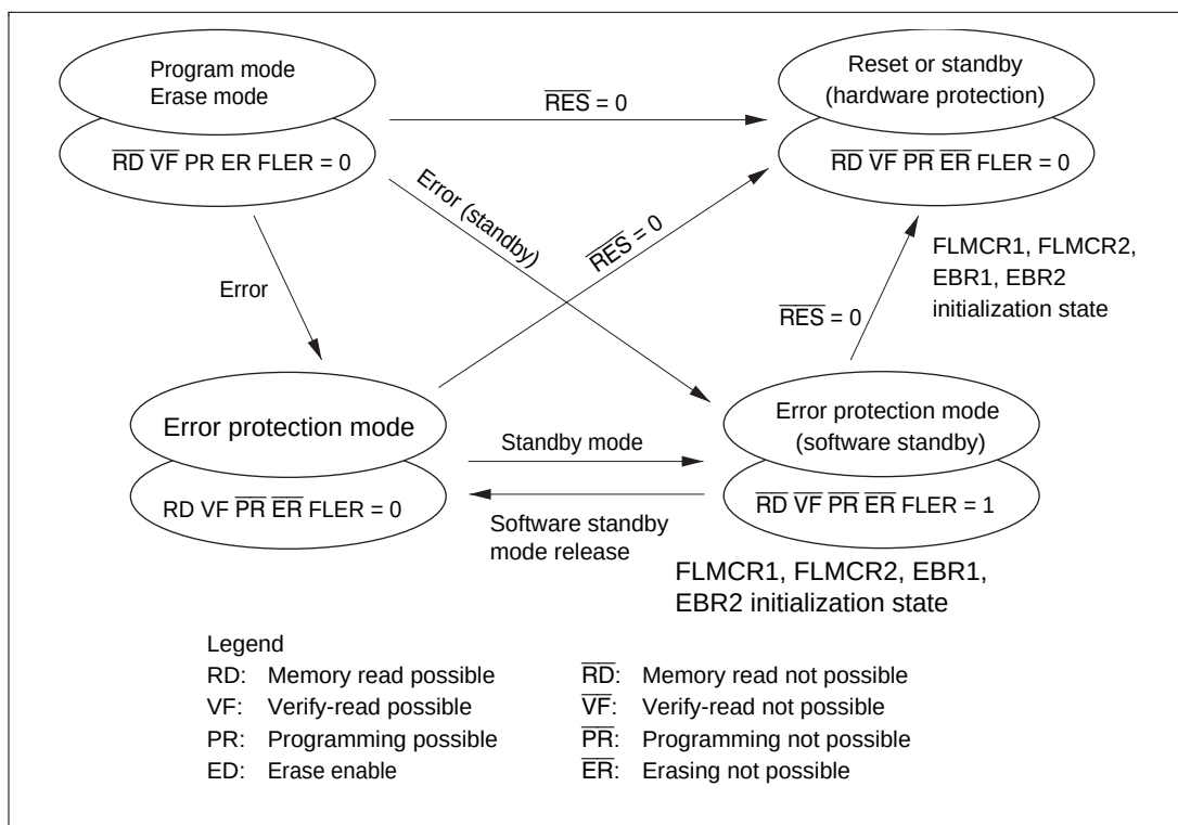
Figure 22.9 Flash Memory State Transitions
