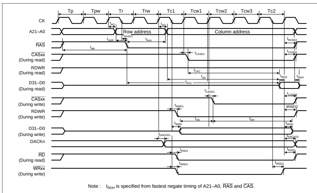
Figure 25.14 DRAM Cycle (Normal Mode, 3 Waits, TPC = 1, RCD = 1)
