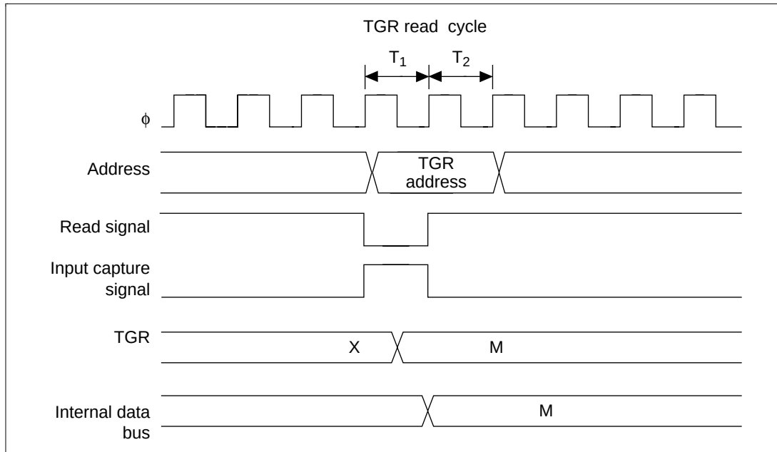
Figure 12.82 TGR Read and Input Capture Contention
