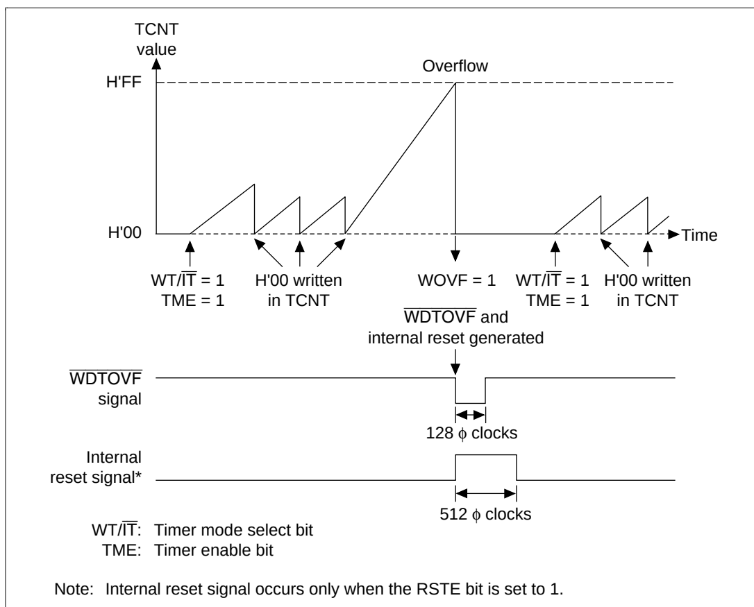
Figure 13.4 Operation in the Watchdog Timer Mode
