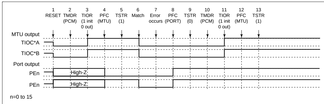
Figure 12.116 Error Occurrence in Phase Counting Mode, Recovery in Phase Counting Mode
