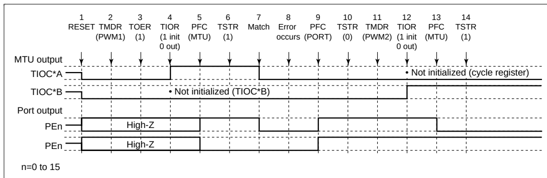
Figure 12.105 Error Occurrence in PWM Mode 1, Recovery in PWM Mode 2
