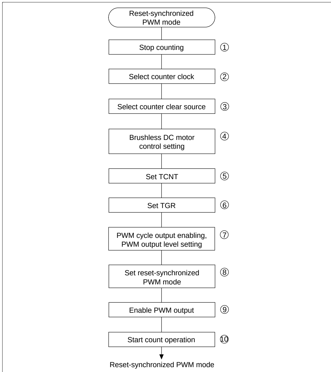
Figure 12.36 Procedure for Selecting the Reset-Synchronized PWM Mode
