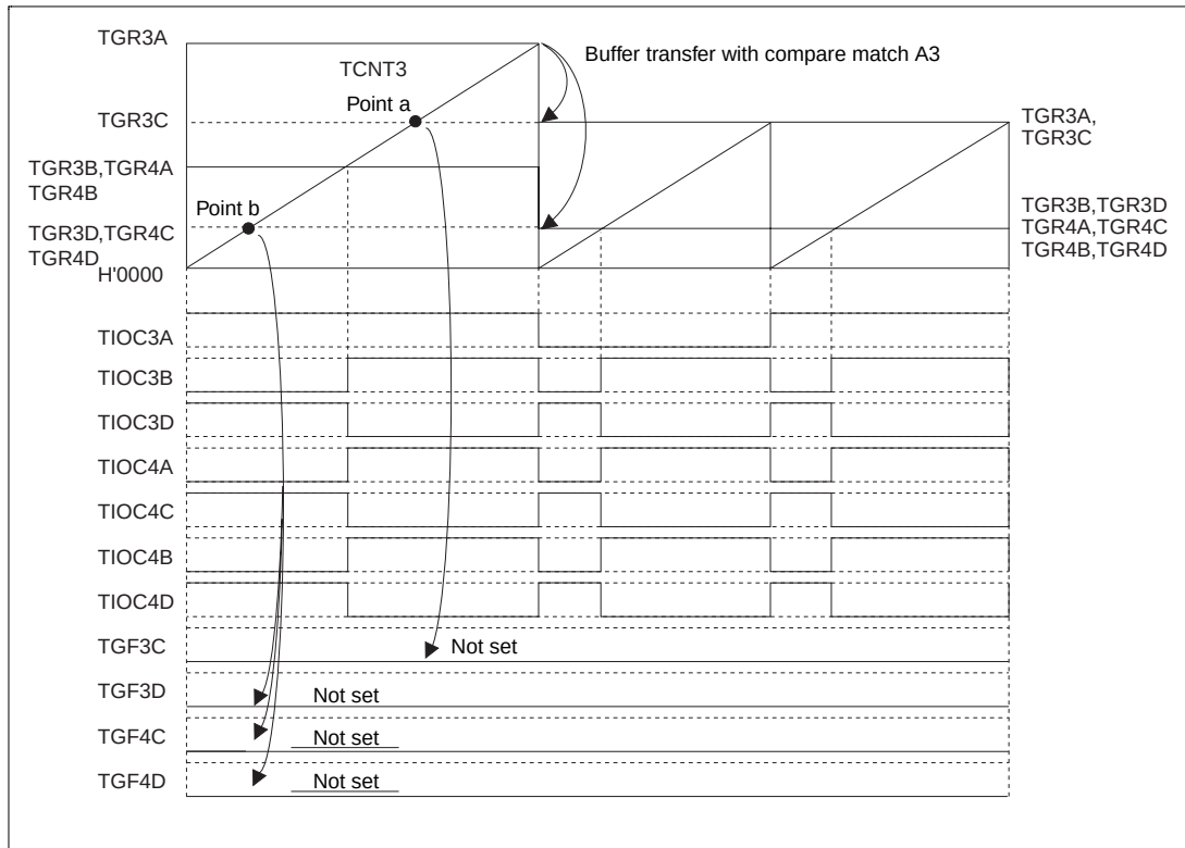
Figure 12.89 Buffer Operation and Compare-Match Flags in Reset Sync PWM Mode (for A Mask)
