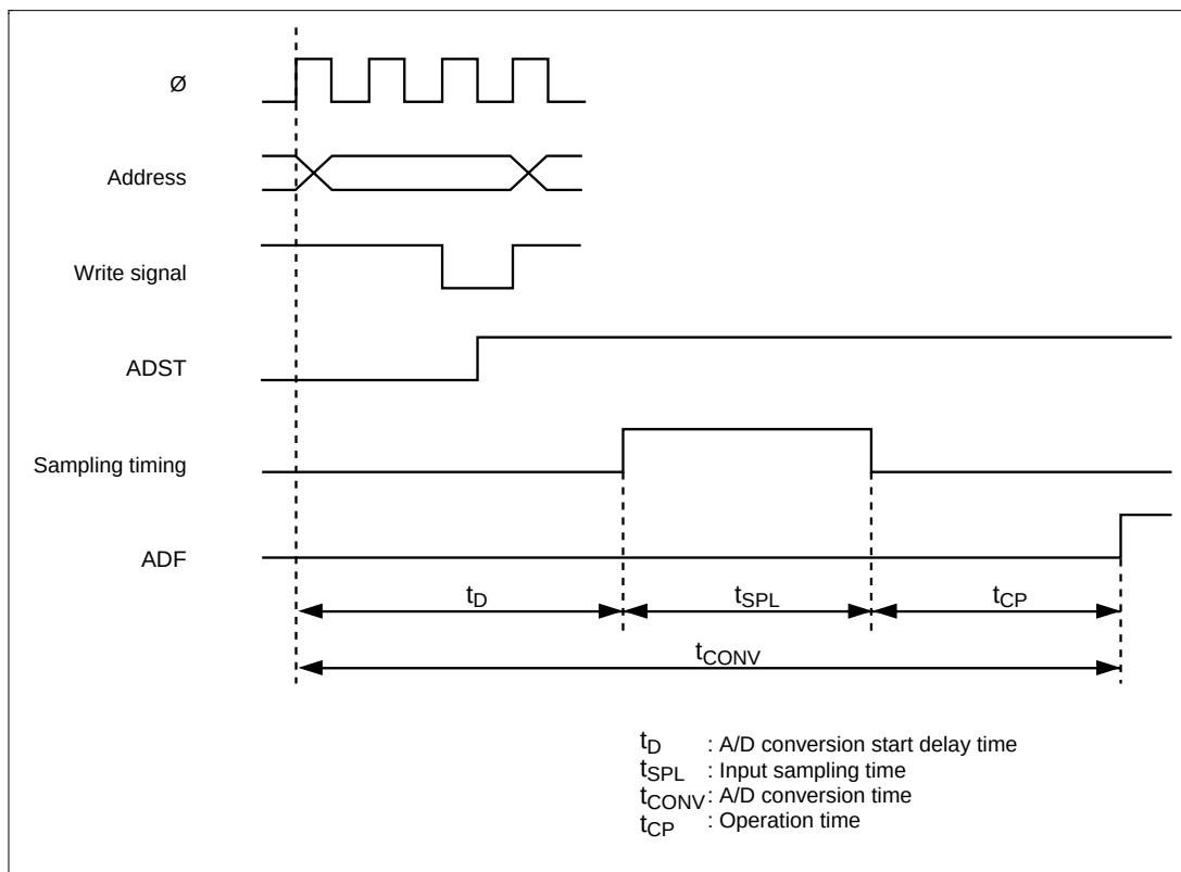
Figure 27.32 Analog Conversion Timing
