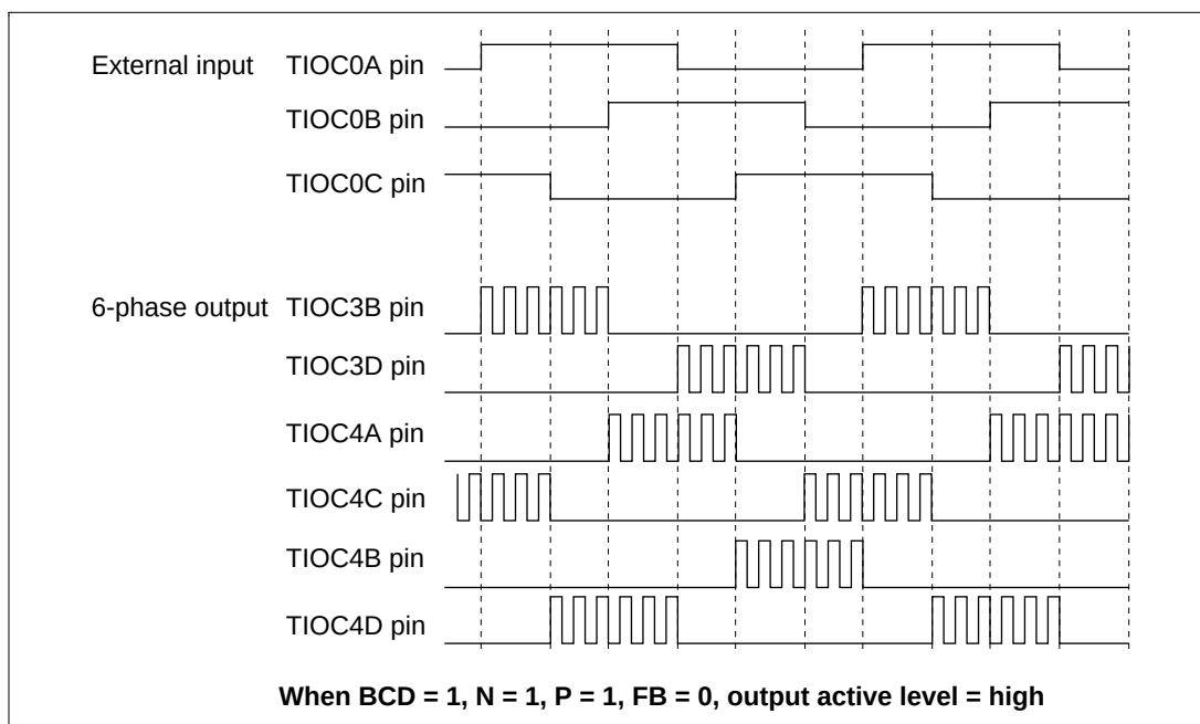
Figure 12.57 Example of Output Phase Switching by External Input (2)
