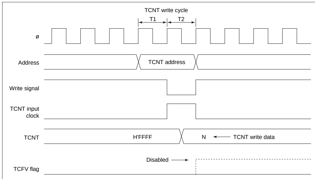
Figure 12.95 Contention between TCNT Write and Overflow
