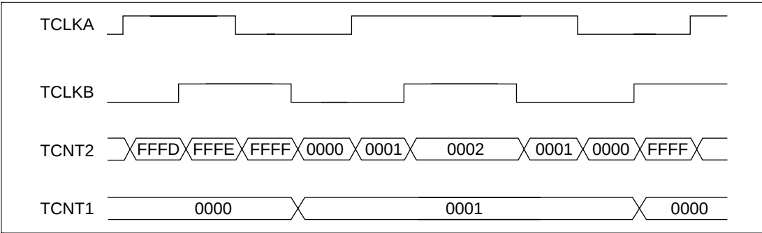
Figure 12.24 Cascade Connection Operation Example (Phase Counting Mode)
