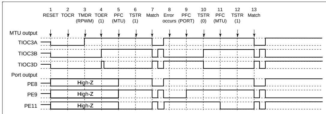
Figure 12.125 Error Occurrence in Reset-Synchronous PWM Mode, Recovery in Reset-Synchronous PWM Mode
