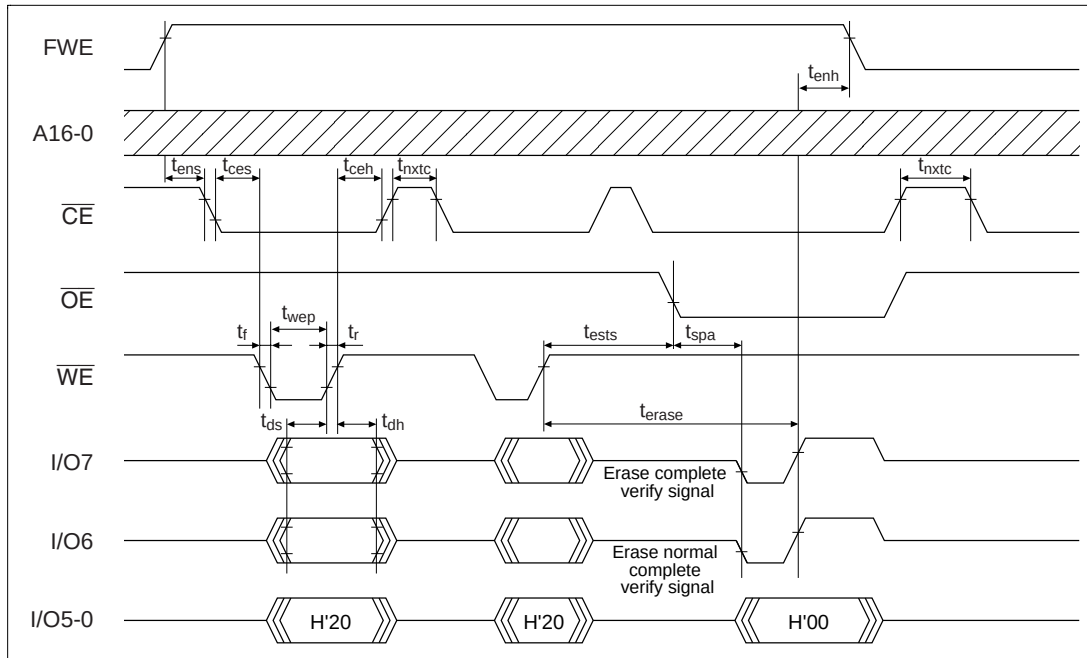
Figure 22.20 Auto-Erase Mode Timing Waveforms
