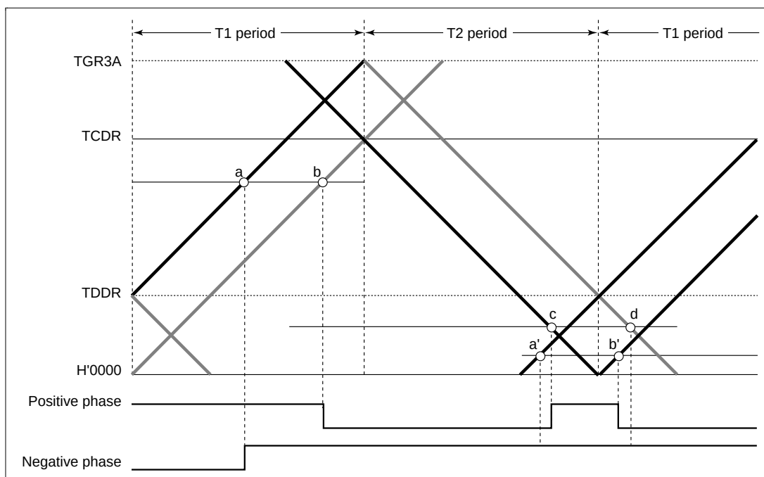
Figure 12.48 Example of Complementary PWM Mode Waveform Output (3)
