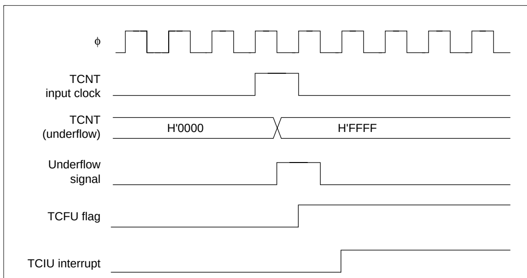
Figure 12.73 TCIU Interrupt Setting Timing
