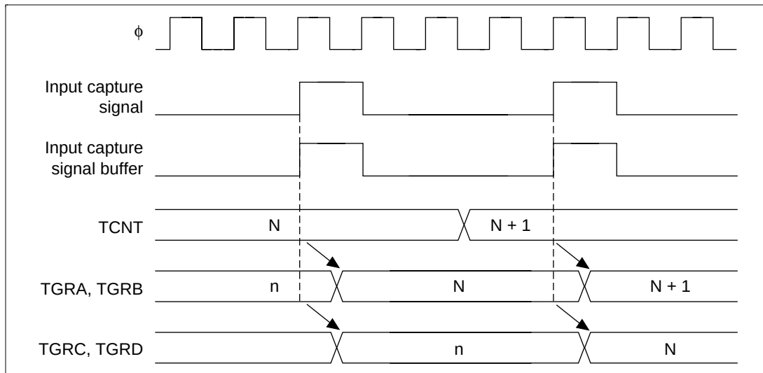
Figure 12.69 Buffer Operation Timing (Input Capture)
