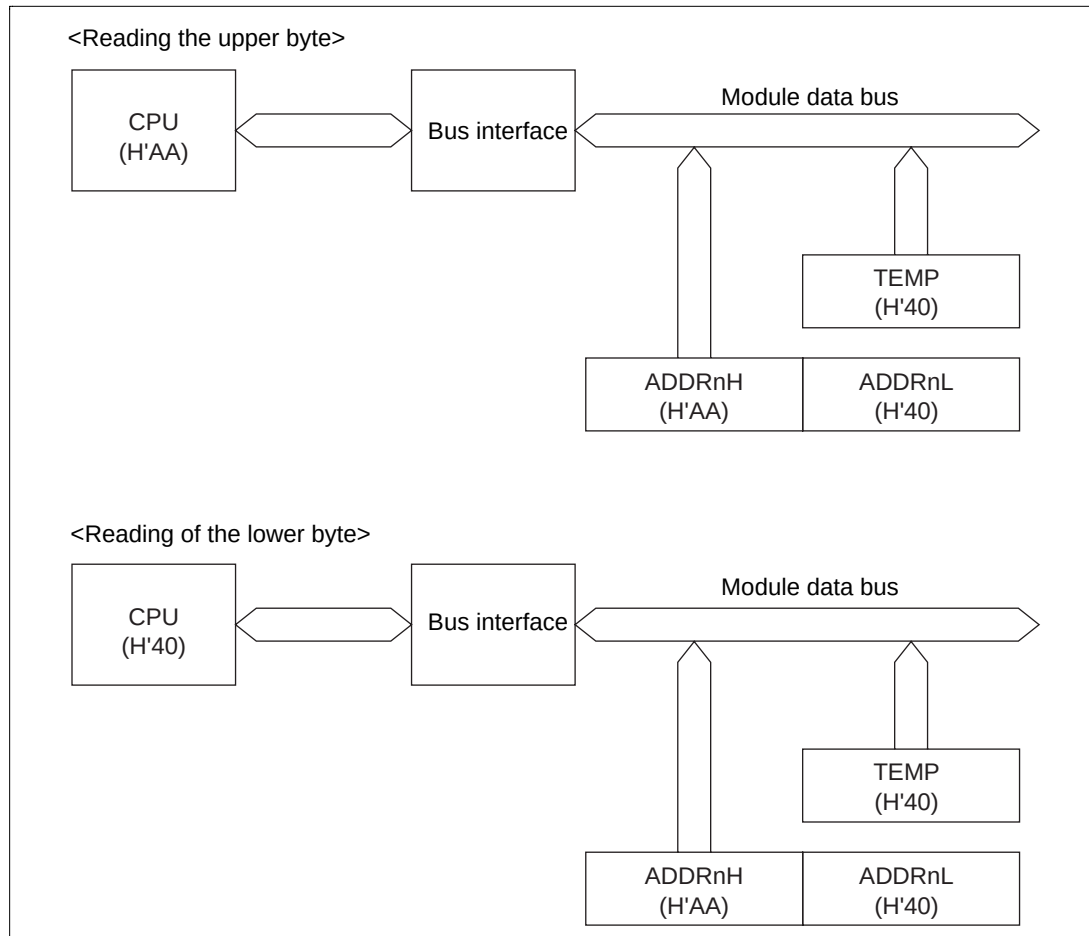
Figure 16.2 ADDR Access Operation (During Reading of (H'AA40))
