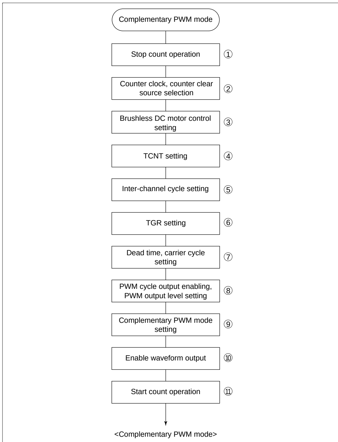
Figure 12.39 Example of Complementary PWM Mode Setting Procedure
