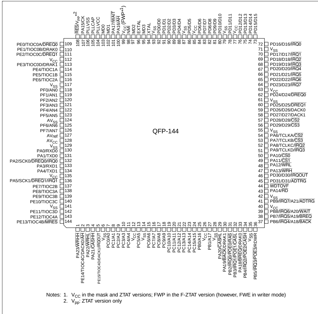
Figure 1.4 SH7041, SH7043, SH7045 Pin Arrangement (QFP-144 Top View)
