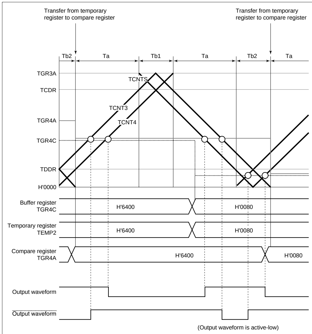
Figure 12.41 Example of Complementary PWM Mode Operation
