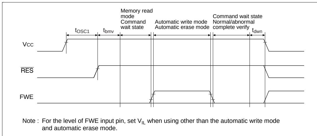
Figure 22.22 Oscillation Stabilization Time and Boot Program Transfer Time
