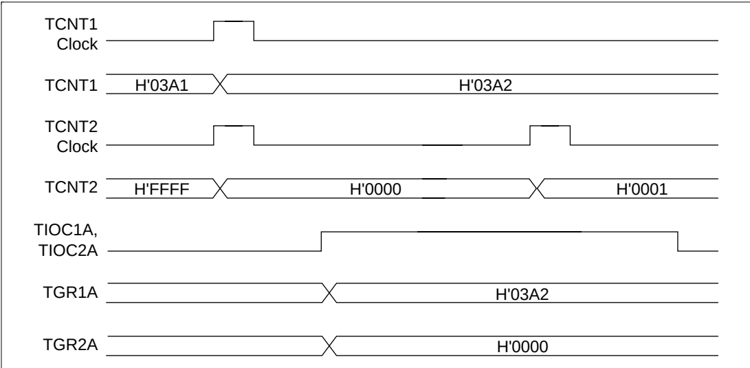
Figure 12.23 Cascade Connection Operation Example (Input Capture)
