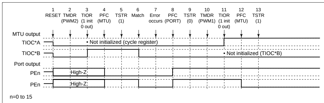
Figure 12.110 Error Occurrence in PWM Mode 2, Recovery in PWM Mode 1
