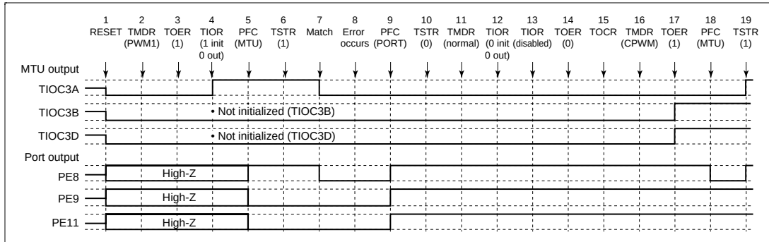
Figure 12.107 Error Occurrence in PWM Mode 1, Recovery in Complementary PWM Mode
