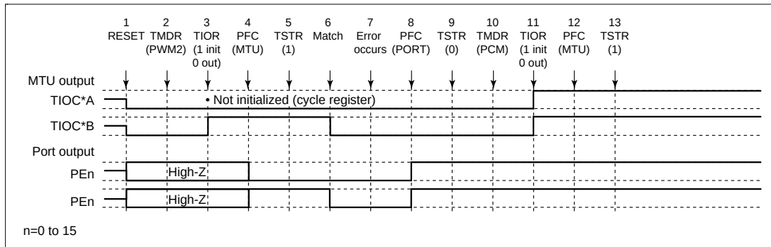
Figure 12.112 Error Occurrence in PWM Mode 2, Recovery in Phase Counting Mode
