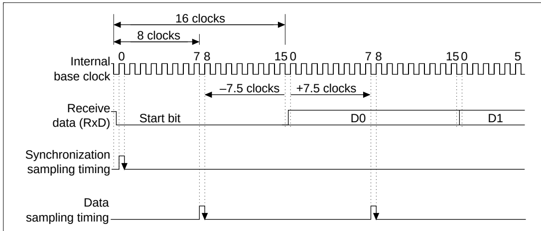
Figure 14.23 Receive Data Sampling Timing in Asynchronous Mode
