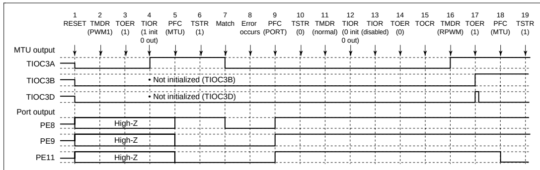
Figure 12.108 Error Occurrence in PWM Mode 1, Recovery in Reset-Synchronous PWM Mode
