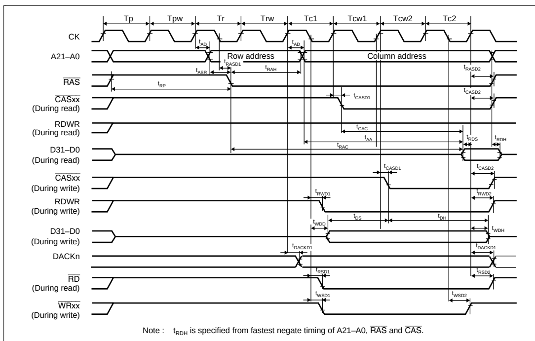
Figure 26.13 DRAM Cycle (Normal Mode, 2 Waits, TPC = 1, RCD = 1)
