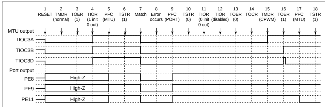
Figure 12.102 Error Occurrence in Normal Mode, Recovery in Reset-Synchronous PWM Mode
