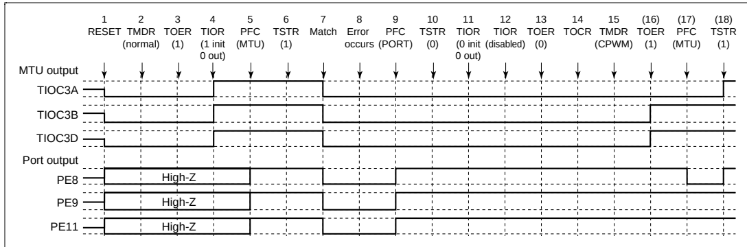
Figure 12.101 Error Occurrence in Normal Mode, Recovery in Complementary PWM Mode
