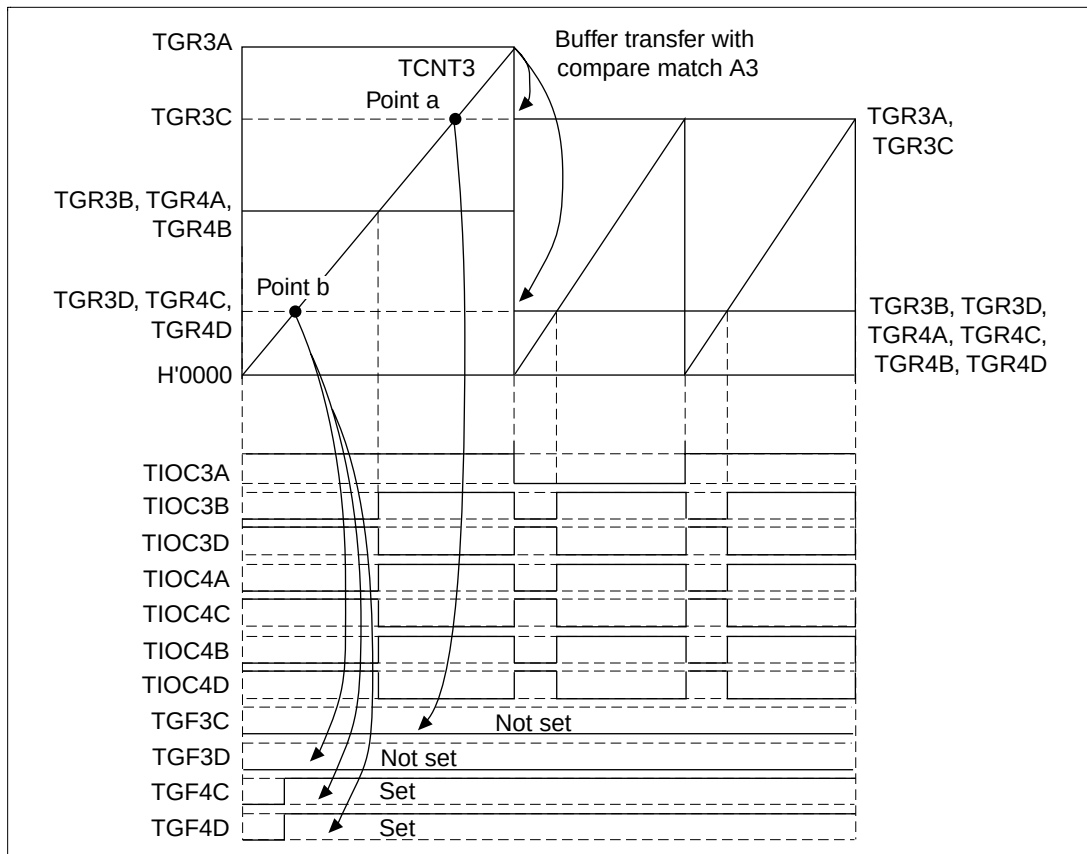
Figure 12.88 Buffer Operation and Compare-Match Flags in Reset Sync PWM Mode
