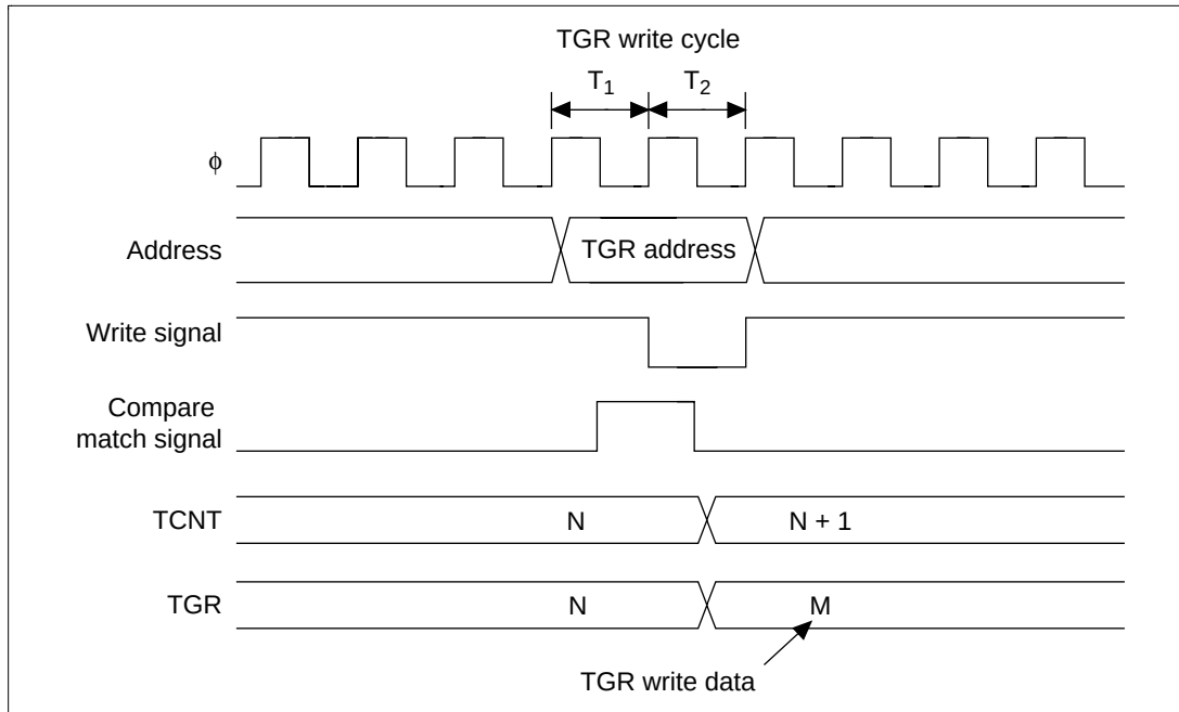
Figure 12.85 TGR Write and Compare Match Contention
