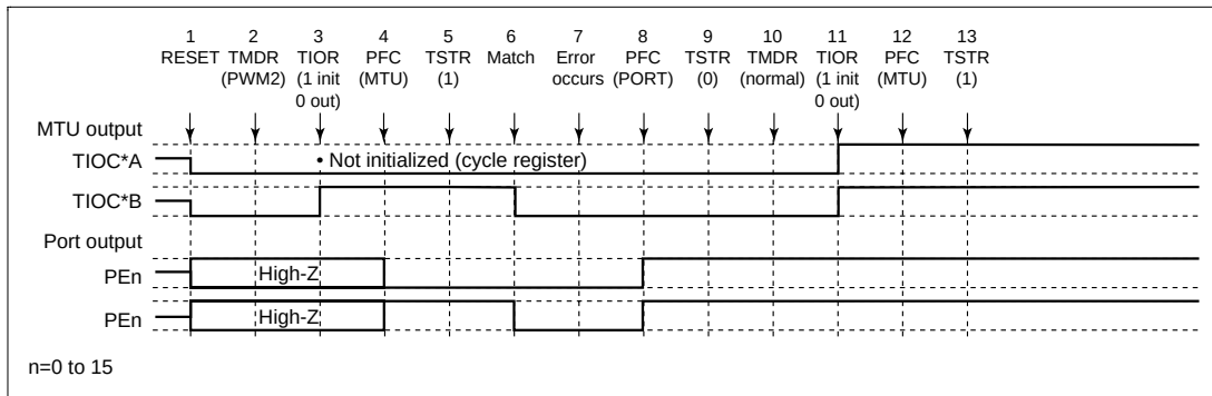
Figure 12.109 Error Occurrence in PWM Mode 2, Recovery in Normal Mode
