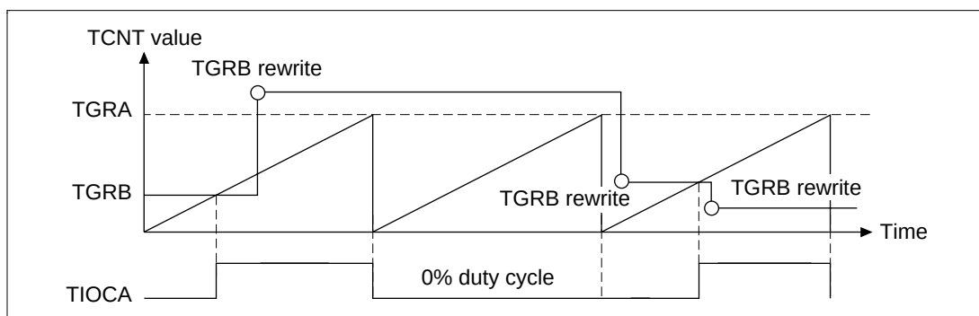
Figure 12.28 PWM Mode Operation Example (0% Duty Cycle)
