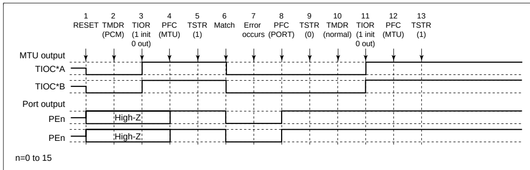
Figure 12.113 Error Occurrence in Phase Counting Mode, Recovery in Normal Mode
