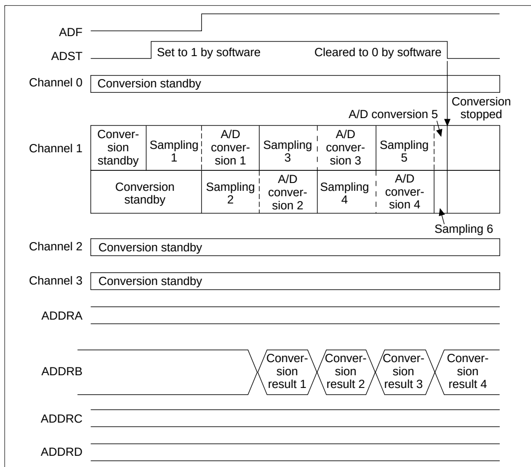
Figure 15.4 A/D Converter Operation Example (Select-Scan Mode)
