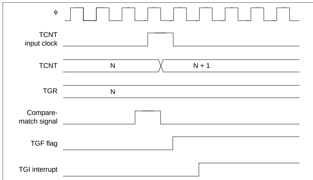
Figure 12.70 TGI Interrupt Timing (Compare Match)
