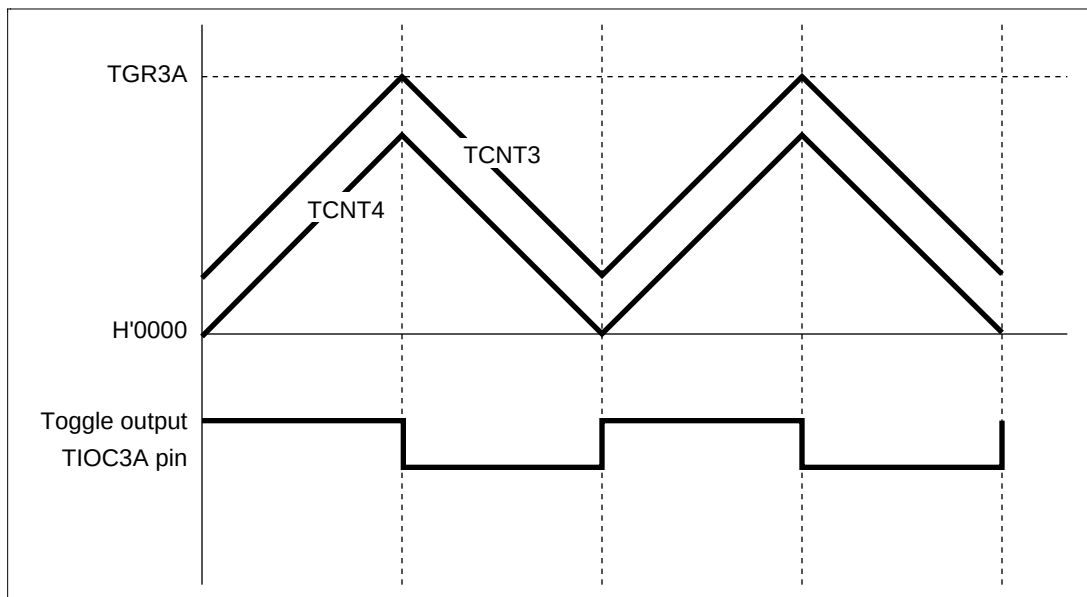
Figure 12.54 Example of Toggle Output Waveform Synchronized with PWM Output
