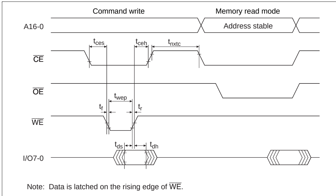
Figure 22.15 Timing Waveforms for Memory Read after Memory Write
