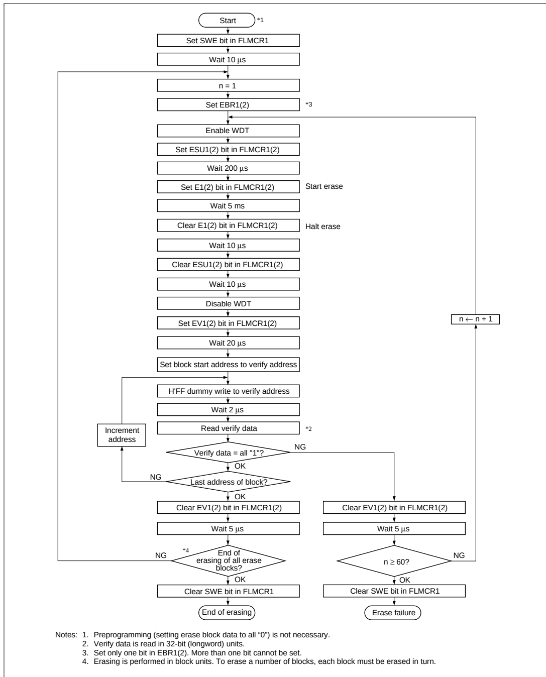
Figure 22.8 Erase/Erase-Verify Flowchart (Single Block Erase)
