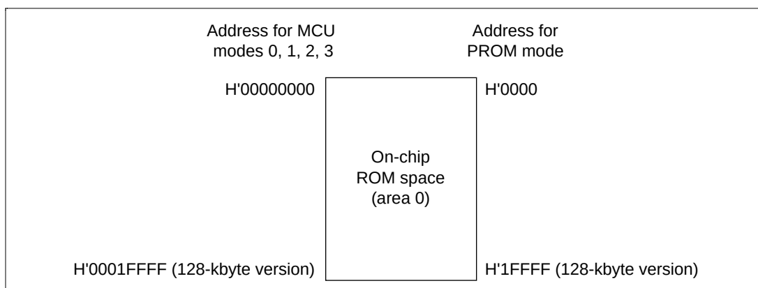
Figure 21.4 On-Chip ROM Memory Map
