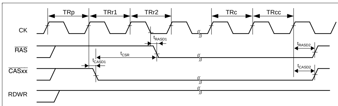
Figure 27.18 Self Refresh
