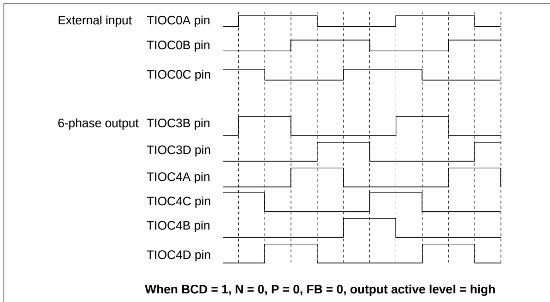
Figure 12.56 Example of Output Phase Switching by External Input (1)
