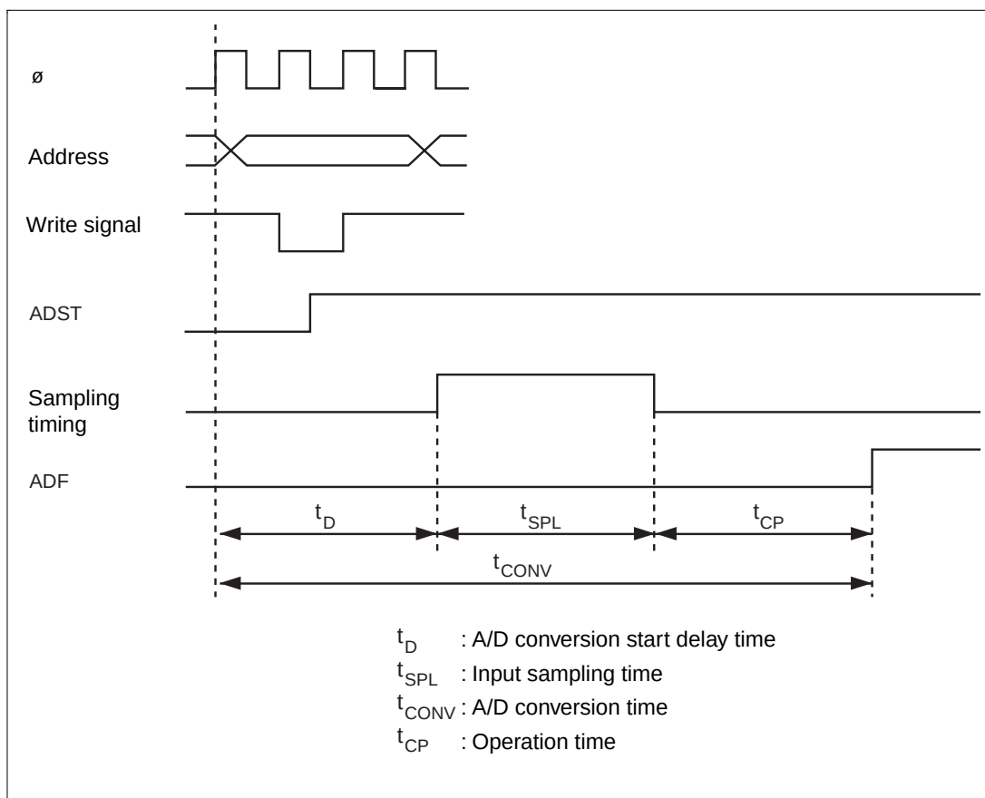
Figure 26.32 Analog Conversion Timing
