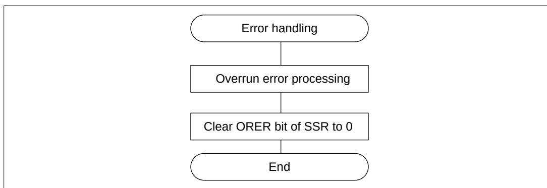
Figure 14.20 Sample Flowchart for Serial Receiving (cont)
