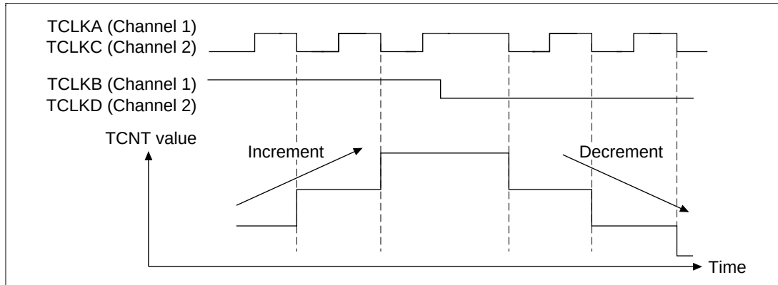
Figure 12.32 Phase Counting Mode 2 Operation
