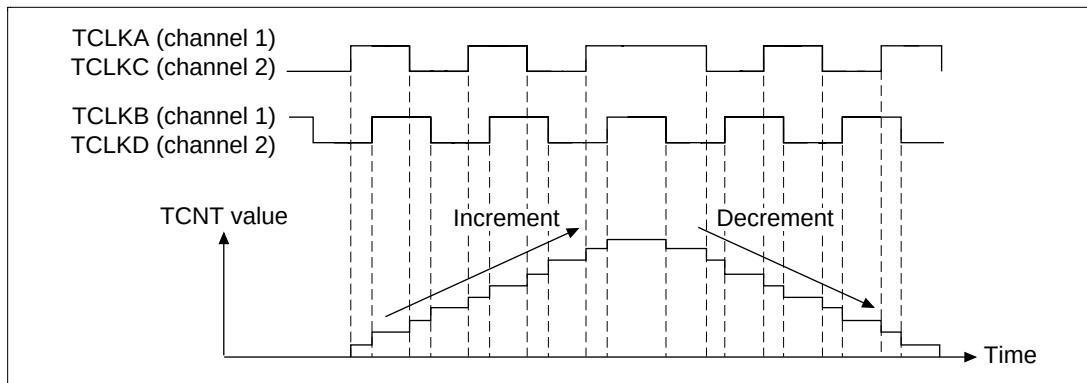
Figure 12.31 Phase Counting Mode 1 Operation
