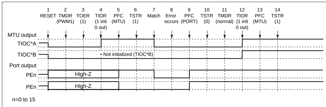
Figure 12.103 Error Occurrence in PWM Mode 1, Recovery in Normal Mode
