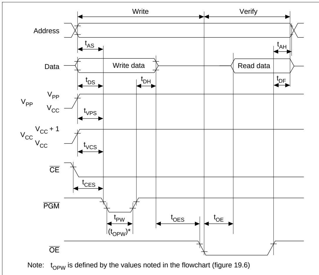
Figure 21.6 Write/Verify Timing
