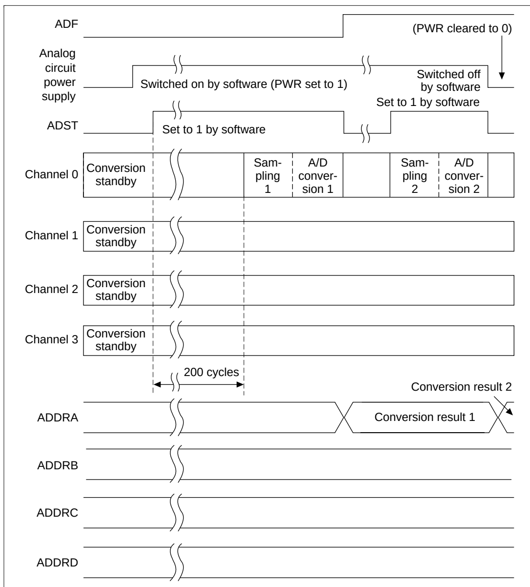
Figure 15.10 Conversion Start Operation (High-Speed Start Mode)
