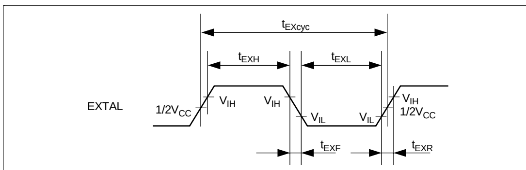
Figure 27.2 EXTAL Clock Input Timing
