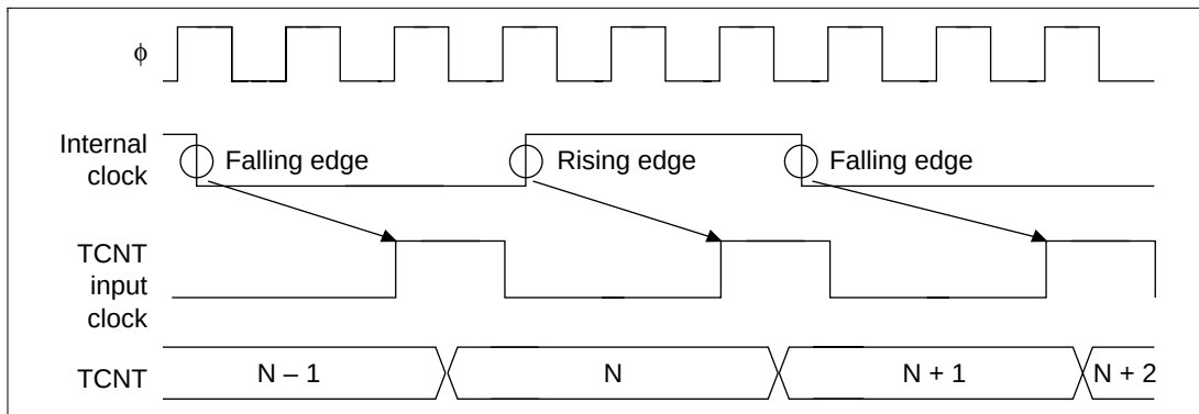
Figure 12.61 TCNT Count Timing during External Clock Operation (Normal Mode)
