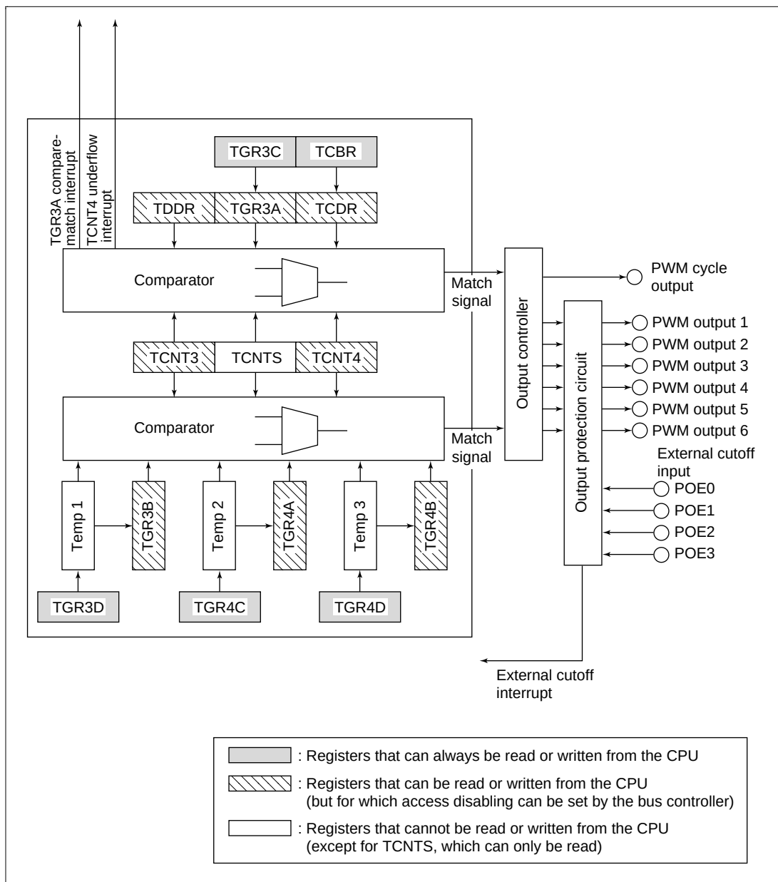
Figure 12.38 Block Diagram of Channels 3 and 4 in Complementary PWM Mode
