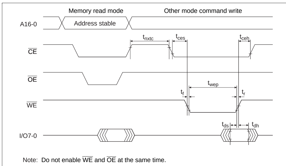
Figure 22.16 Timing Waveforms in Transition from Memory Read Mode to Another Mode
