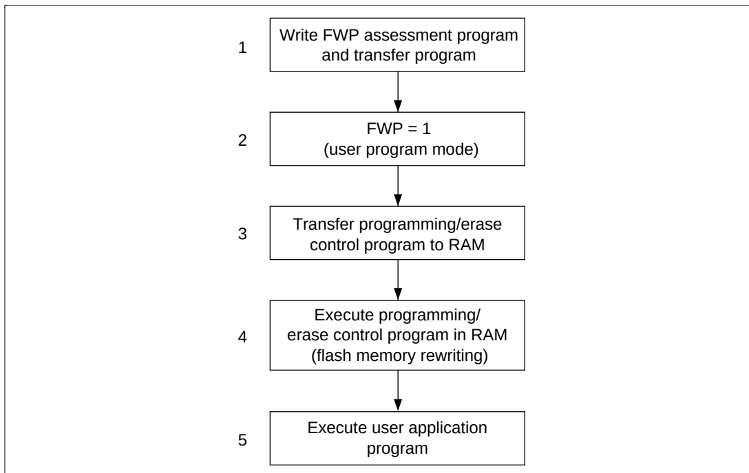
Figure 22.6 User Program Mode Execution Procedure
