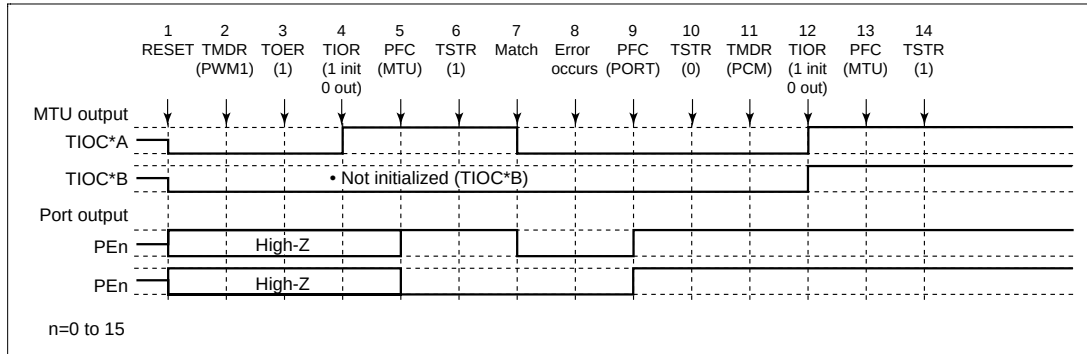
Figure 12.106 Error Occurrence in PWM Mode 1, Recovery in Phase Counting Mode
