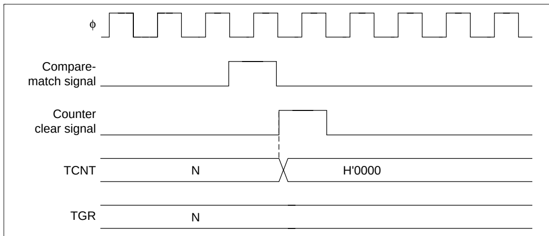
Figure 12.66 Counter Clearing Timing (Compare-Match)
