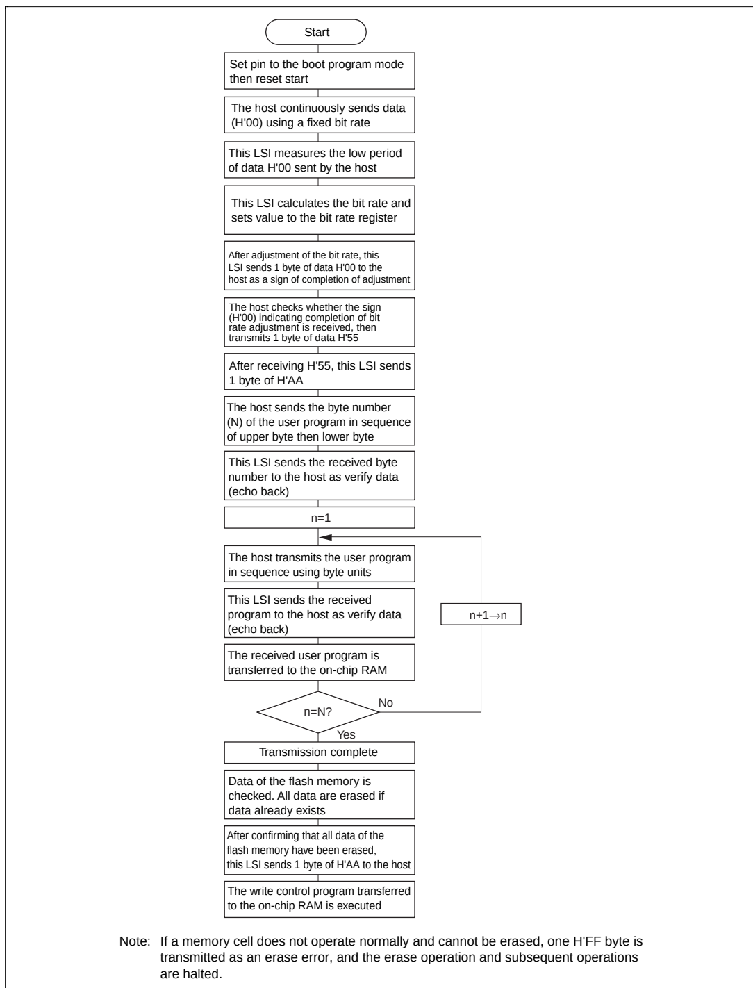
Figure 22.4 Boot Mode Execution Procedure
