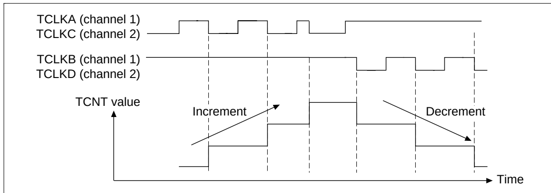
Figure 12.33 Phase Counting Mode 3 Operation
