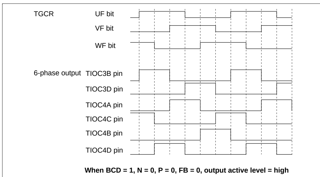
Figure 12.58 Example of Output Phase Switching by Means of UF, VF, WF Bit Settings (1)
