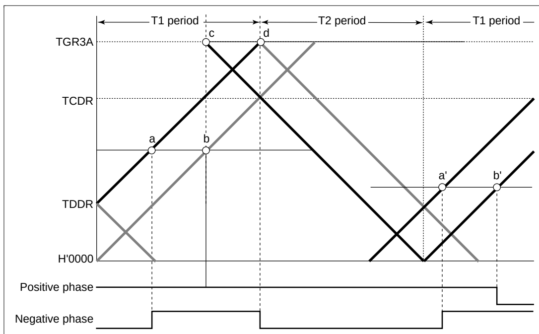
Figure 12.49 Example of Complementary PWM Mode 0% and 100% Waveform Output (1)
