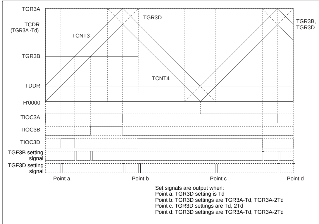
Figure. 12.93 Special Properties of Compare Match Flag in Complementary PWM Mode (for A Mask)
