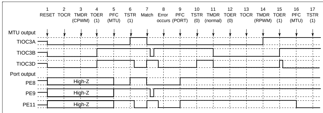
Figure 12.121 Error Occurrence in Complementary PWM Mode, Recovery in Reset-Synchronous PWM Mode
