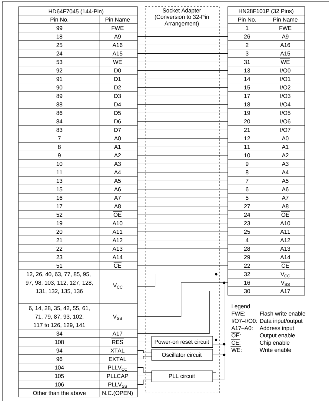
Figure 22.14 Socket Adapter Pin Correspondence Diagram (SH7045)
