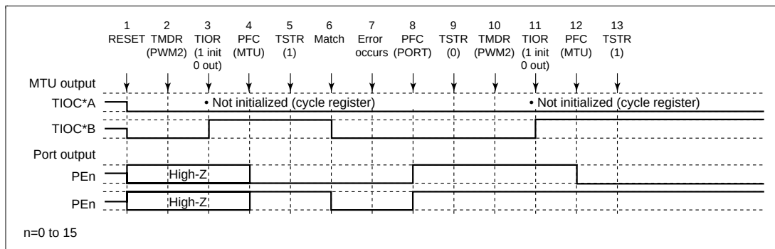
Figure 12.111 Error Occurrence in PWM Mode 2, Recovery in PWM Mode 2
