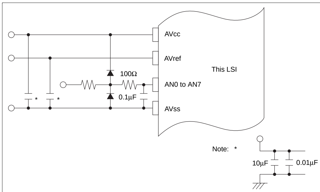
Figure 15.13 Example of a Protection Circuit for the Analog Input Pins
