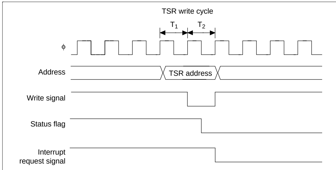
Figure 12.75 Timing of Status Flag Clearing by the CPU
