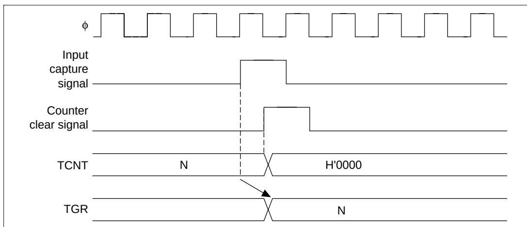
Figure 12.67 Counter Clearing Timing (Input Capture)
