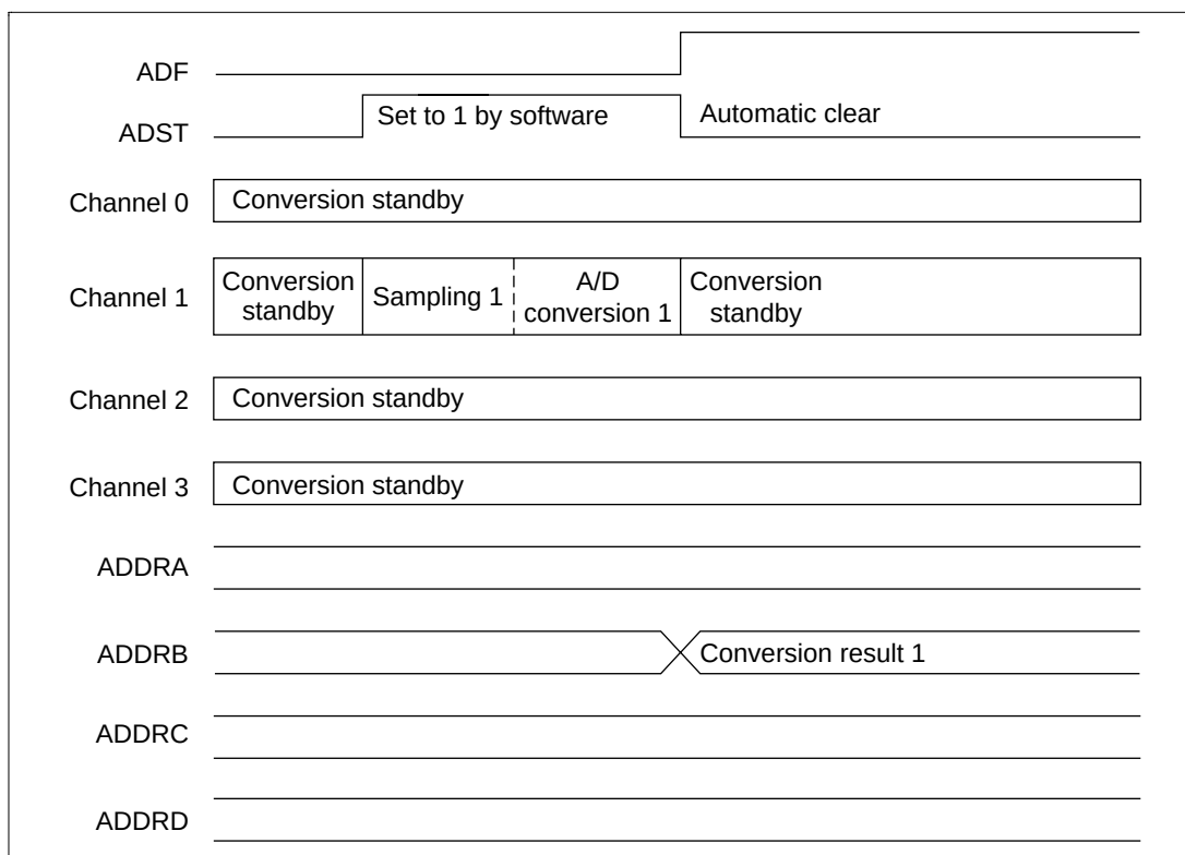
Figure 15.3 A/D Converter Operation Example (Select-Single Mode)
