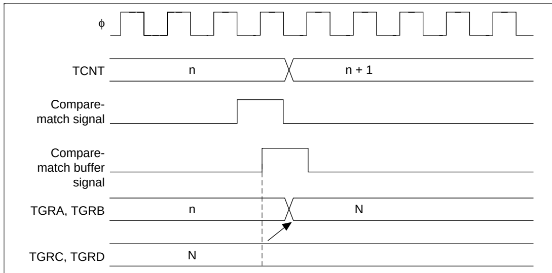
Figure 12.68 Buffer Operation Timing (Compare-Match)
