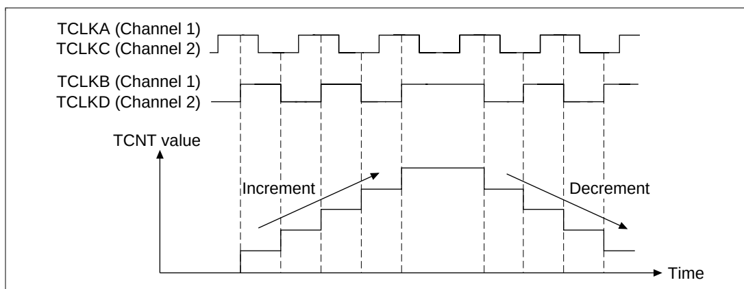
Figure 12.34 Phase Counting Mode 4 Operation
