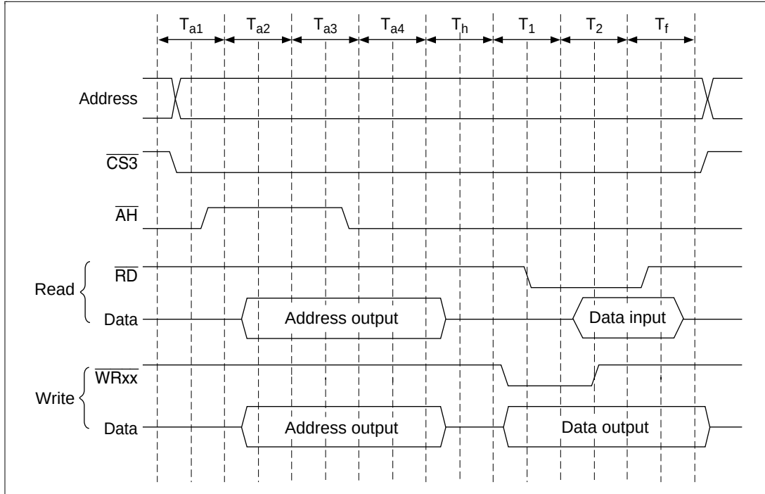
Figure 10.19 Wait timing during address/data multiplex I/O space when CS assort extension is set
