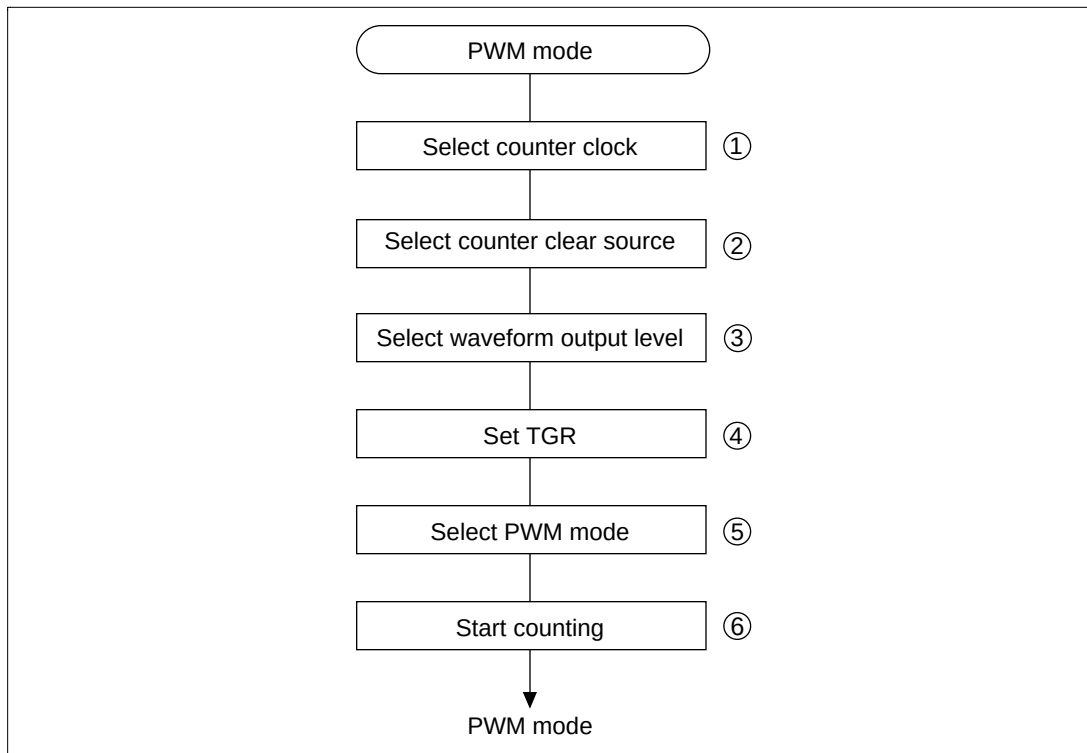
Figure 12.25 Procedure for Selecting the PWM Mode
