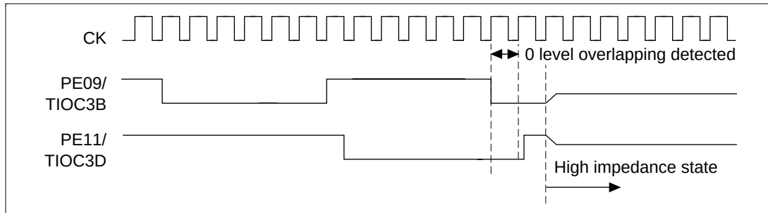
Figure 12.128 Output-Level Detection Operation
