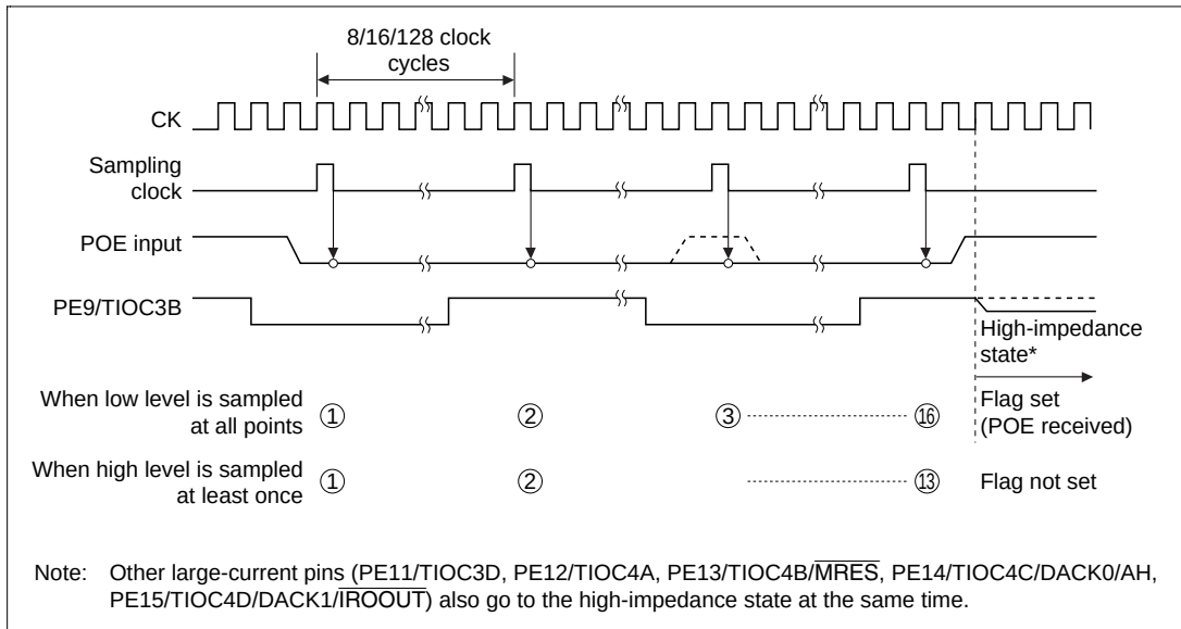
Figure 12.127 Low-Level Detection Operation
