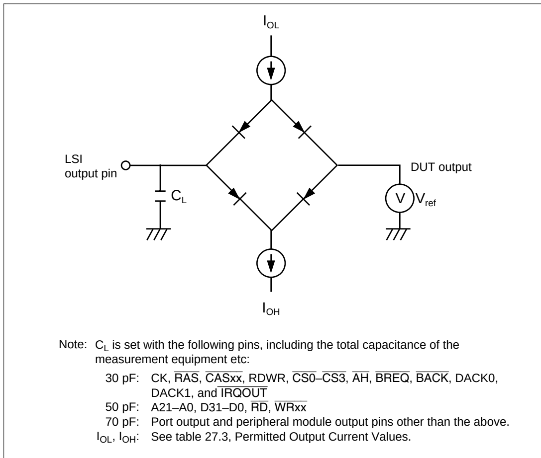
Figure 27.33 Output Added Circuit
