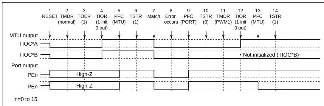
Figure 12.98 Error Occurrence in Normal Mode, Recovery in PWM Mode 1
