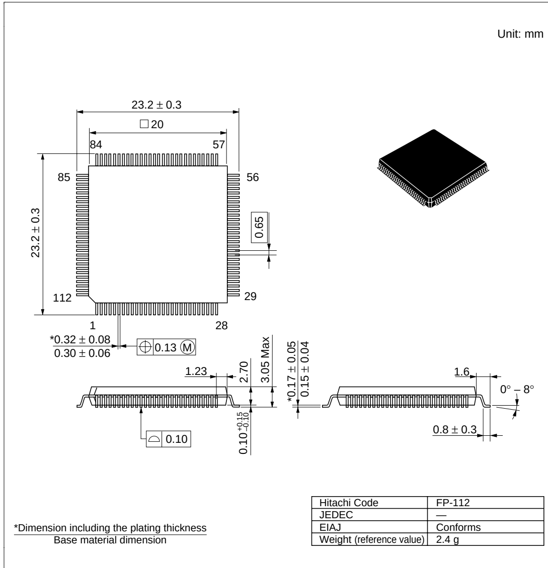
Figure D.1 Package Dimensions (FP-112)
