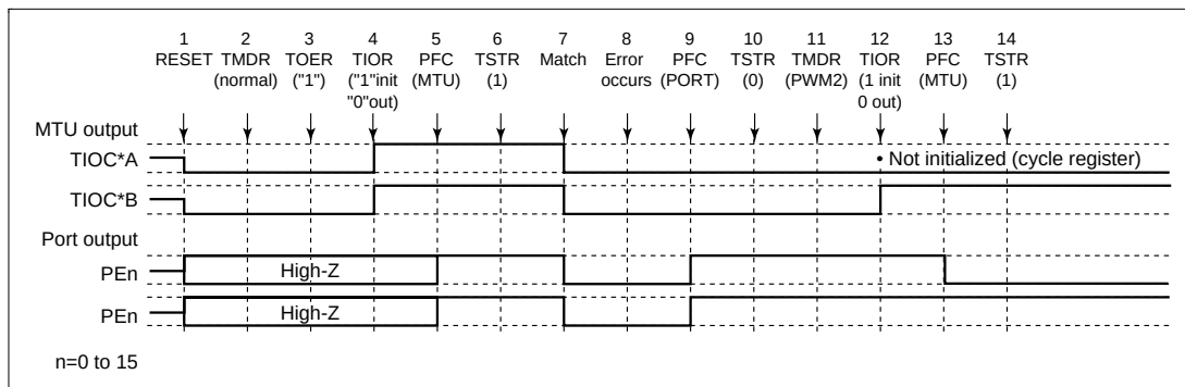
Figure 12.99 Error Occurrence in Normal Mode, Recovery in PWM Mode 2
