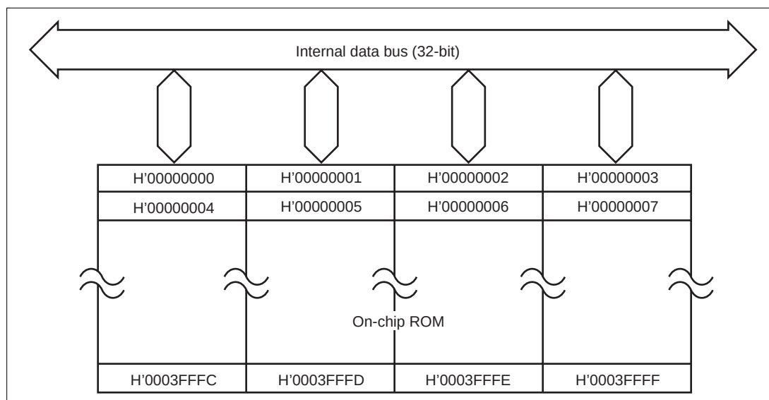
Figure 20.3 Mask ROM Block Diagram (256kbyte version)
