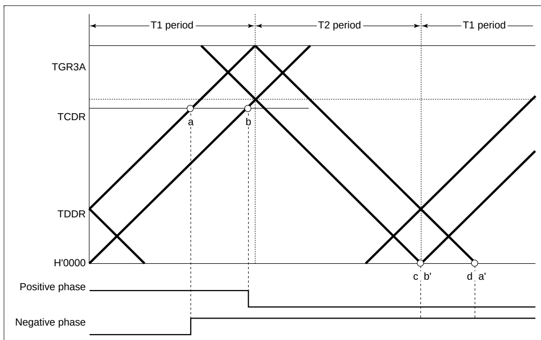
Figure 12.52 Example of Complementary PWM Mode 0% and 100% Waveform Output (4)
