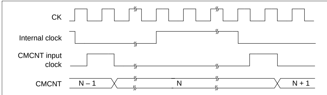
Figure 17.3 Count Timing
