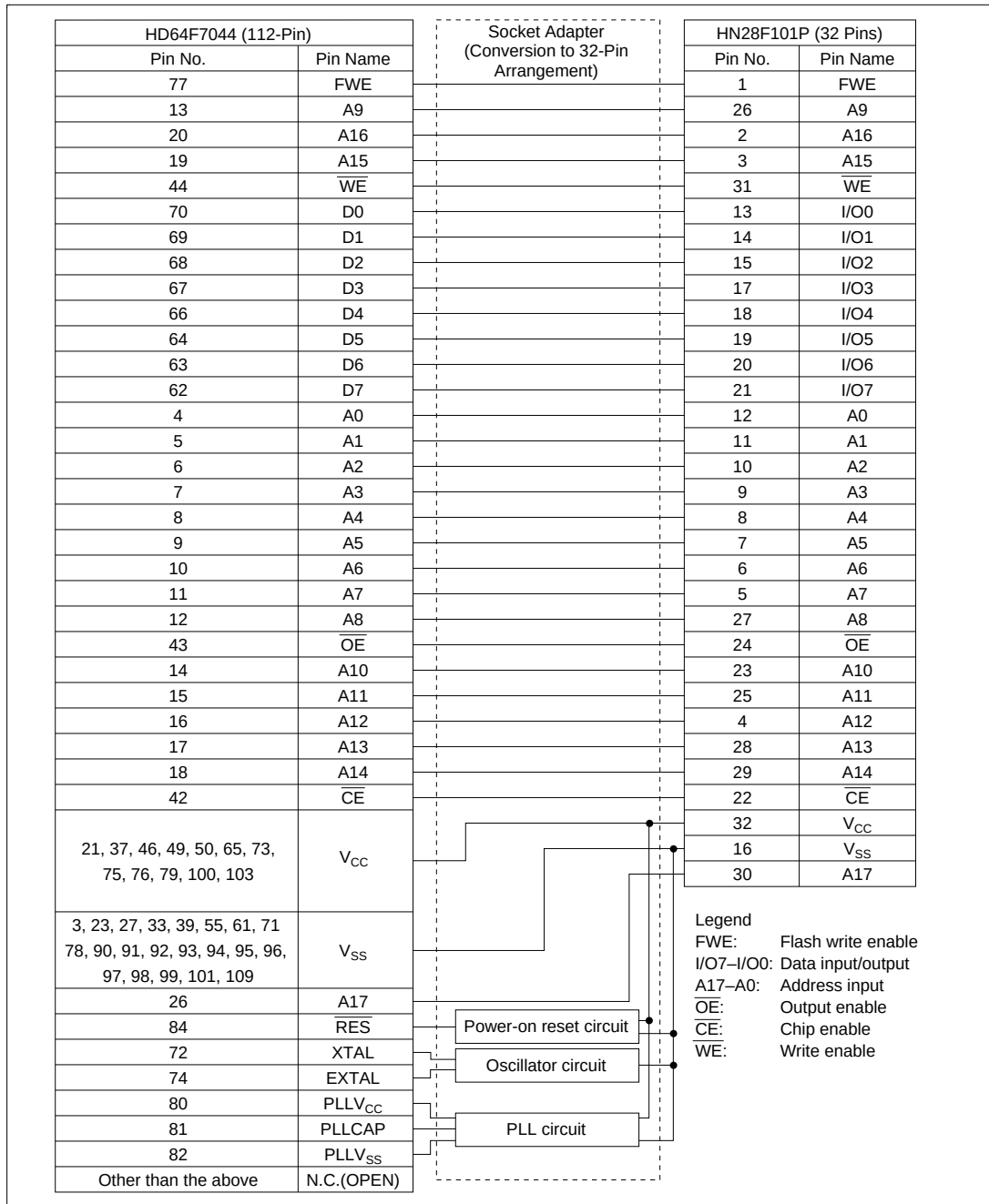
Figure 22.13 Socket Adapter Pin Correspondence Diagram (SH7044)
