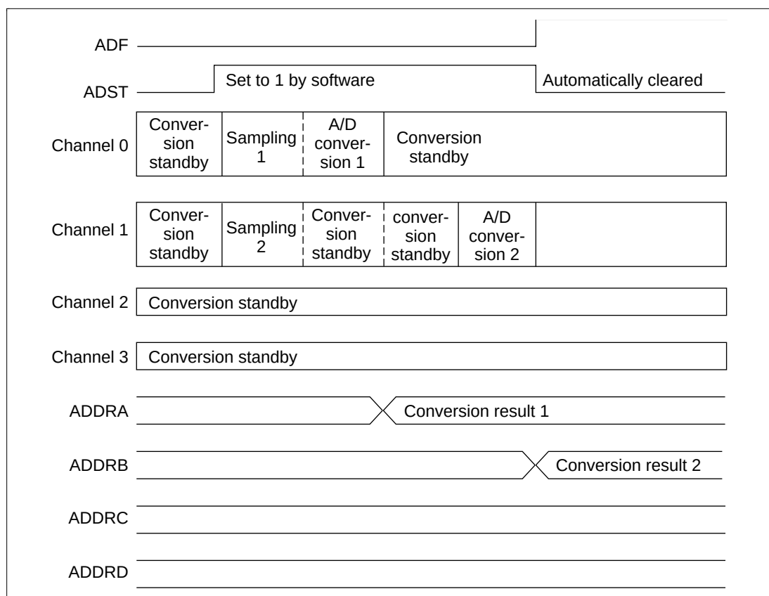
Figure 15.8 Simultaneous Sampling Operation (Group Single Mode)
