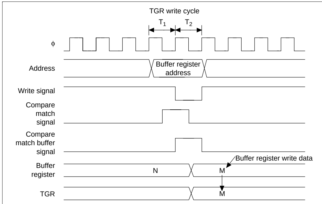
Figure 12.80 TGR Write and Compare-Match Contention (Channel 0)
