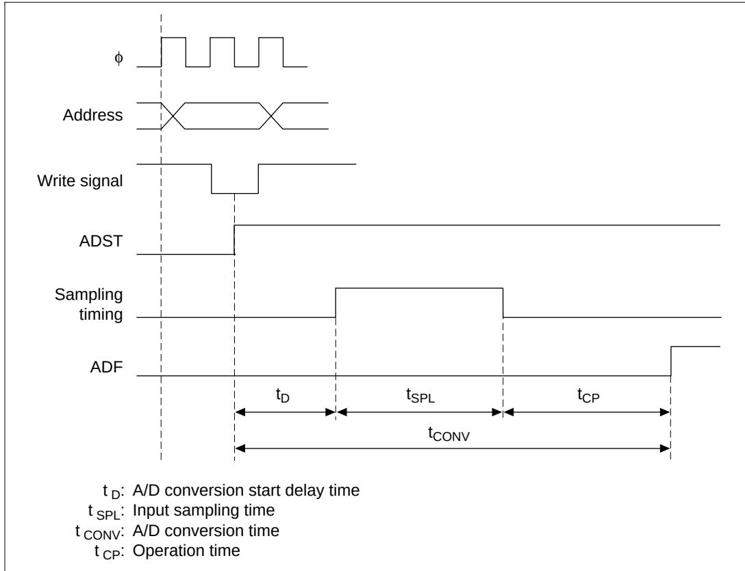
Figure 15.12 A/D Conversion Timing
