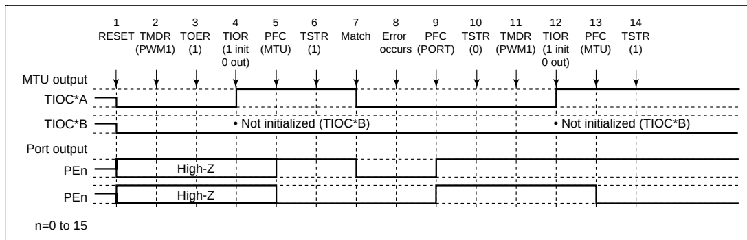
Figure 12.104 Error Occurrence in PWM Mode 1, Recovery in PWM Mode 1
