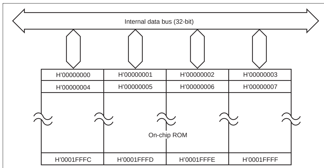
Figure 20.2 Mask ROM Block Diagram (128kbyte version)
