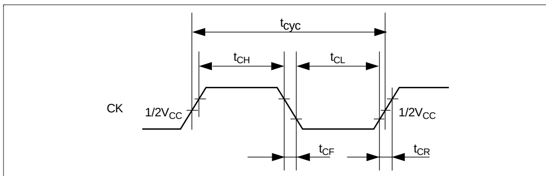
Figure 27.1 System Clock Timing
