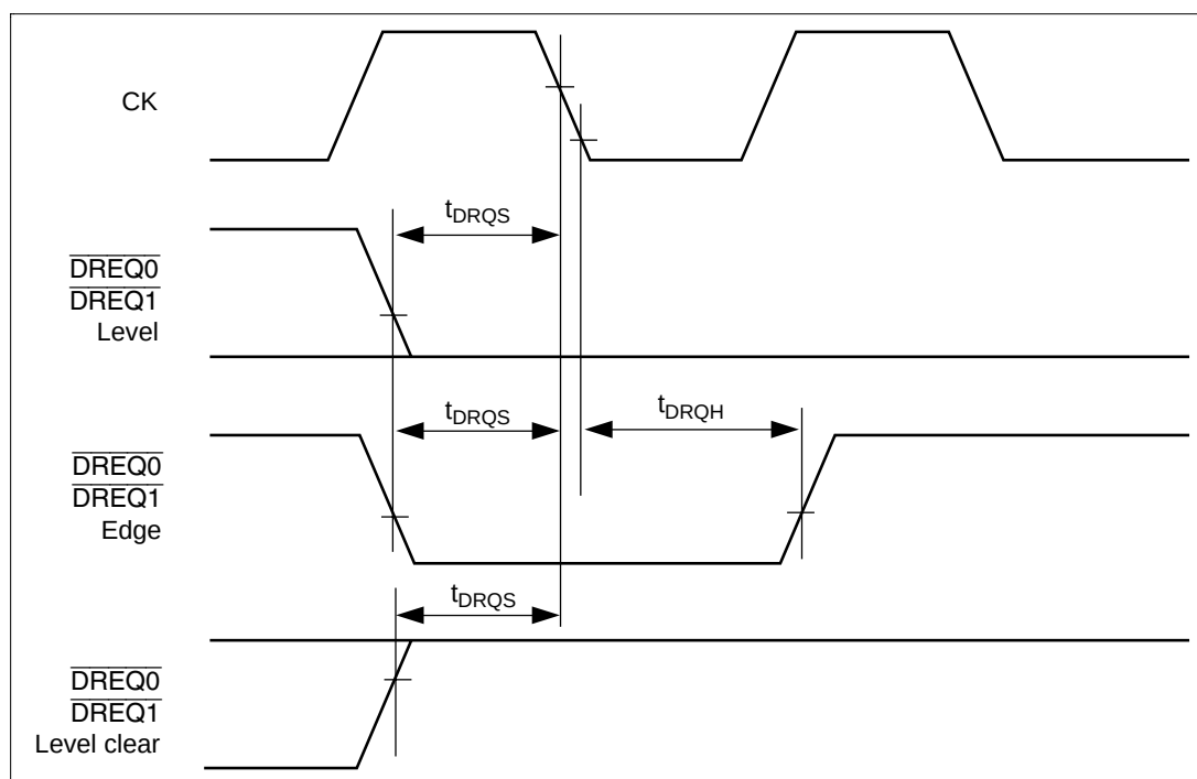
Figure 27.20 \overline{DREQ0} and \overline{DREQ1} Input Timing (1)
