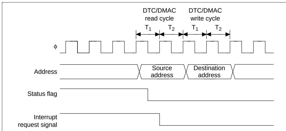
Figure 12.76 Timing of Status Flag Clearing by DTC/DMA Activation
