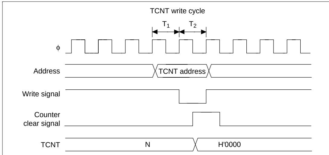
Figure 12.78 TCNT Write and Clear Contention
