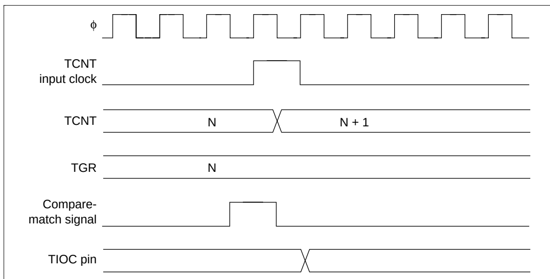
Figure 12.63 Output Compare Output Timing (Normal Mode/PWM Mode)
