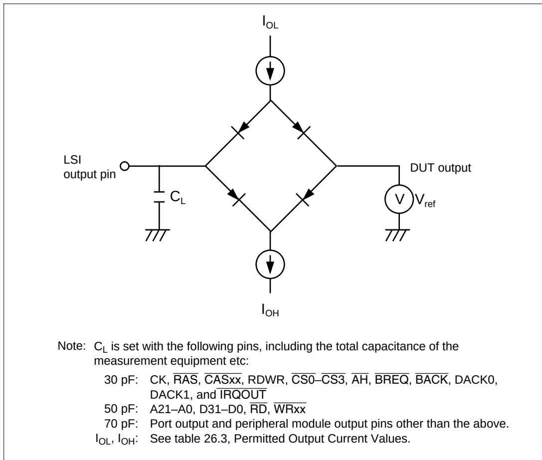
Figure 26.33 Output Test Circuit
