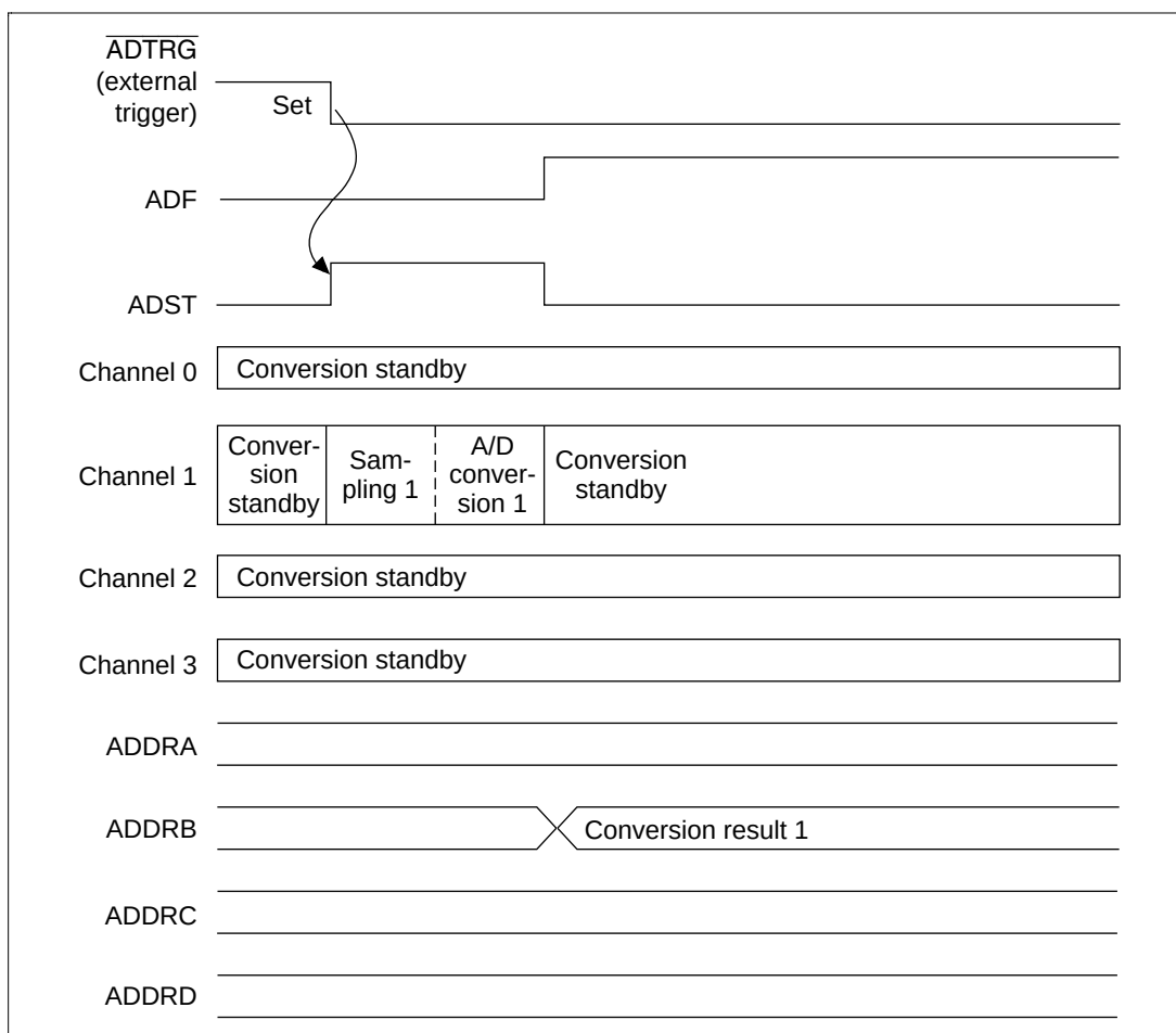
Figure 15.11 Conversion Start by \overline{\text{ADTRG}} Conversion Start Trigger
