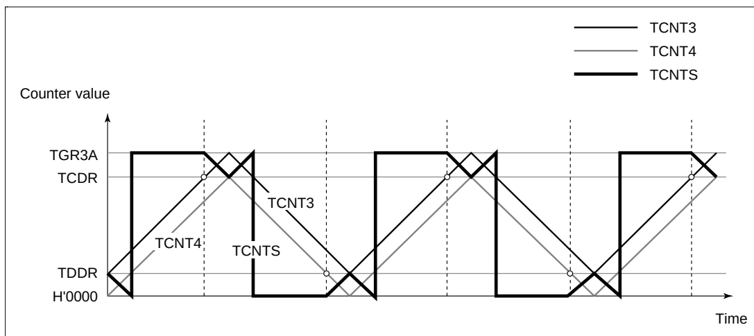
Figure 12.40 Complementary PWM Mode Counter Operation
