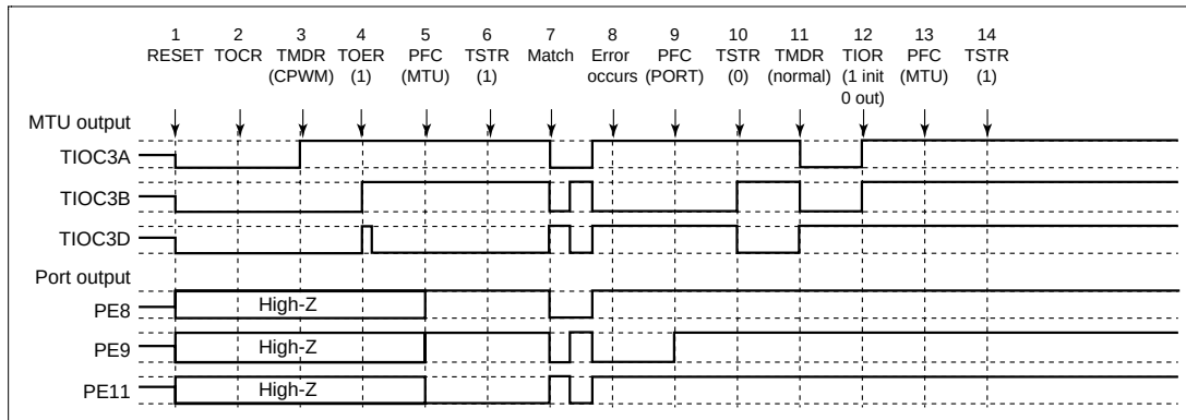
Figure 12.122 Error Occurrence in Reset-Synchronous PWM Mode, Recovery in Normal Mode
