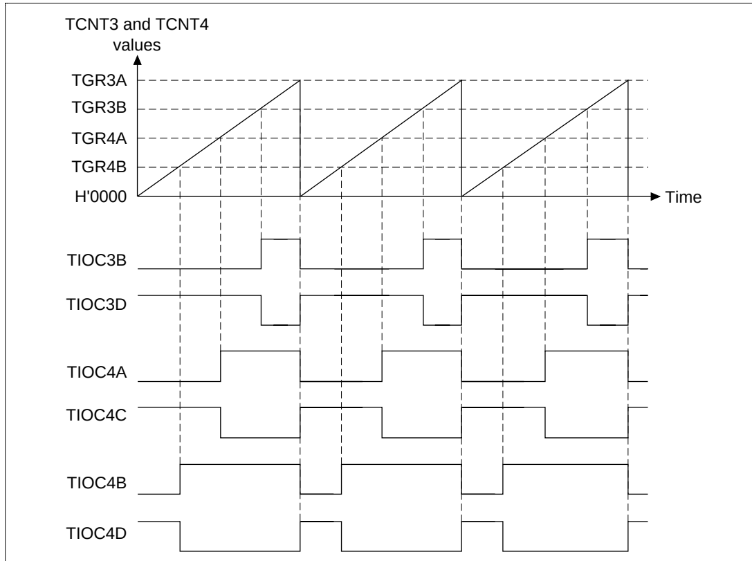
Figure 12.37 Reset-Synchronized PWM Mode Operation Example (When the TOCR's OLSN = 1 and OLSP = 1)
