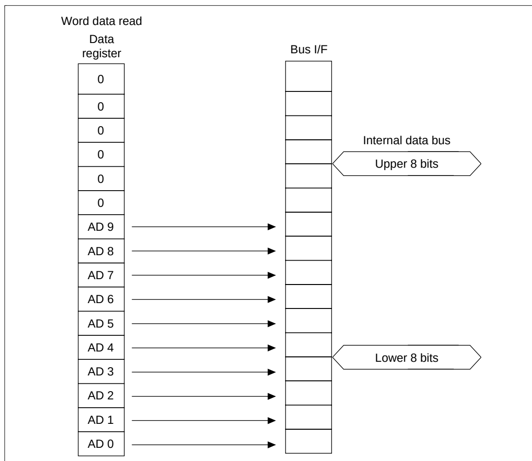
Figure 15.2 ADDR Read Operation
