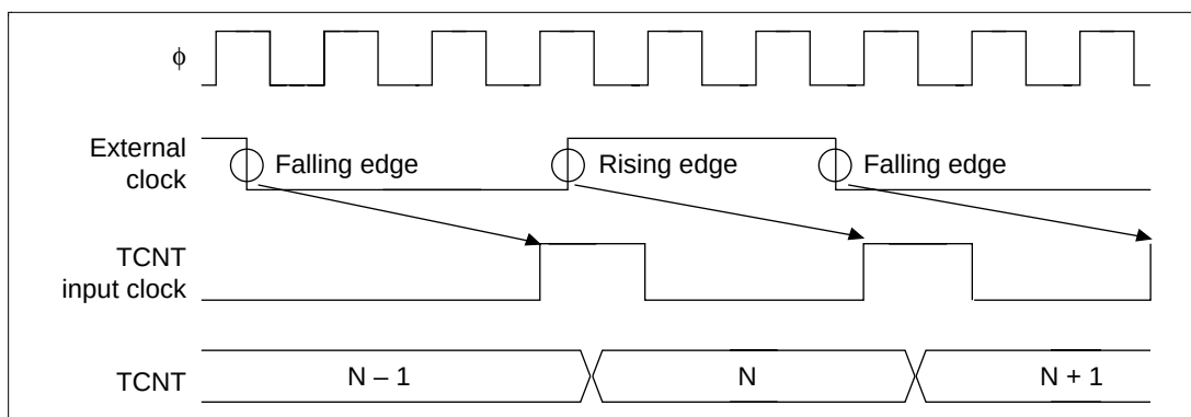
Figure 12.62 TCNT Count Timing during External Clock Operation (Phase Counting Mode)
