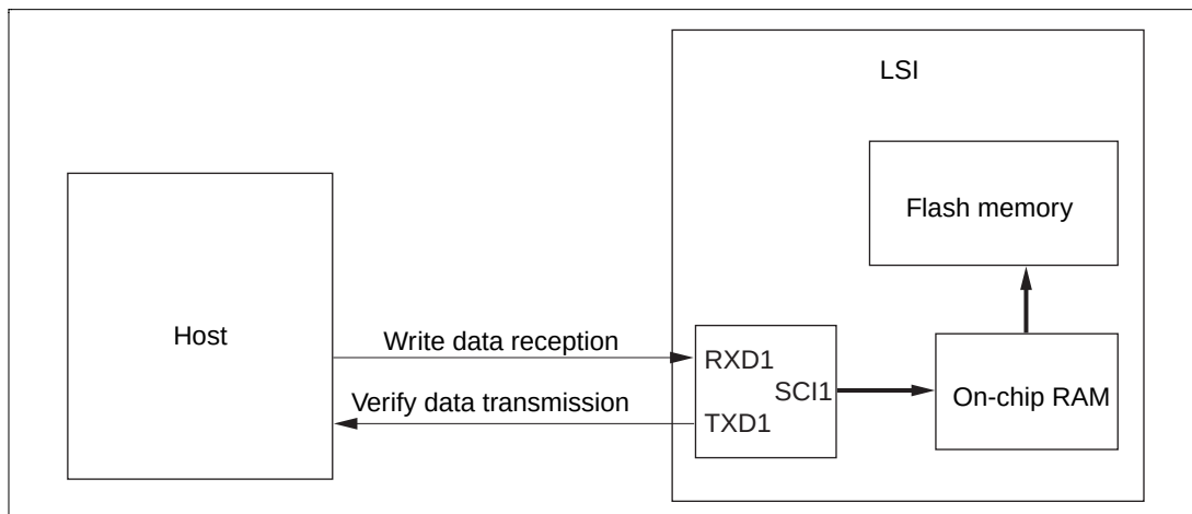
Figure 22.3 System Configuration in Boot Mode
