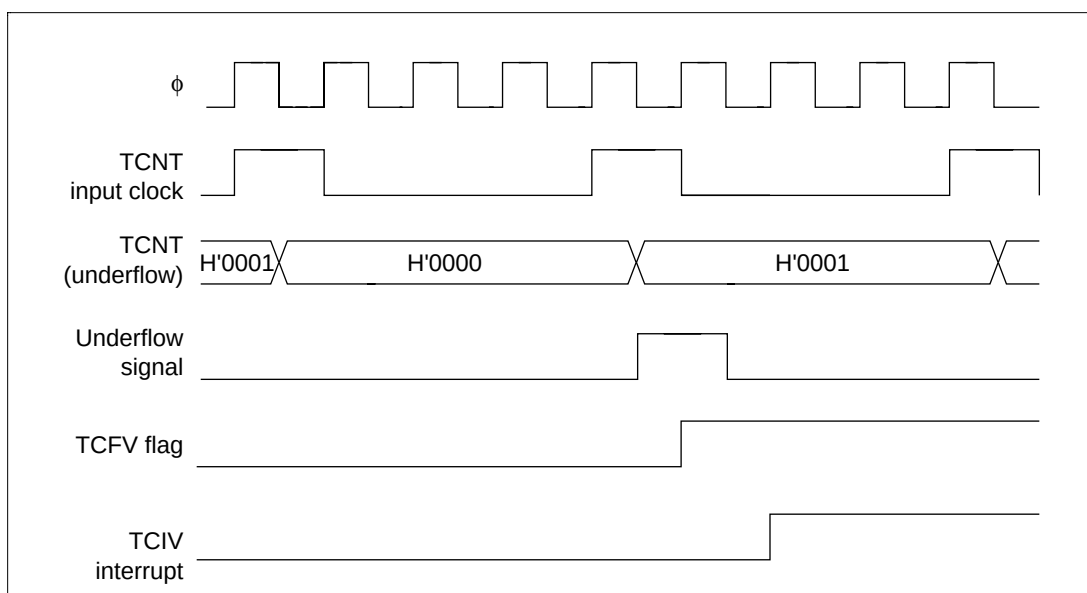
Figure 12.74 TCIV Interrupt Setting Timing (TSR4, Complementary PWM Mode)
