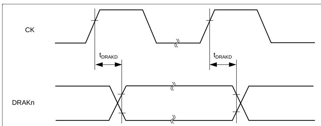
Figure 27.22 DRAK Output Delay Time
