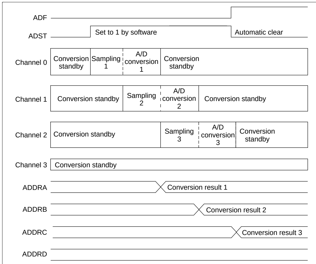
Figure 15.5 A/D Converter Operation Example (Group-Single Mode)
