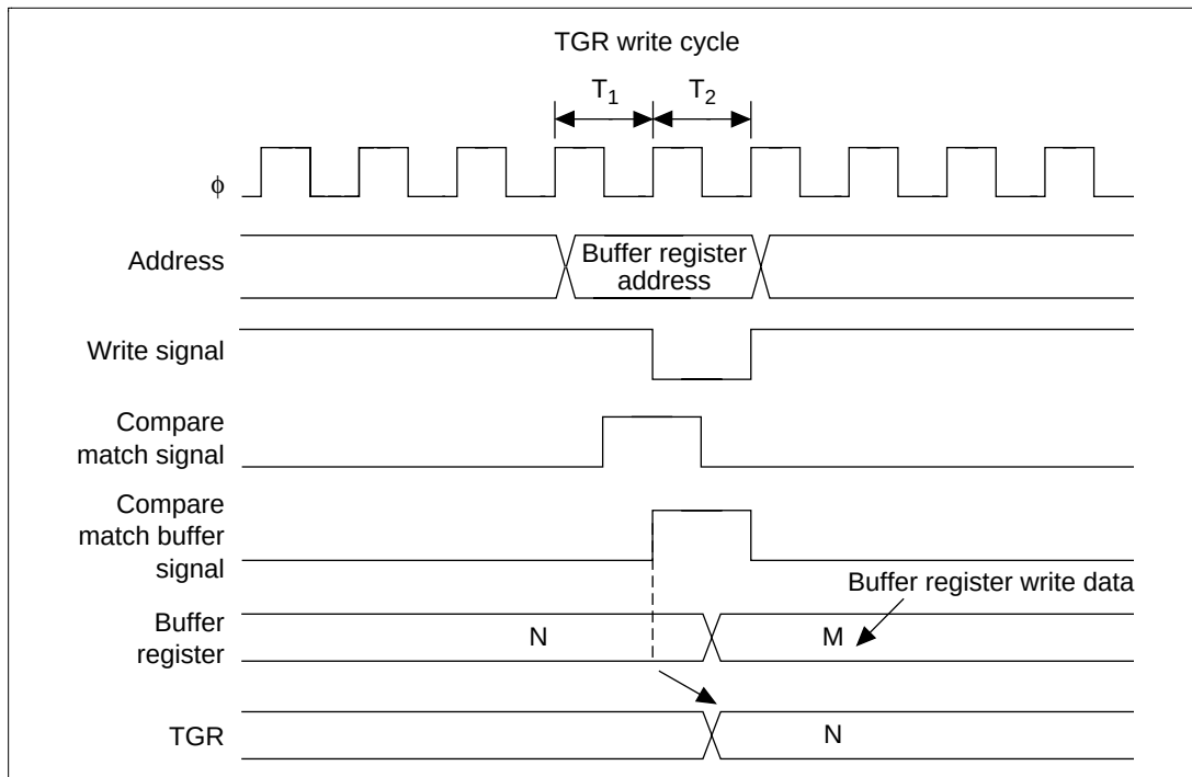
Figure 12.81 TGR Write and Compare-Match Contention (Channels 3 and 4)
