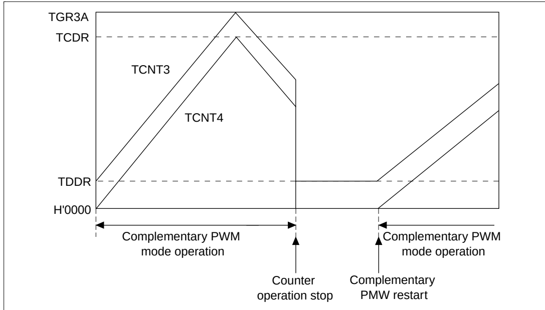
Figure 12.87 Counter Value during Complementary PWM Mode Stop
