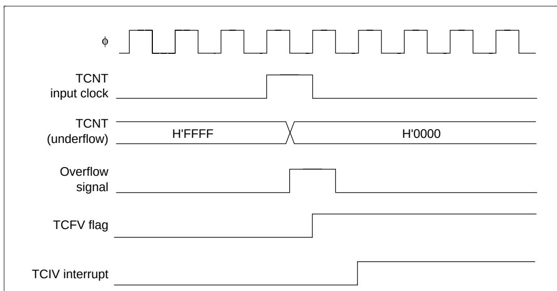
Figure 12.72 TCIV Interrupt Setting Timing
