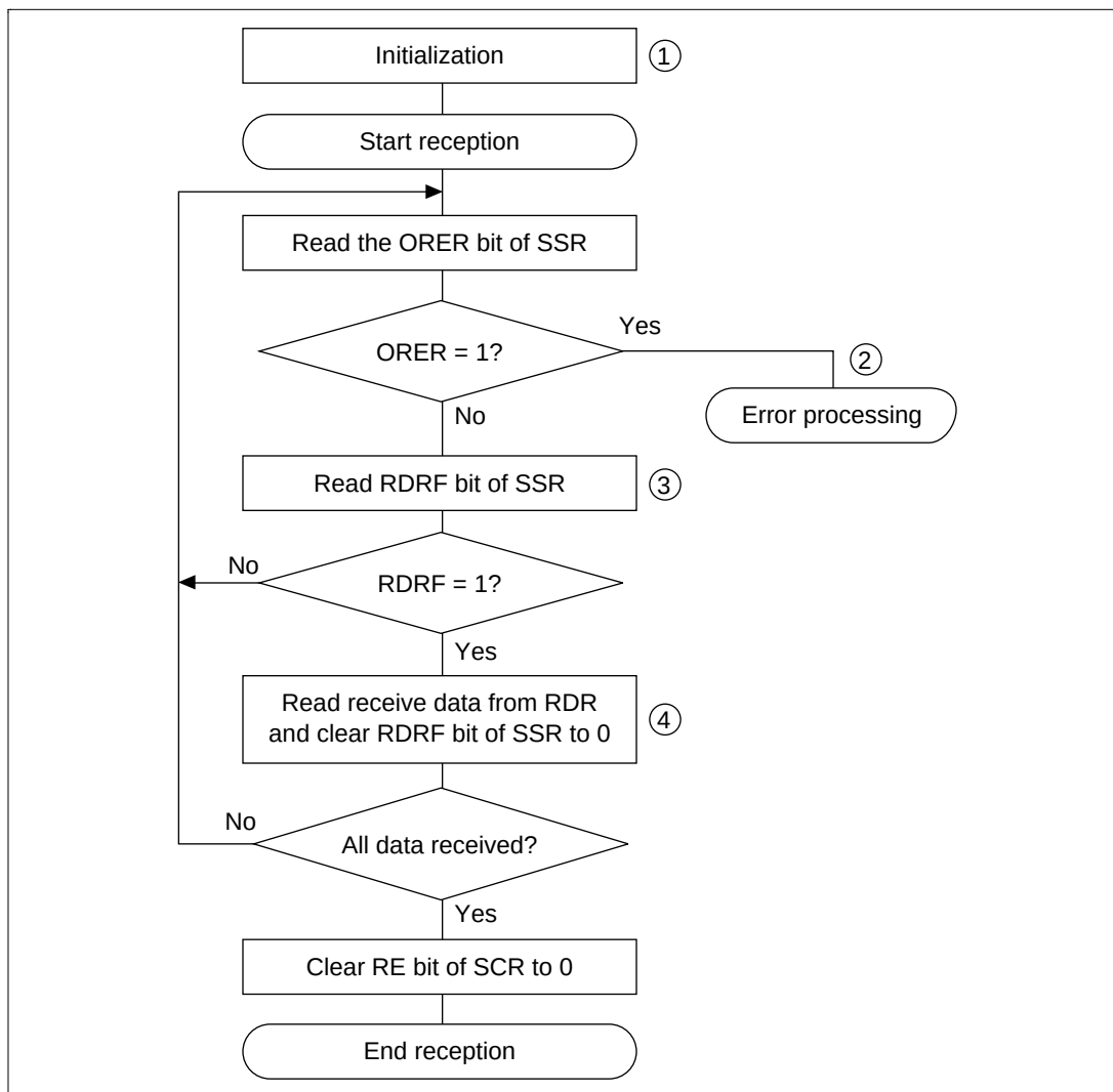
Figure 14.20 Sample Flowchart for Serial Receiving
