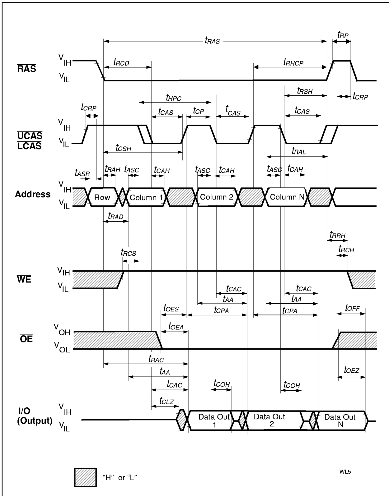
Hyper Page Mode (EDO) Read Cycle
