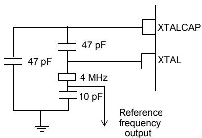
Figure 8 - Crystal oscillator application
