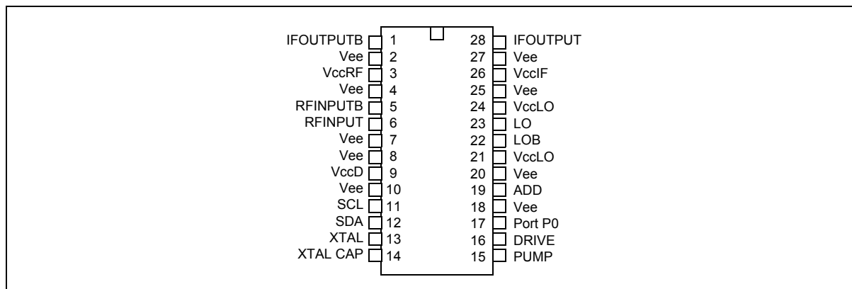
Figure 2 - Pin Description
