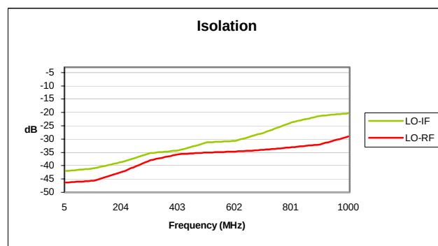
Typical Test Data – LO-RF and LO-IF Isolation
