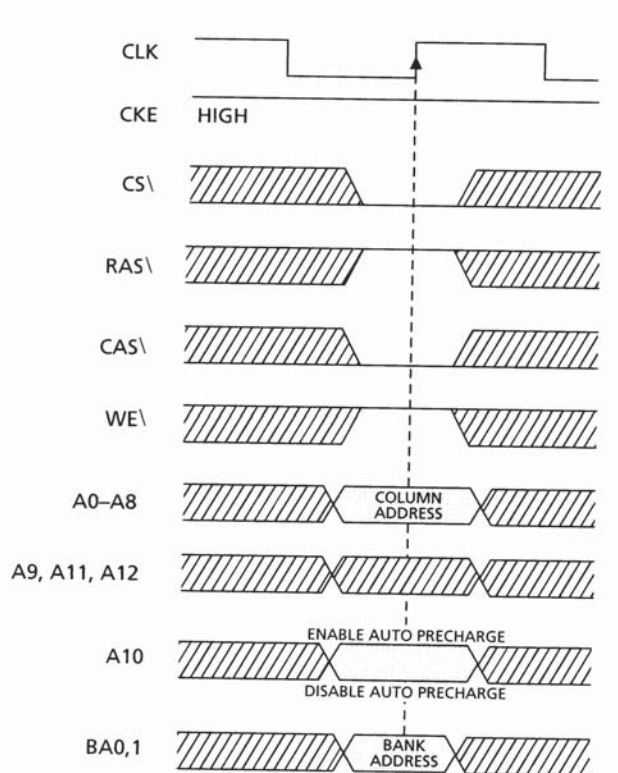
FIGURE 5: READ Command
