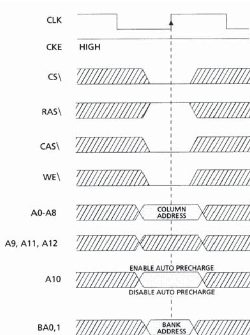
FIGURE 13: WRITE Command
