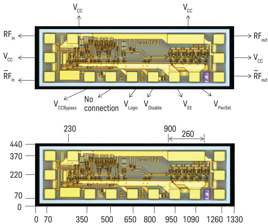
Figure 2. Pad locations and chip dimensions
