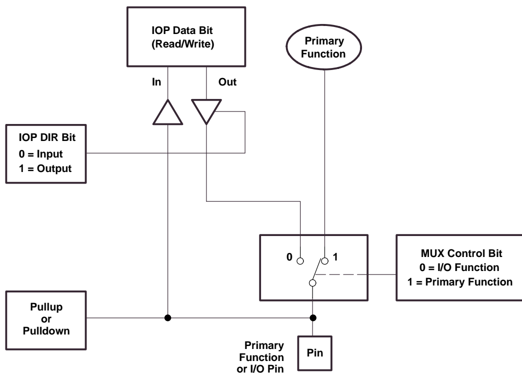
Figure 17. Shared Pin Configuration
