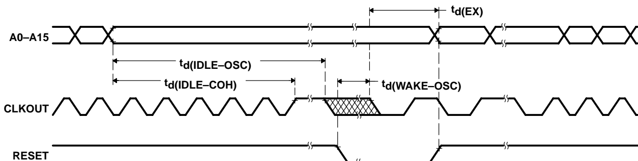
Figure 31. HALT Mode – LPM2
