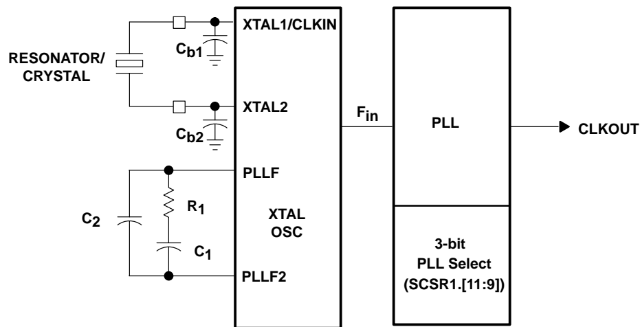
Figure 15. PLL Clock Module Block Diagram
