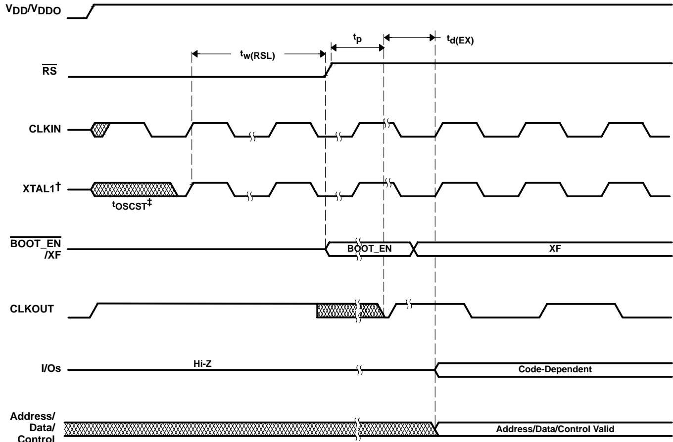
Figure 26. Power-on Reset
