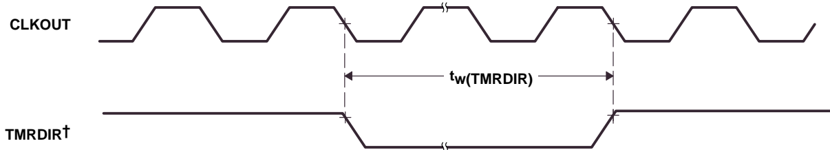
Figure 35. Capture/TMRDIR Timing
