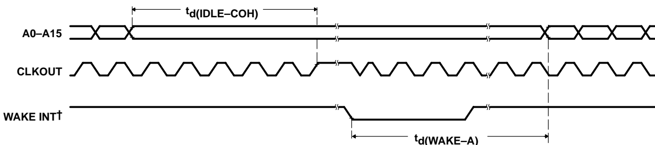
Figure 30. IDLE2 Entry and Exit Timing – LPM1
