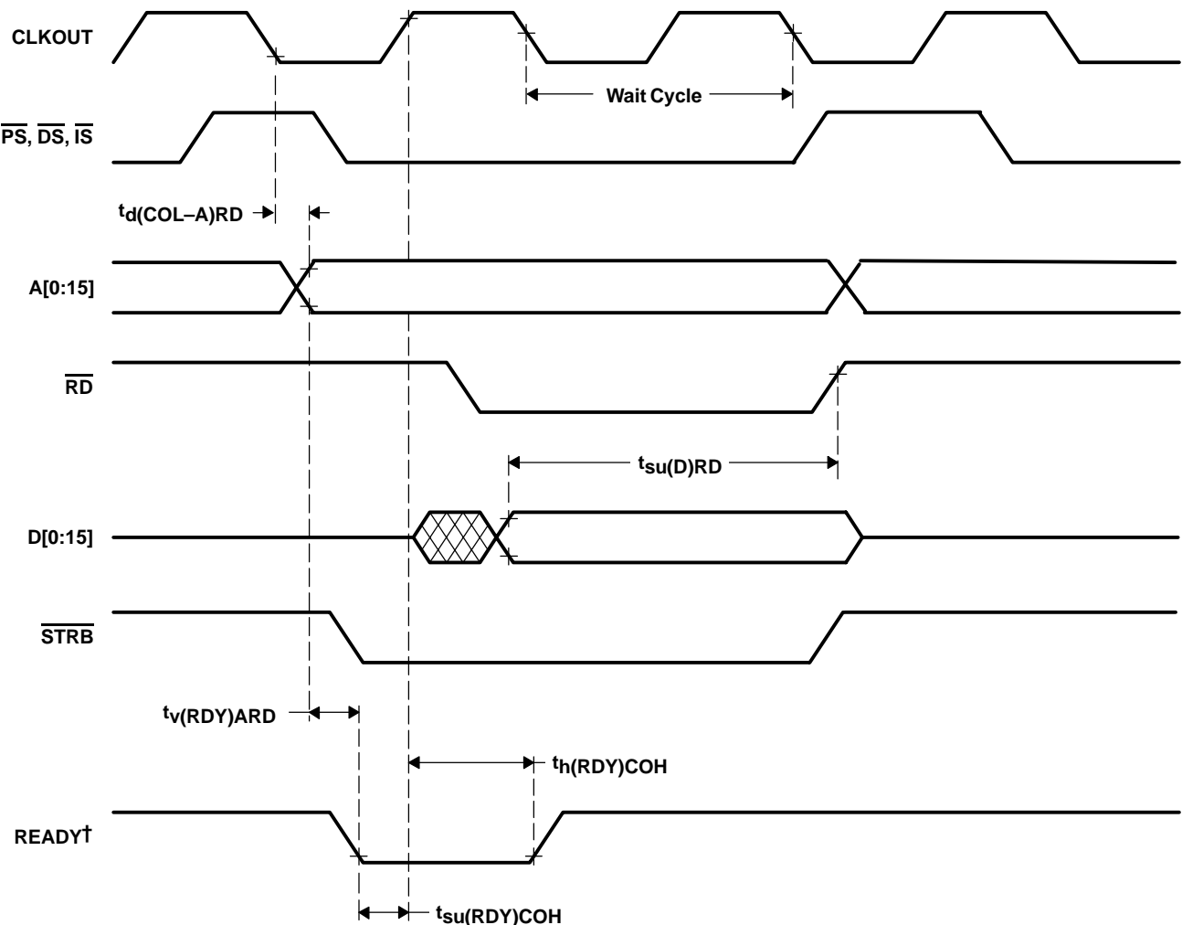
Figure 46. Ready-on-Read Timings
