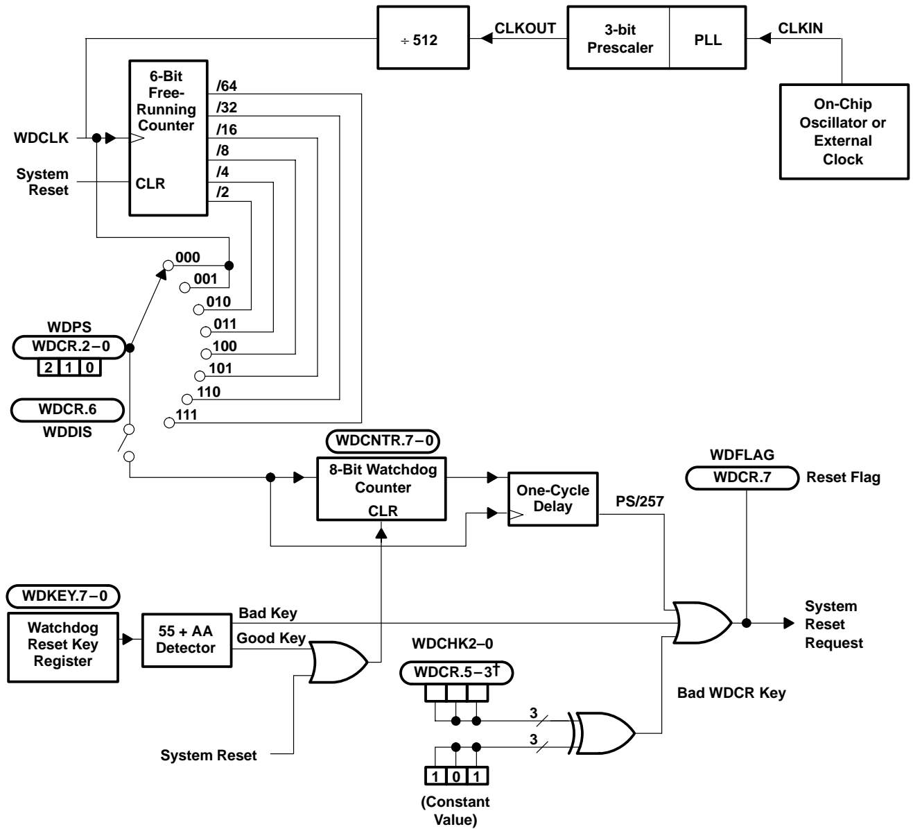
Figure 18. Block Diagram of the WD Module
