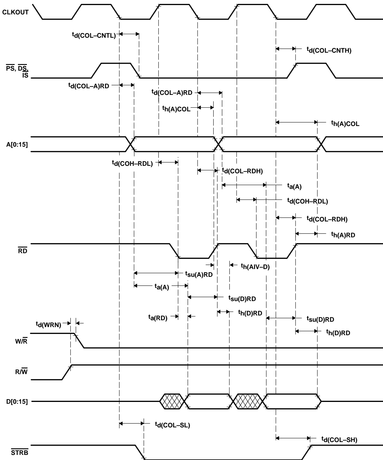
Figure 44. Memory Interface Read/Read Timings
