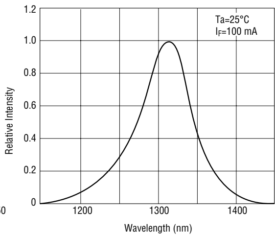
Emission Spectrum
