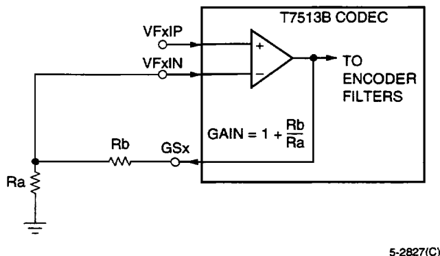
Figure 4. Analog Inputs
