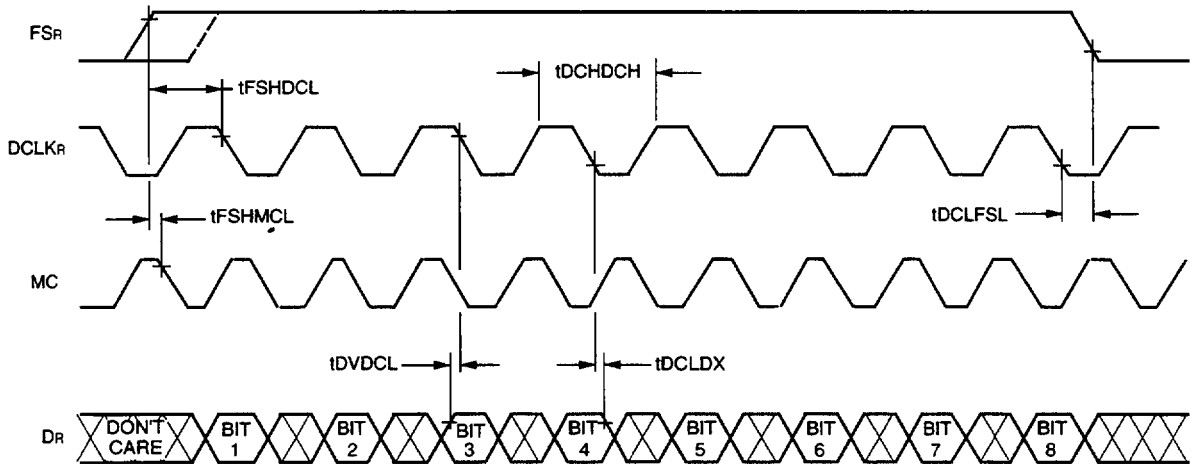
Figure 10. Variable-Data-Rate Transmit Timing
