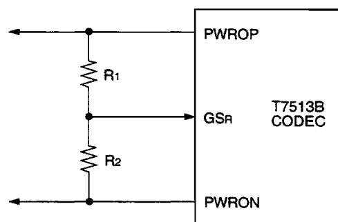
Figure 5. Analog Outputs
