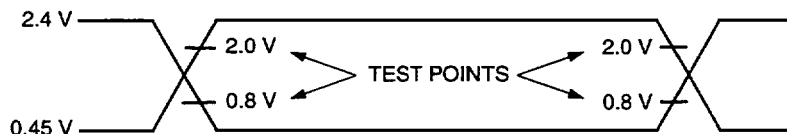
Figure 11. Variable-Data-Rate Receive Timing
