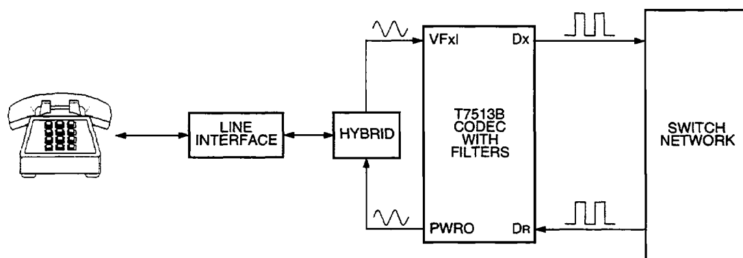
Figure 3. PCM System Block Diagram
