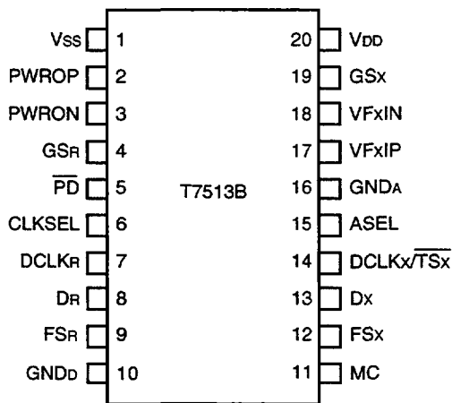
Figure 2. Pin Diagram
