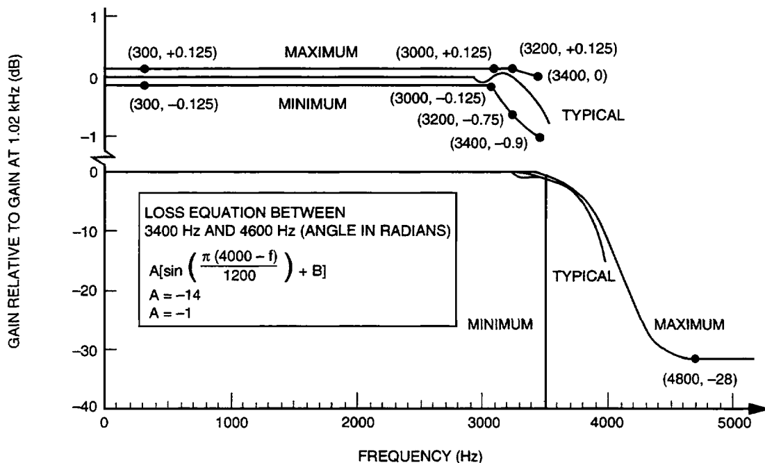
Figure 6. Receive Filter Characteristics
