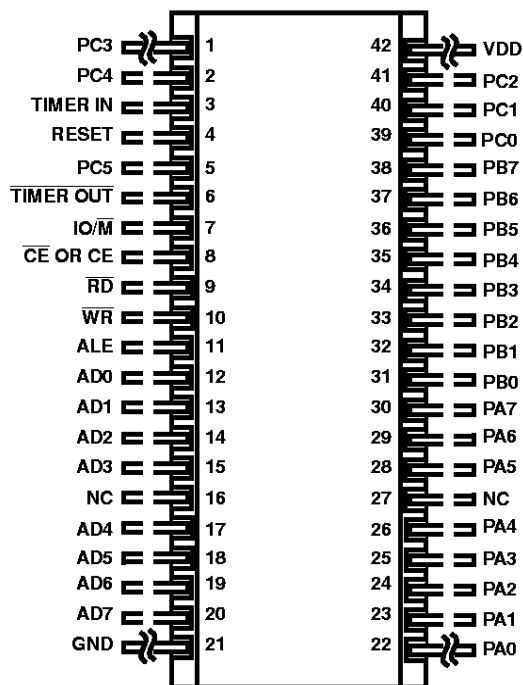
42 LEAD CERAMIC METAL SEAL FLATPACK PACKAGE HARRIS OUTLINE K42.A TOP VIEW
