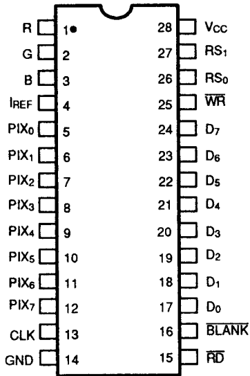
28-PIN DIP
