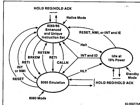
Figure 7. V30 Modes
