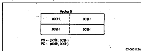
Figure 9. Interrupt Vector 0
