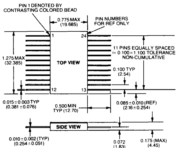
FIGURE 9. BUS-63106II, BUS-63108II, BUS-63116II, AND BUS-63118II MECHANICAL OUTLINE-24PIN FLATPACK
