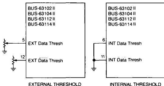
FIGURE 5. THRESHOLD CONNECTIONS
