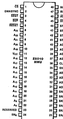
Figure 2. 48-pin Dual-In-Line Package (DIP), Pin Assignments
