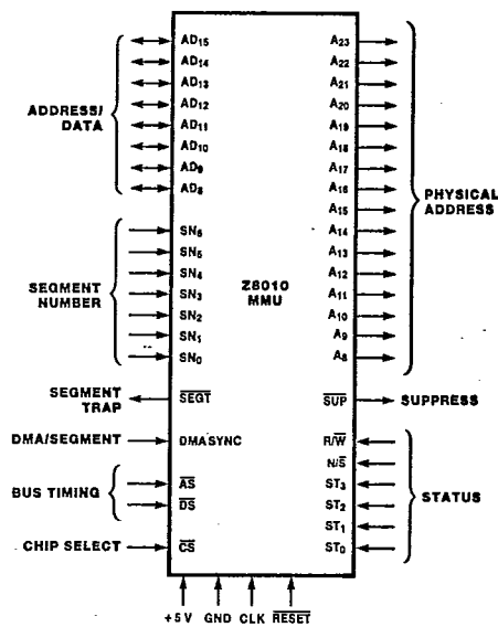
Figure 1. Pin Functions
