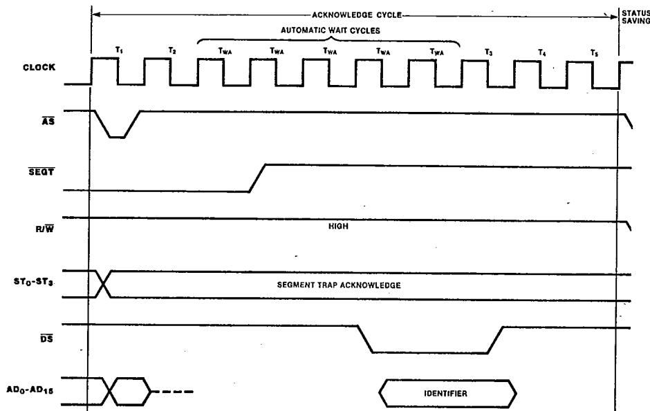
Figure 12. Segment Trap and Acknowledge Timing
