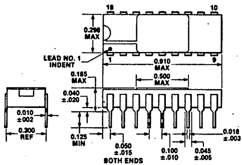
18-Pin Ceramic Package
