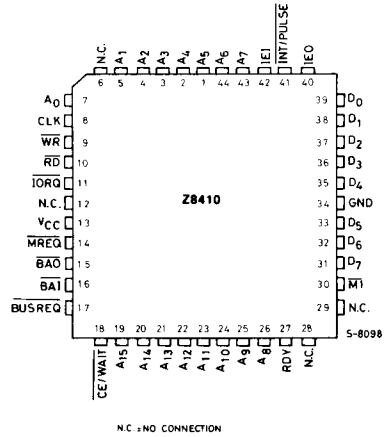
Figure 2a. Chip Carrier Pin Configuration
