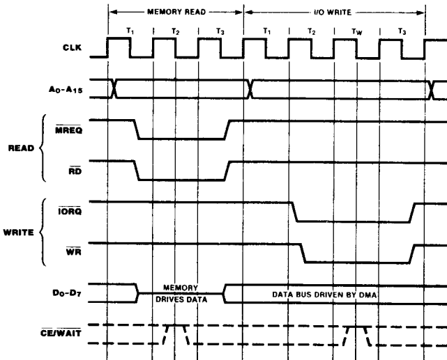
Figure 12. Memory-to-I/O Transfer
