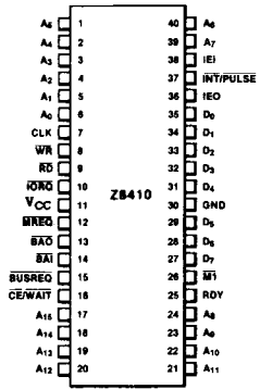
Figure 2. Pin Configuration
