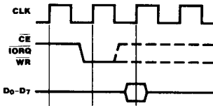
Figure 10. CPU-to-DMA Write Cycle
