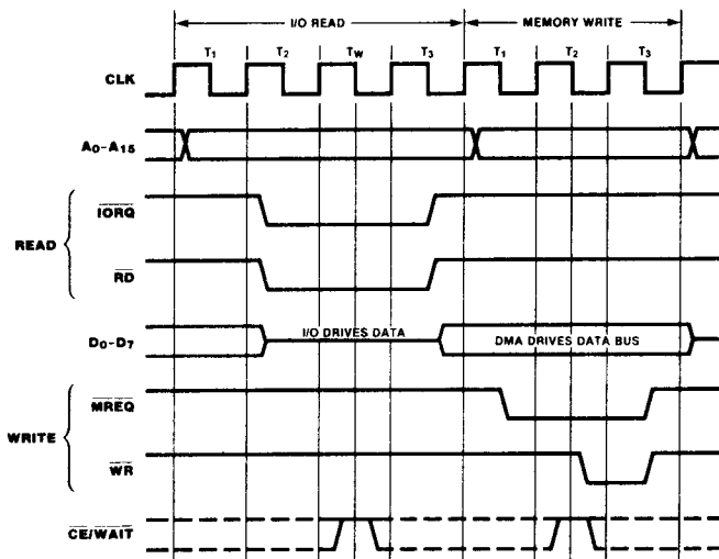
Figure 13. I/O-to-Memory Transfer
