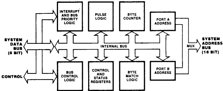
Figure 6. Block Diagram
