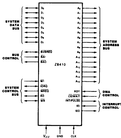
Figure 1. Logic Functions
