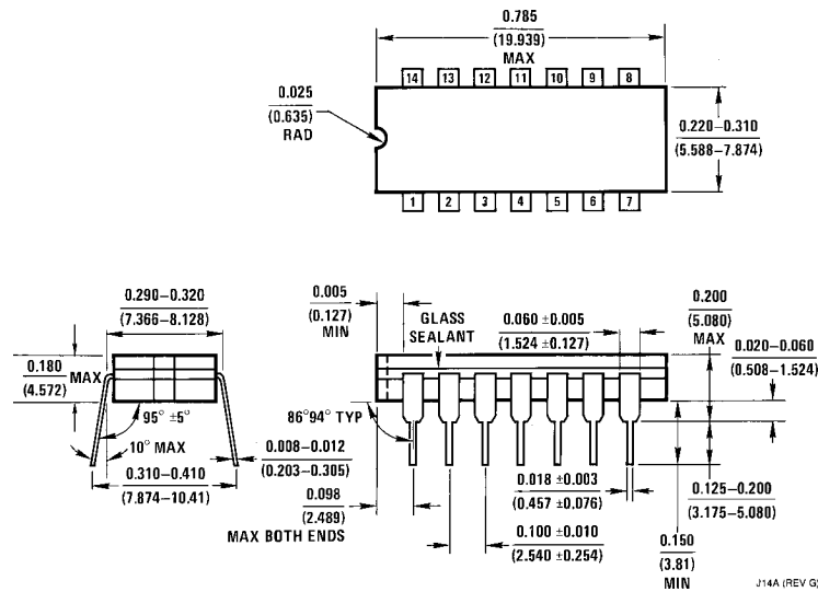
14-Lead Ceramic Dual-In-Line Package (J) Order Number 9601DMQB or DM9601J NS Package Number J14A
