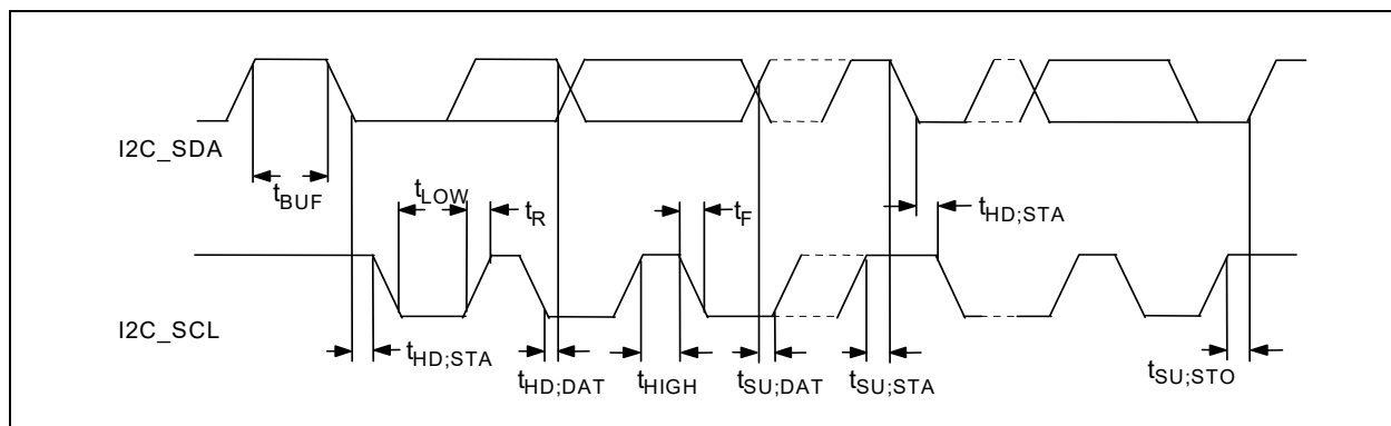
FIGURE 50-15: I2C/SMBUS TIMING
