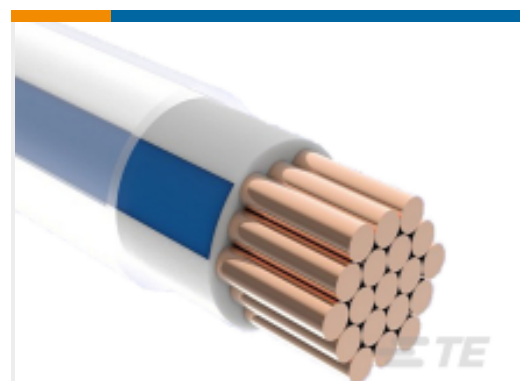
TE Model / Part #9623083001 ACW0219-1.50-0(NS)
