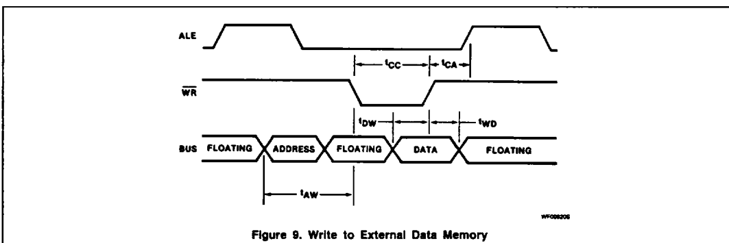
Figure 9. Write to External Data Memory
