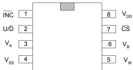
8-MSOP
