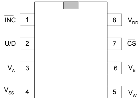
8-SOIC
