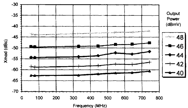
XMOD VS. FREQUENCY 110 CHANNEL LOADING, FLAT
