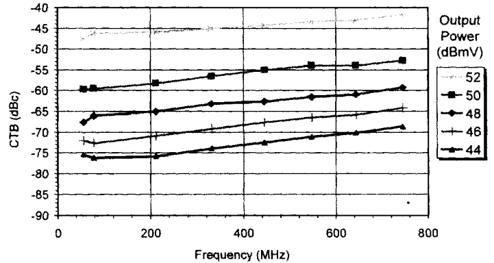
CTB VS. FREQUENCY 110 CHANNEL LOADING, FLAT
