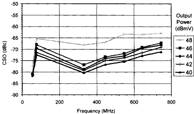
CSO VS. FREQUENCY 110 CHANNEL LOADING, FLAT
