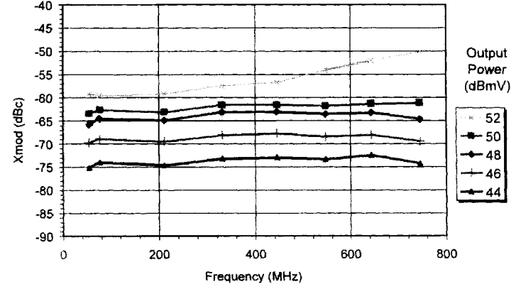
XMOD VS. FREQUENCY 110 CHANNEL LOADING, FLAT
