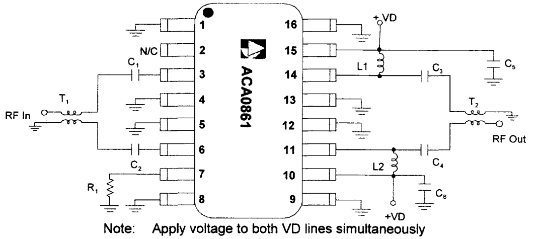
Figure 1. Test Circuit
