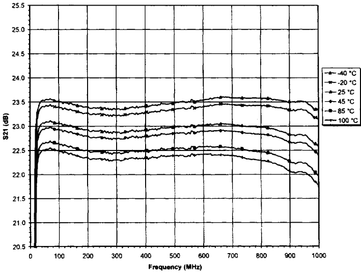
GAIN / S21
