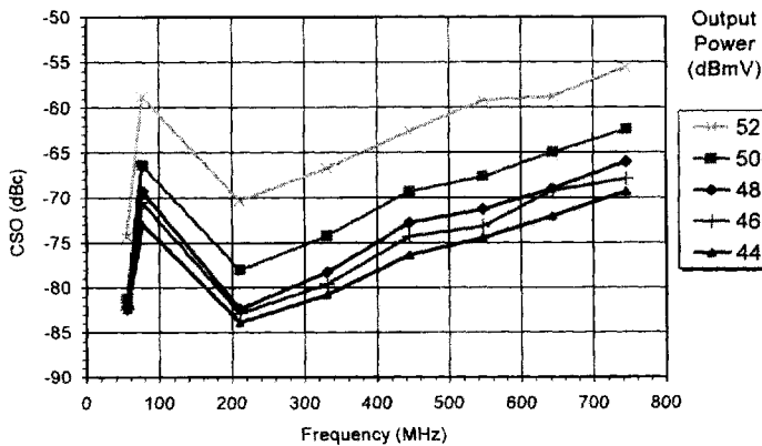
CSO VS. FREQUENCY 110 CHANNEL LOADING, FLAT
