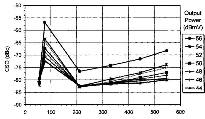
CSO VS. FREQUENCY 77 CHANNEL LOADING, 8 dB TILT
