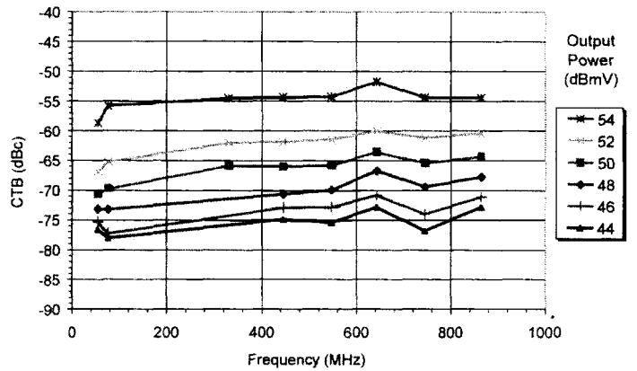
CTB VS. FREQUENCY 128 CHANNEL LOADING, 12dB TILT
