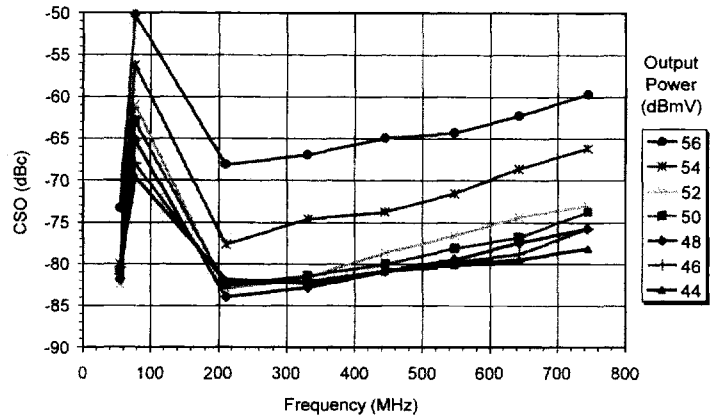
CSO VS. FREQUENCY 110 CHANNEL LOADING, 10dB TILT
