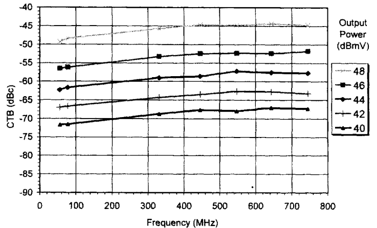
CTB VS. FREQUENCY 110 CHANNEL LOADING, FLAT
