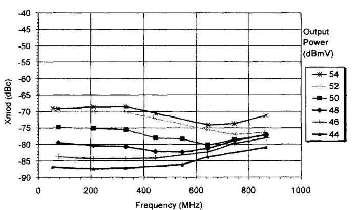
XMOD VS. FREQUENCY 128 CHANNEL LOADING, 12dB TILT
