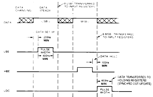
FIGURE 5 Two-Byte Loading
