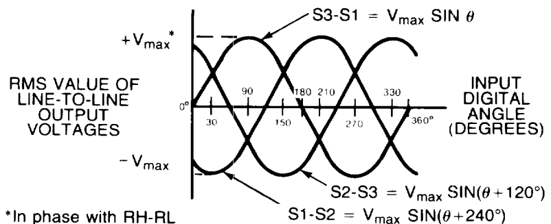
FIGURE 12 Synchro Outputs
