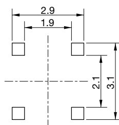
Refer-1 Bottom soldering
