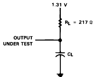
FIGURE 1. LOAD CIRCUIT
