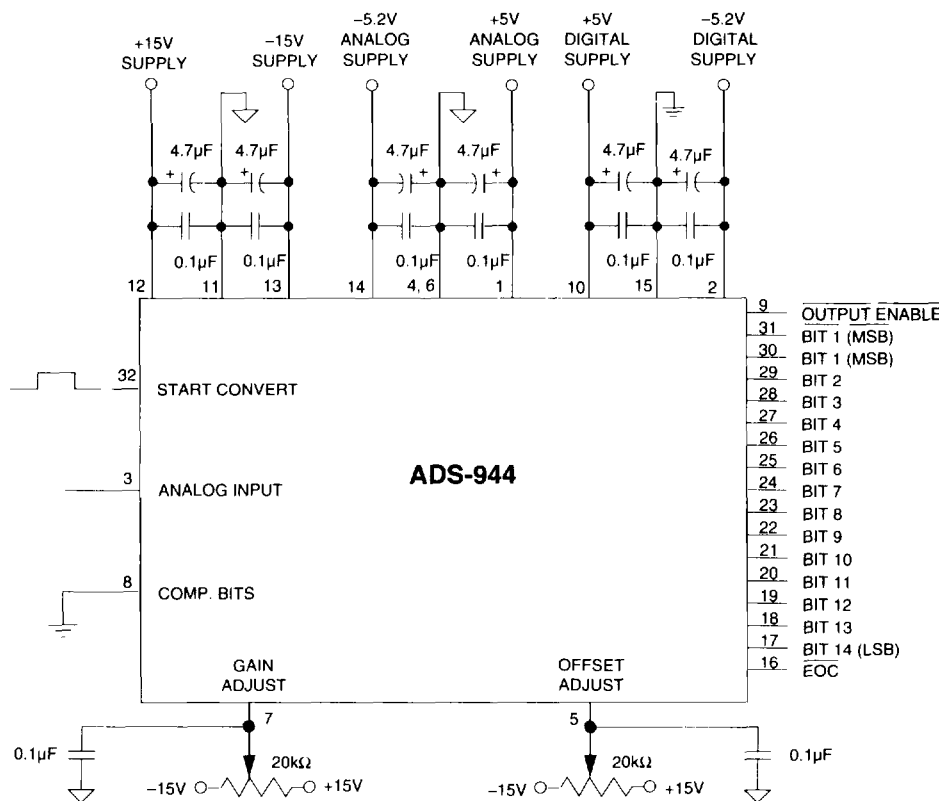
Figure 2. ADS-944 Connection Diagram
