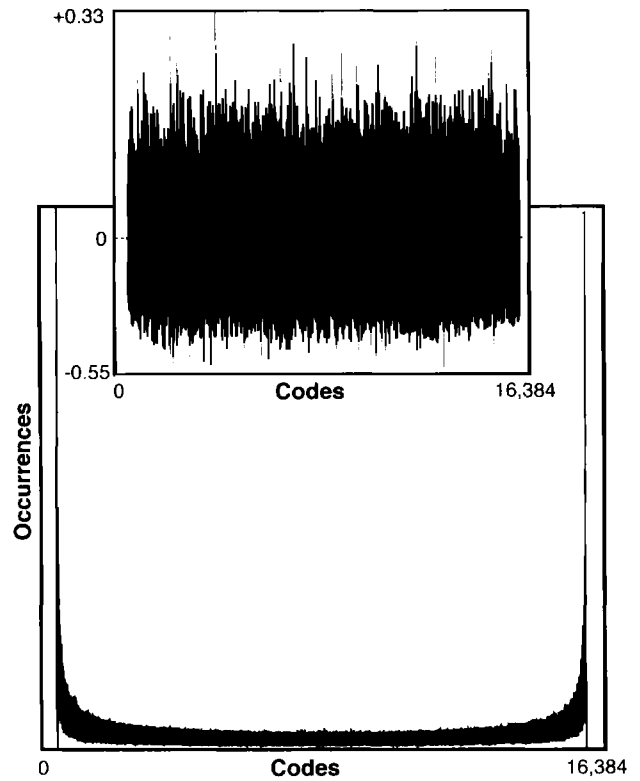
Figure 7. ADS-944 Histogram and Differential Nonlinearity
