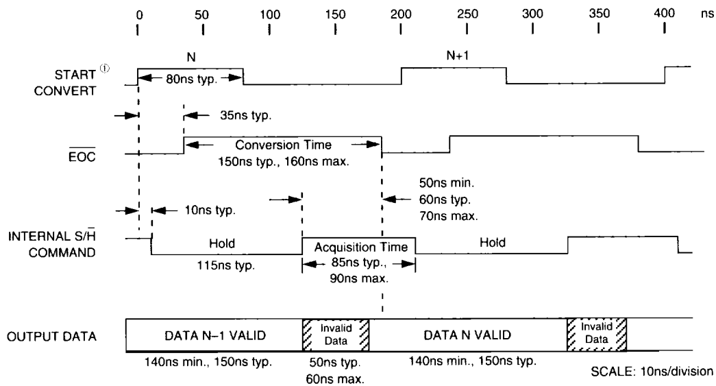
① START CONVERT pulse width: 40 to 80ns or 130 to 160ns
