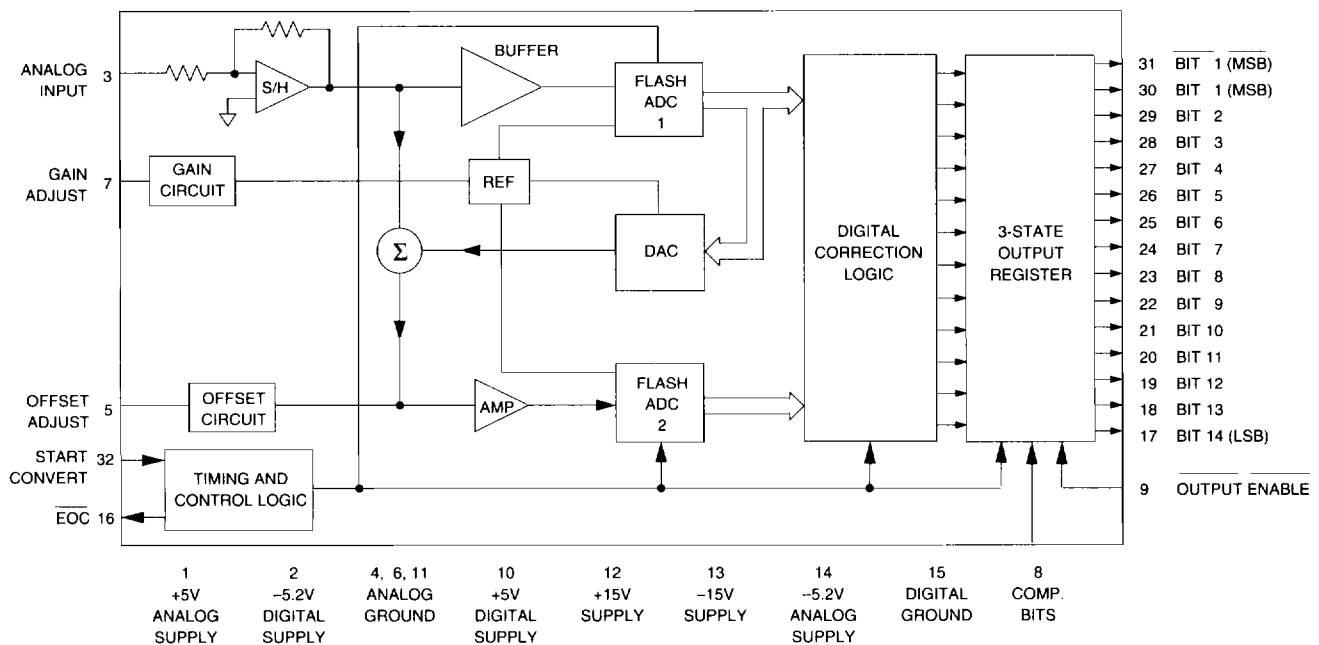
Figure 1. ADS-944 Functional Block Diagram
