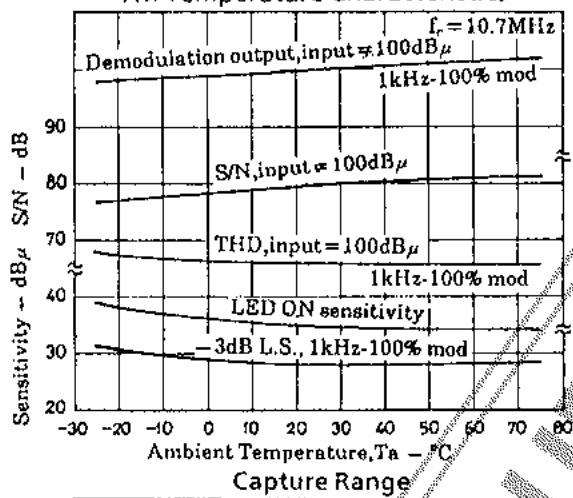
FM Temperature Characteristics
