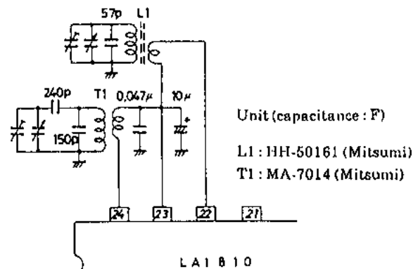
LW Band Test Circuit
