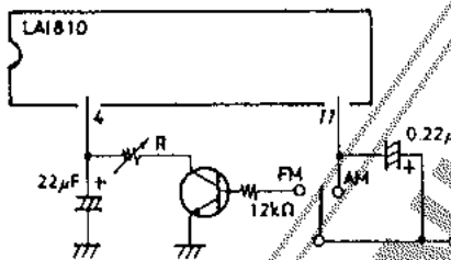
Fig.1 Method to Change the LED ON Sensitivity at the FM Mode
