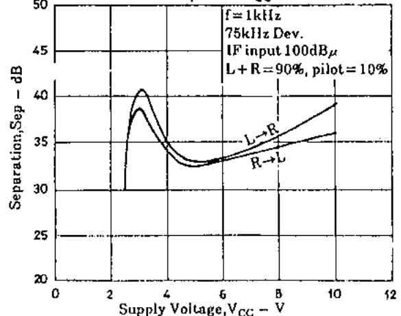
Sep - V CC
