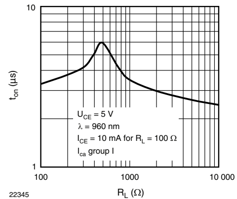
Fig. 2 - Turn-on Time vs. Load Resistance
