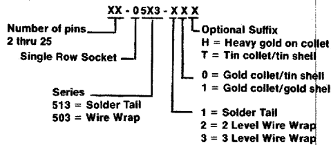
PIN-LINE Collet Contacts with "Break" Feature 2 to 25 positions
