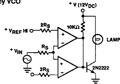
Limit Comparator
