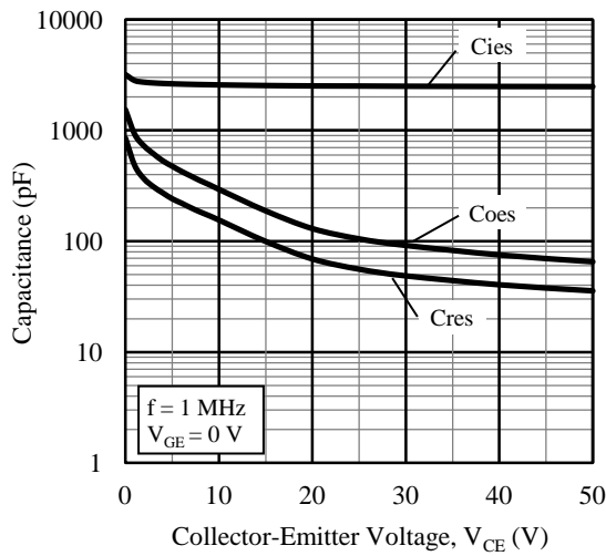
Figure 11. Capacitance Characteristics
