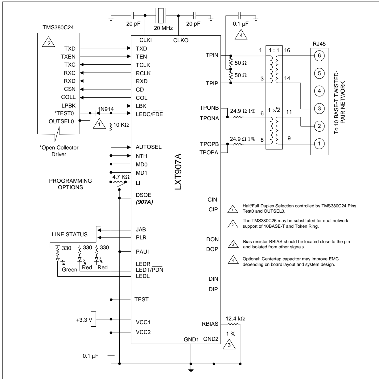
Figure 10. Full-Duplex Operation
