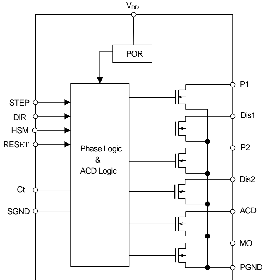
Fig.2 Block Diagram
