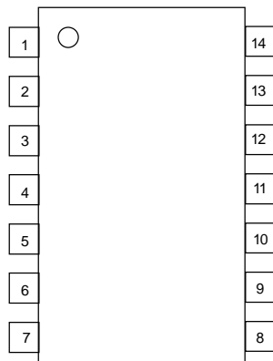
Fig. 1Pin Configurations
