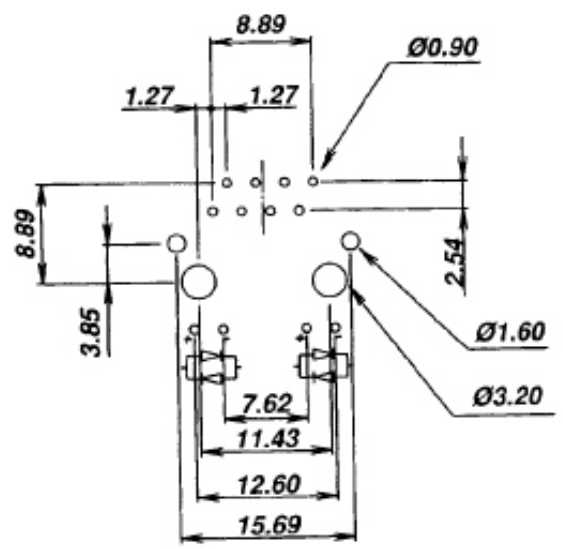
PCB LAYOUT
