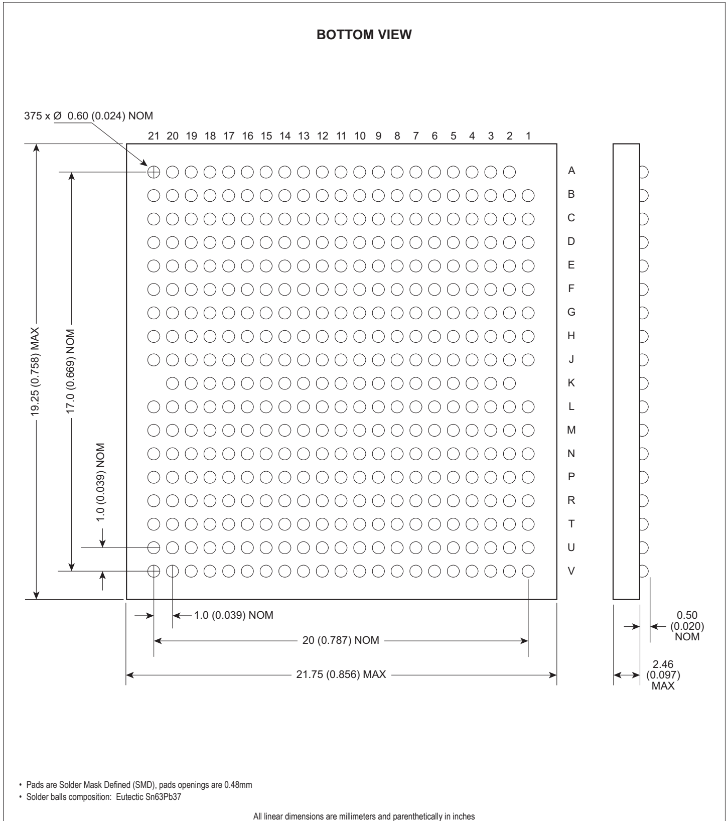
FIGURE 16 – PACKAGE DIMENSION: 375 PLASTIC BALL GRID ARRAY (PBGA) FOR W3J128M64G-XLBX
