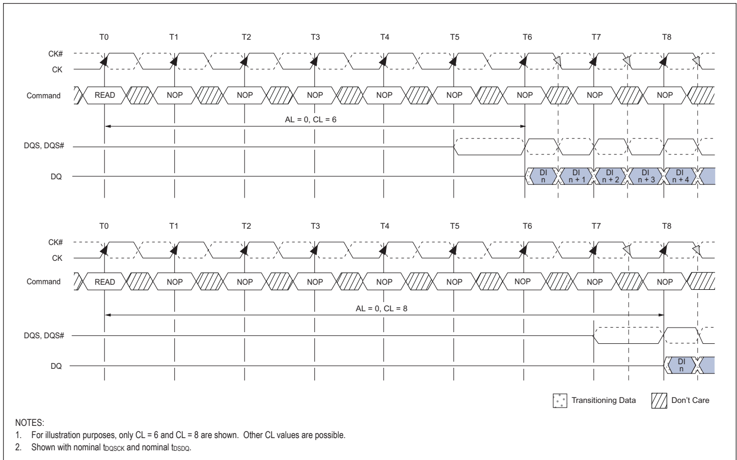
FIGURE 7 – READ LATENCY
