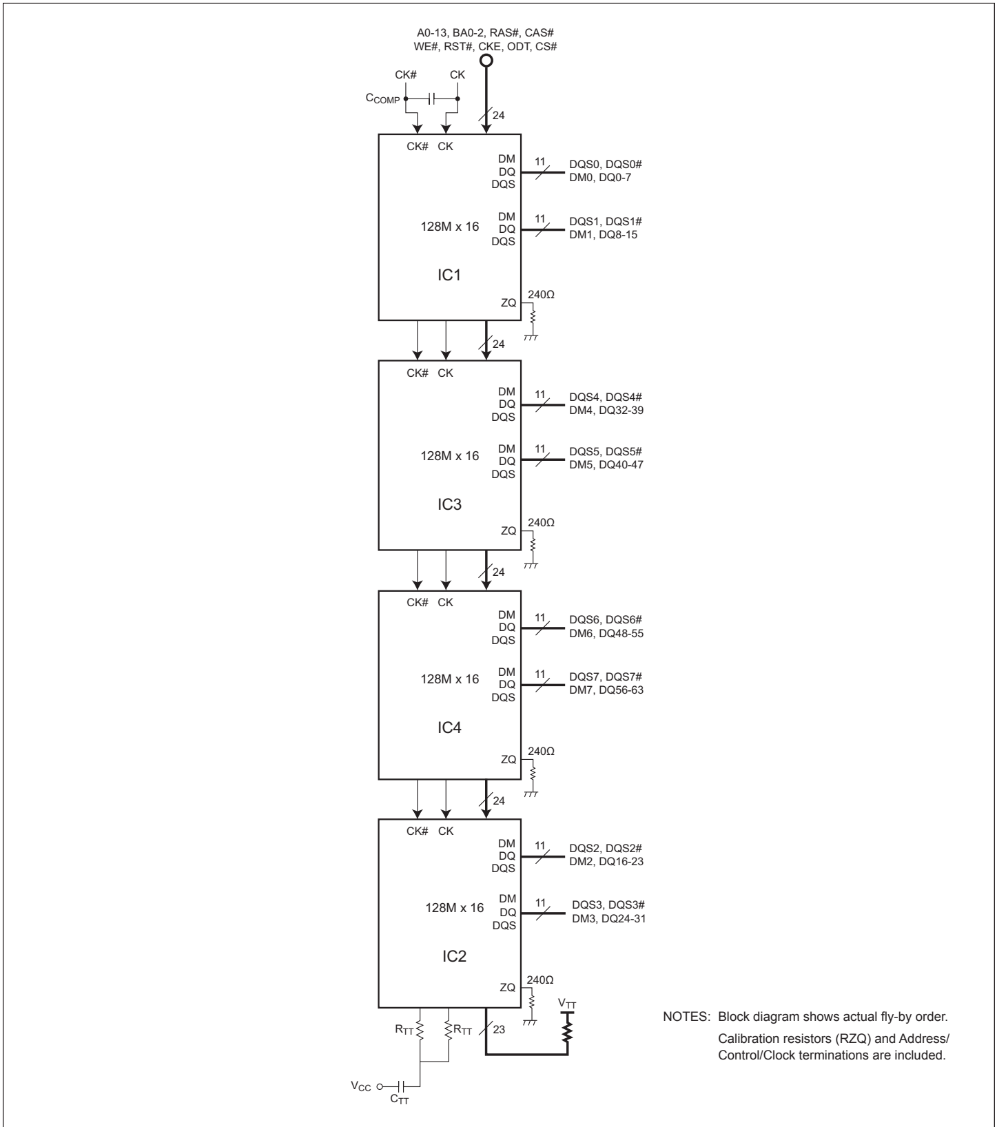
FIGURE 2 – FUNCTIONAL BLOCK DIAGRAM FOR W3J128M64G-XLBX
