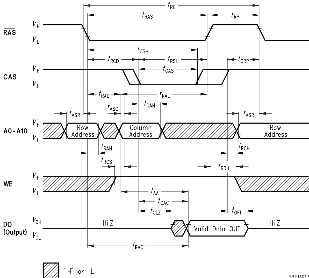
Read Cycle
