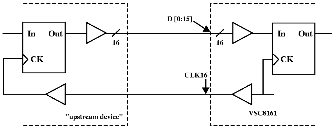
Figure 1: VSC8161 Parallel Data Interface
