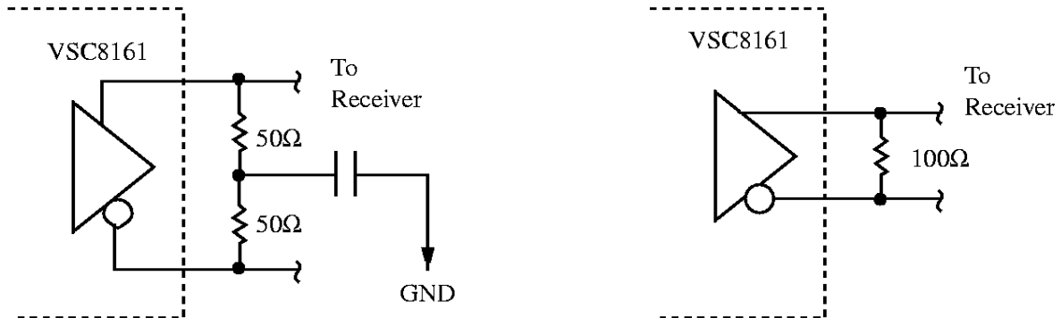
Figure 7: Differential Output Termination Methods
