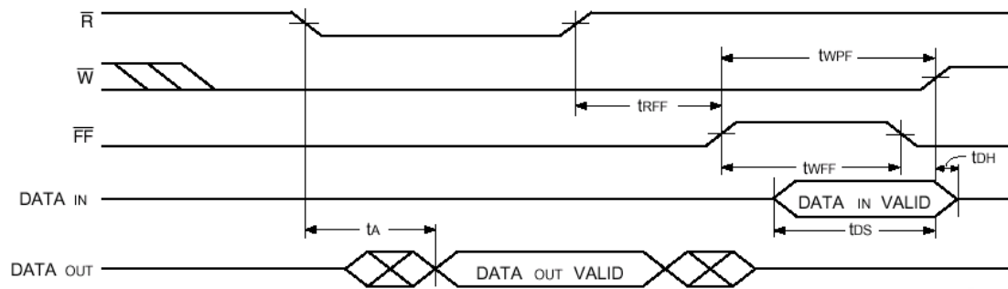
FIGURE 12. WRITE DATA FLOW FOR THROUGH MODE
