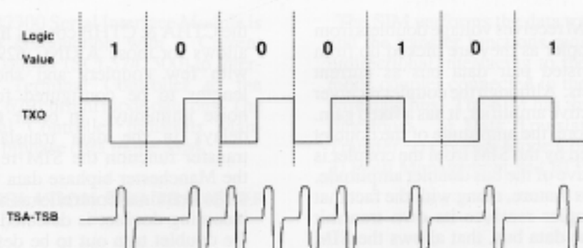
Figure 5. SIM Doublet Signaling
