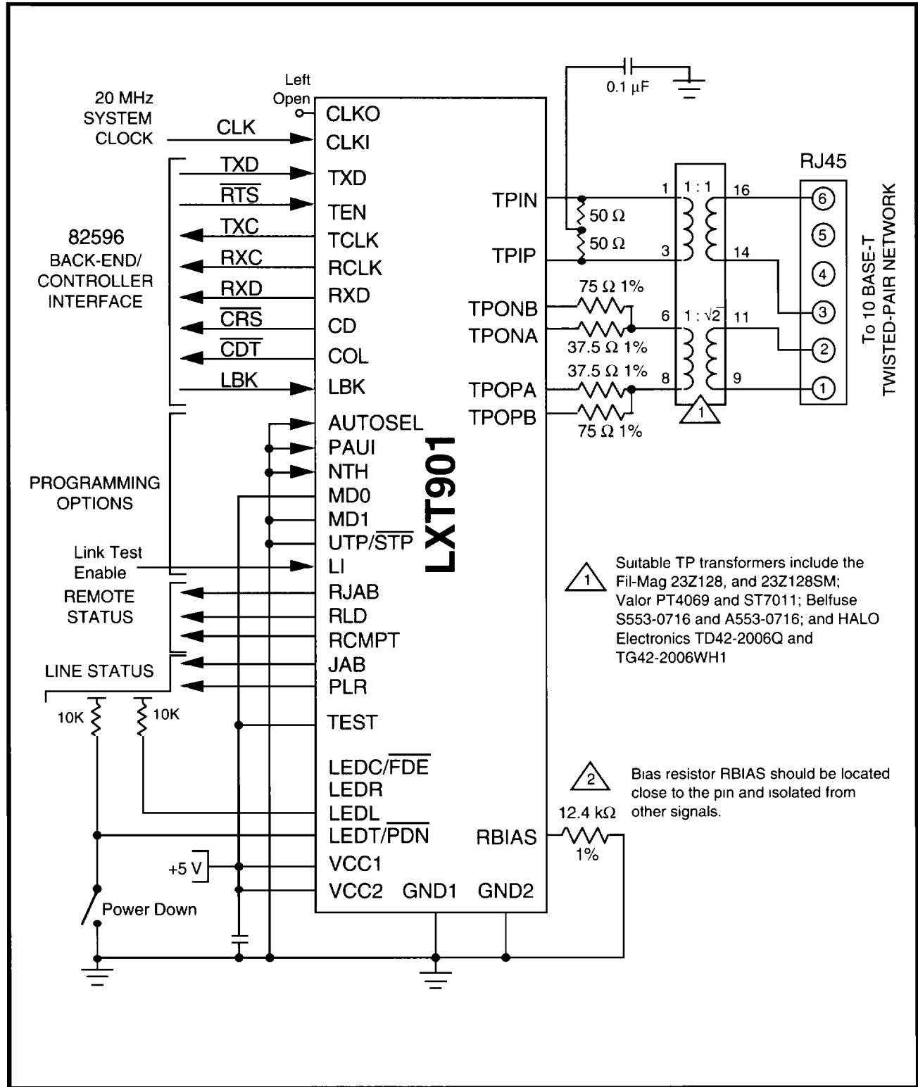
Figure 12: 150 Ω Shielded Twisted-Pair Only Application
