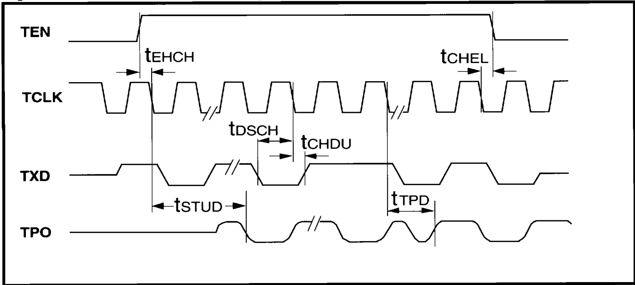
Figure 30: Mode 3 Transmit Timing
