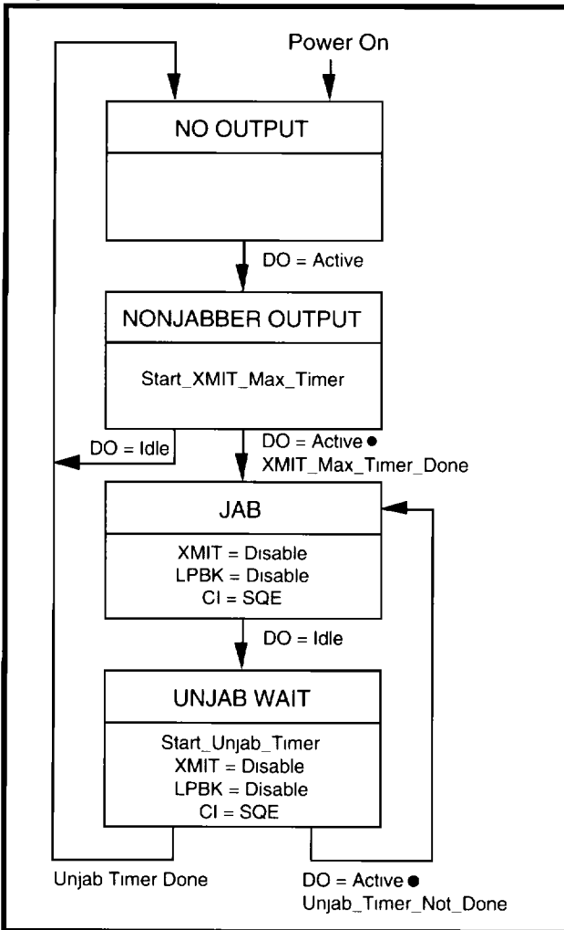
Figure 3: Jabber Control Function
