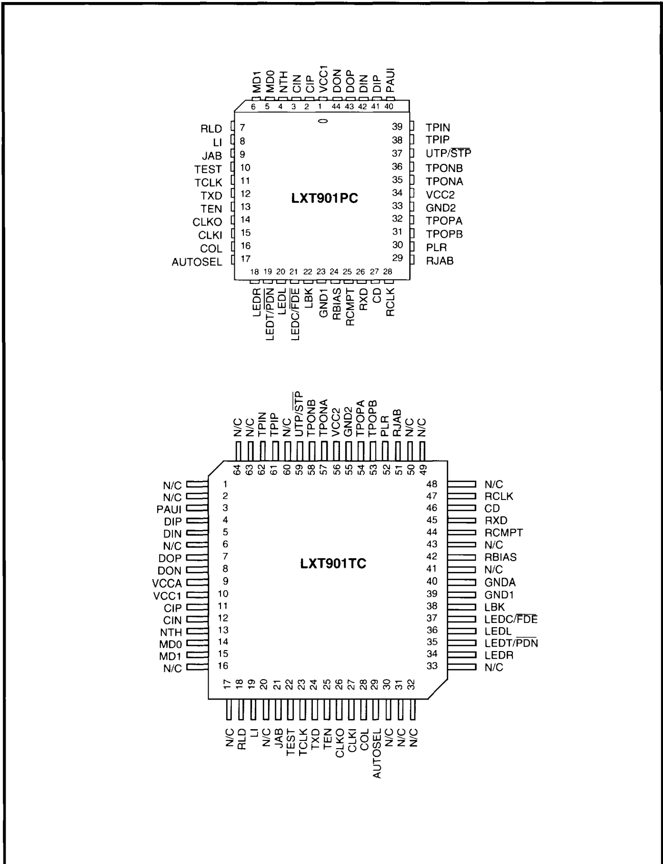
Figure 1: LXT901 Pin Assignments
