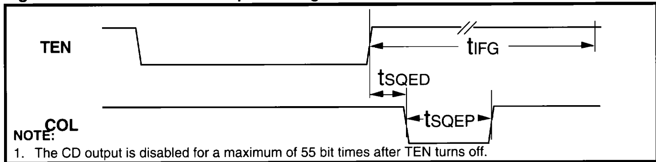
Figure 26: Mode 2 COL/CI Output Timing
