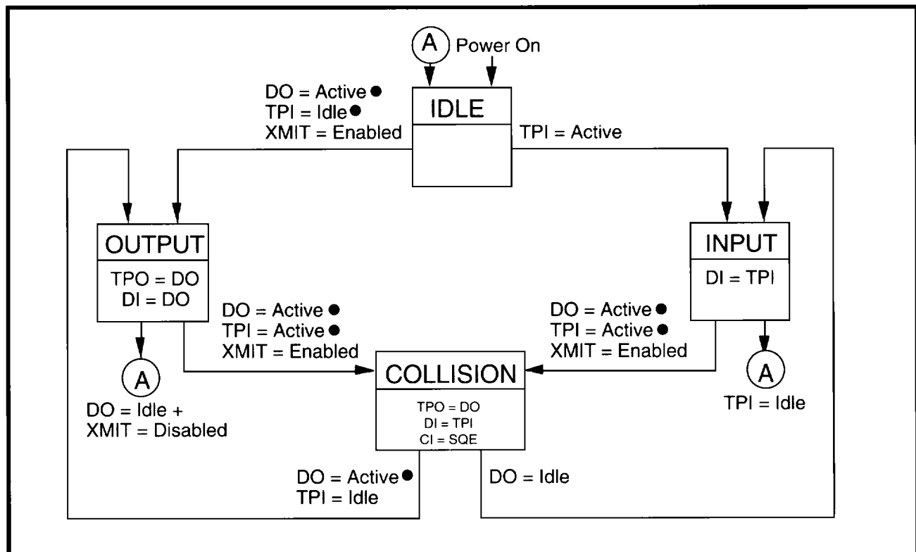
Figure 5: Collision Detection Function
