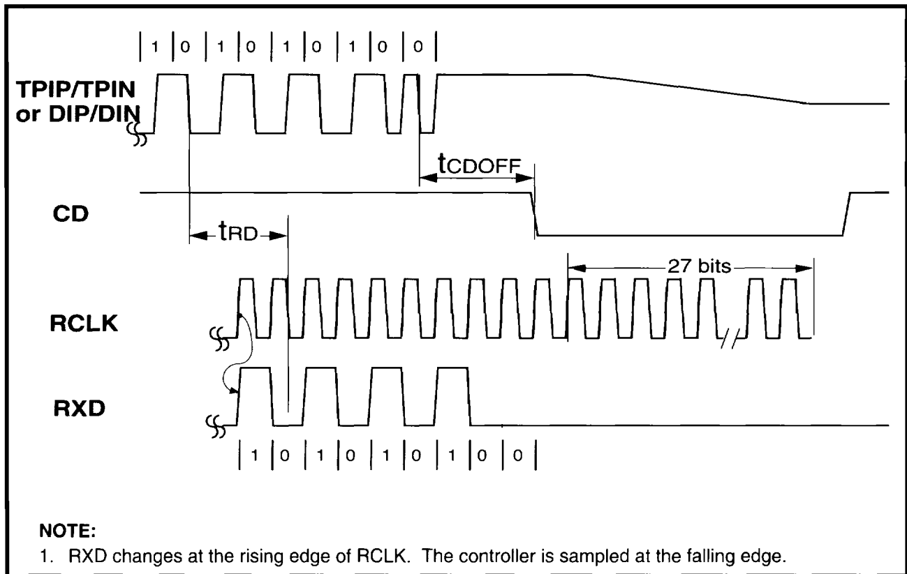
Figure 29: Mode 3 RCLK/End-of-Frame Timing
