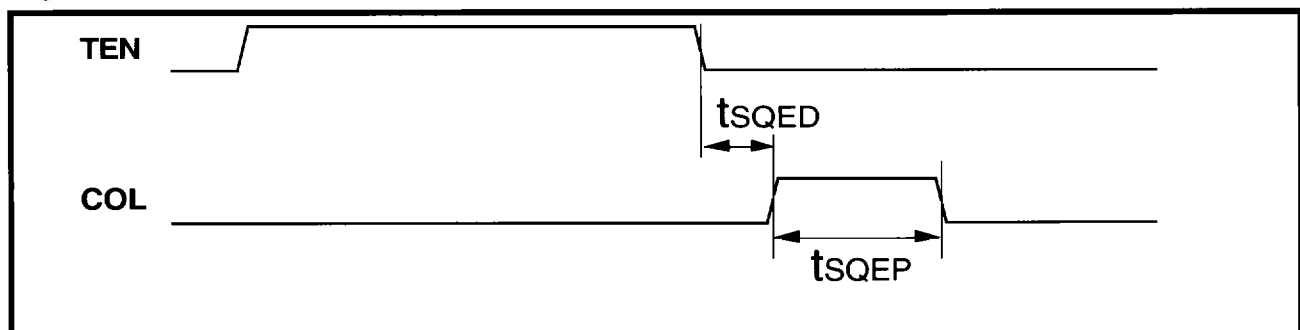
Figure 21: Mode 1 Loopback Timing
