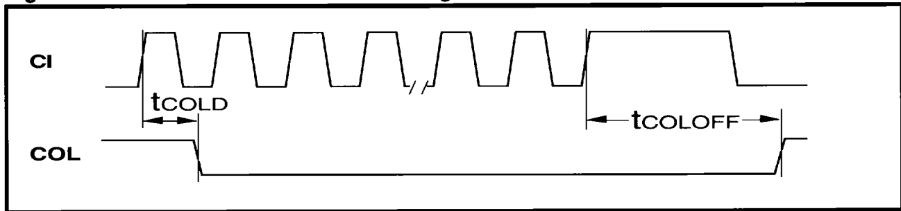
Figure 31: Mode 3 Collision Detect Timing
