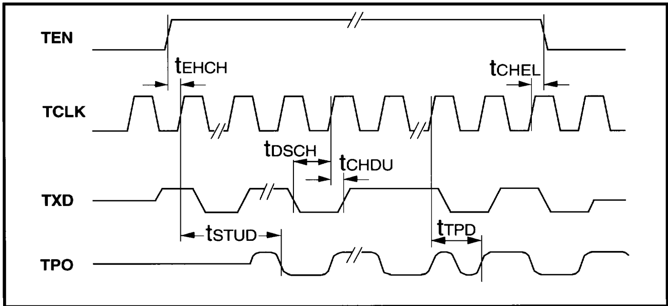
Figure 18: Mode 1 Transmit Timing
