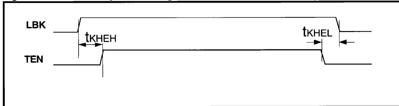
Figure 21: Mode 1 Loopback Timing
