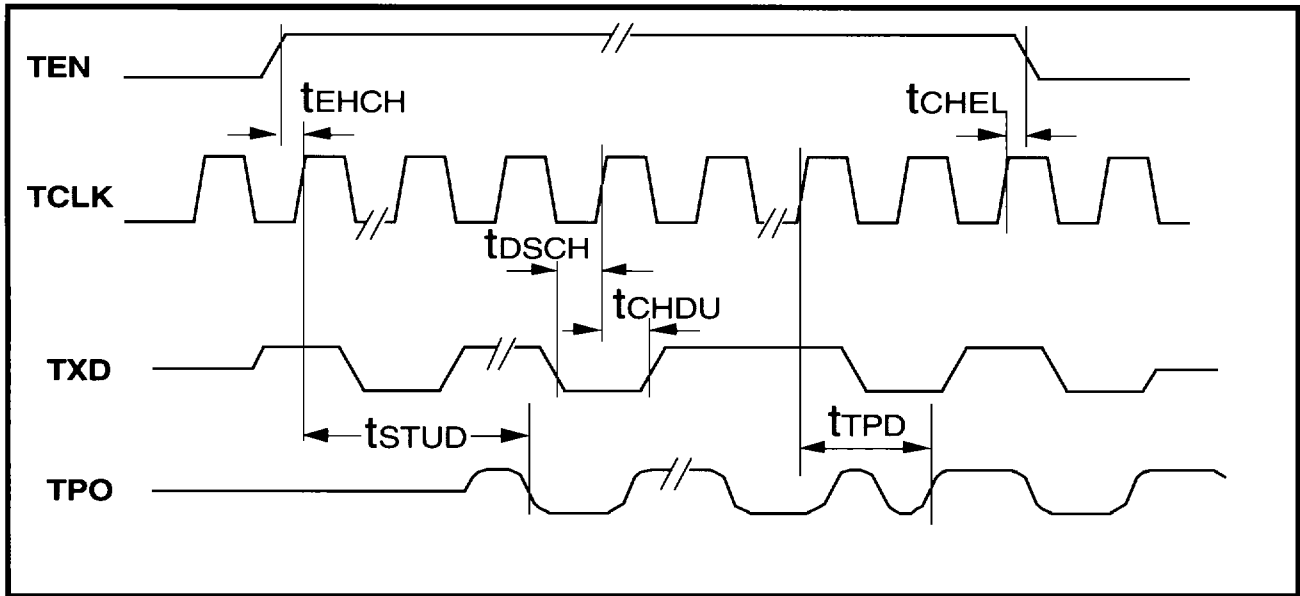
Figure 36: Mode 4 Transmit Timing
