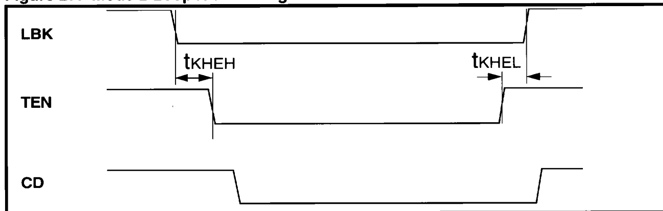
Figure 27: Mode 2 Loopback Timing
