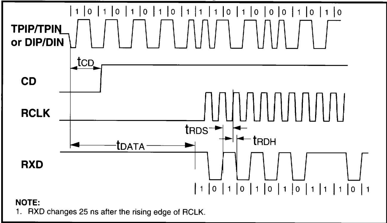
Figure 16: Mode 1 RCLK/Start-of-Frame Timing
