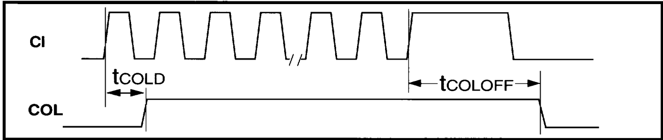
Figure 37: Mode 4 Collision Detect Timing
