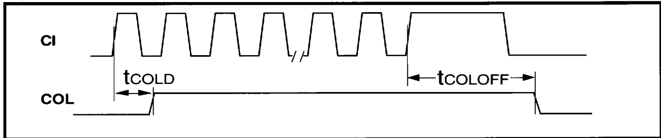
Figure 20: Mode 1 COL/CI Output Timing
