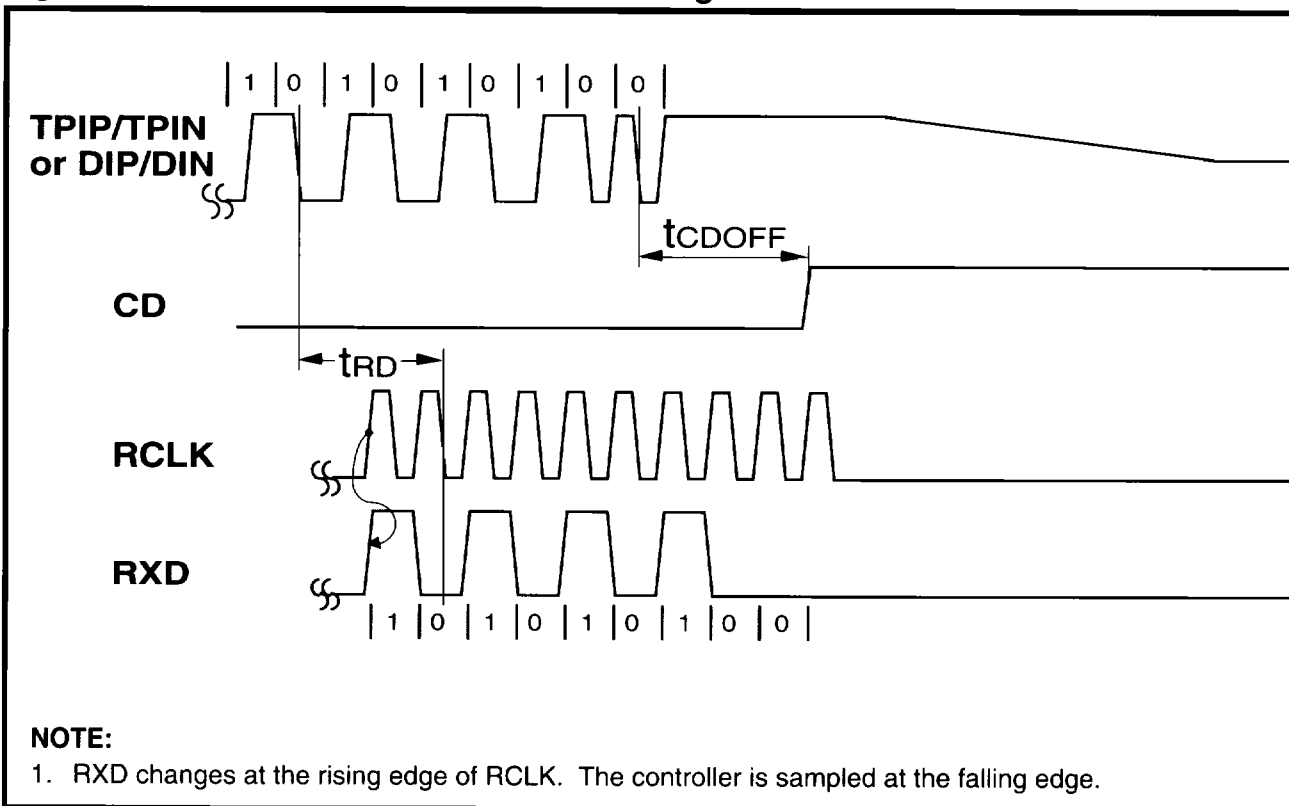
Figure 23: Mode 2 RCLK/End-of-Frame Timing
