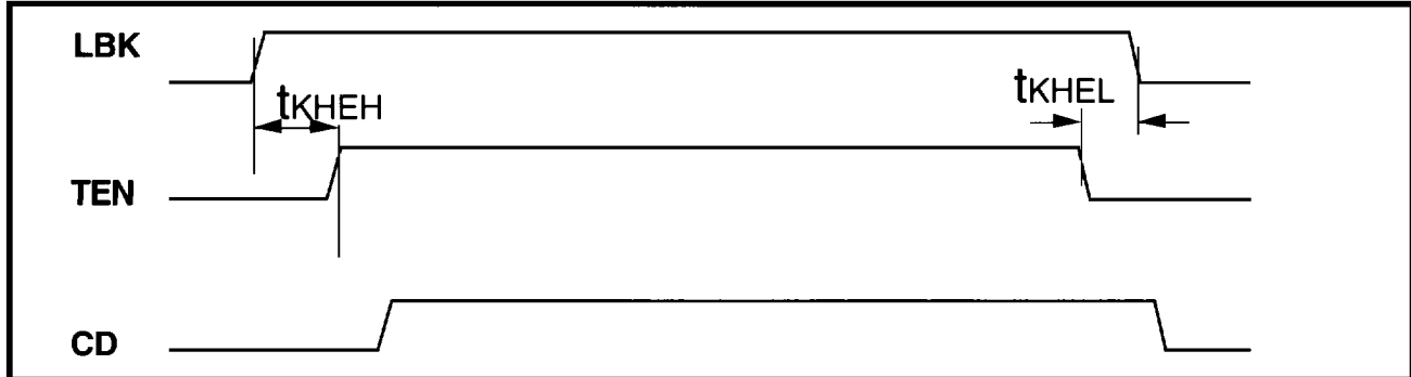
Figure 39: Mode 4 Loopback Timing
