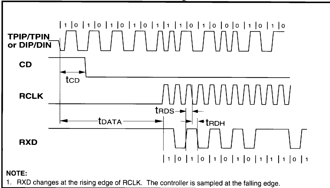
Figure 22: Mode 2 RCLK/Start-of-Frame Timing
