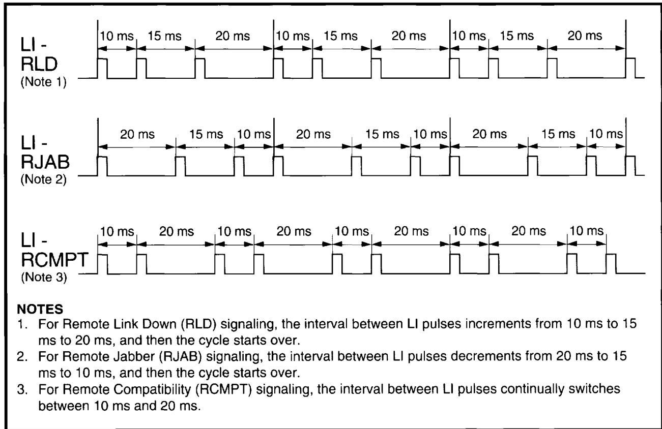
Figure 7: Remote Signaling Link Integrity Pulse Timing
