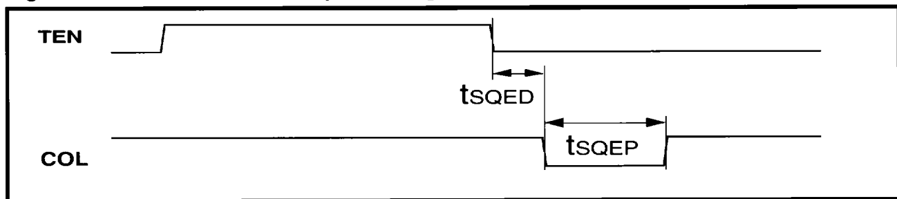
Figure 32: Mode 3 COL/CI Output Timing
