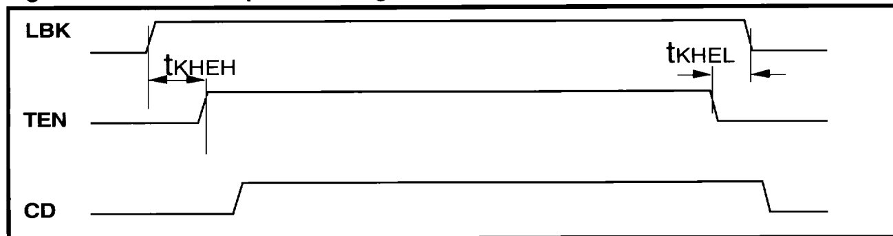
Figure 33: Mode 3 Loopback Timing
