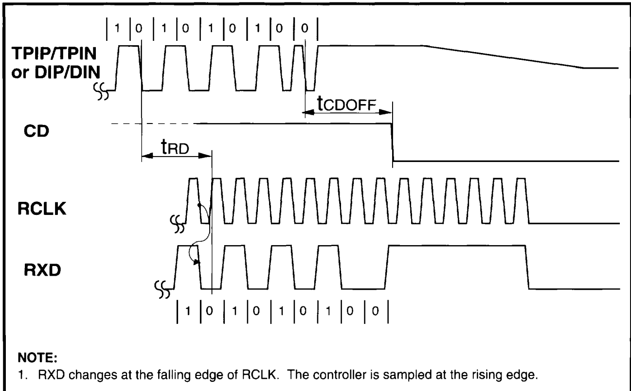
Figure 35: Mode 4 RCLK/End-of-Frame Timing
