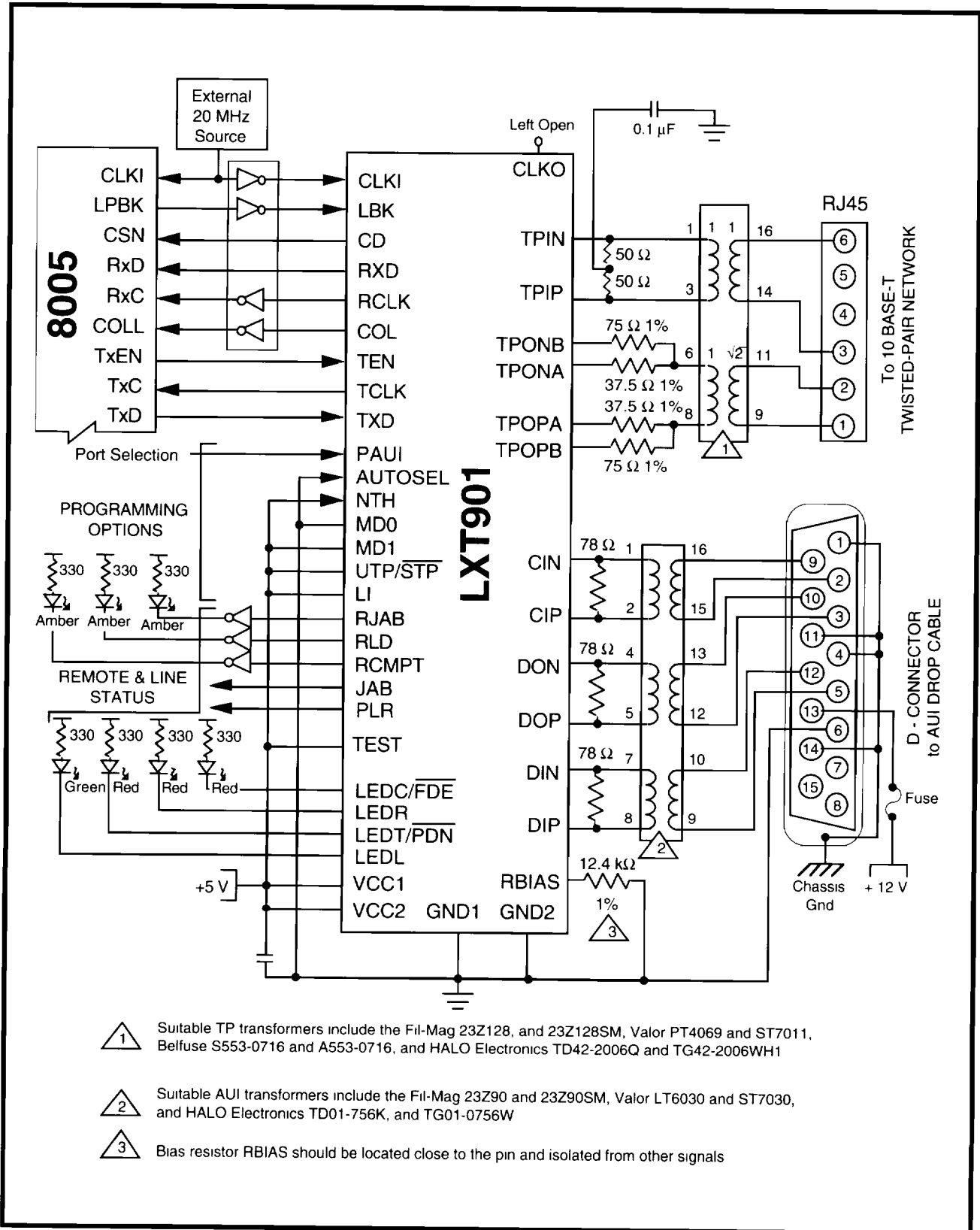
Figure 11: Manual Port Select with Seeq 8005 Controller
