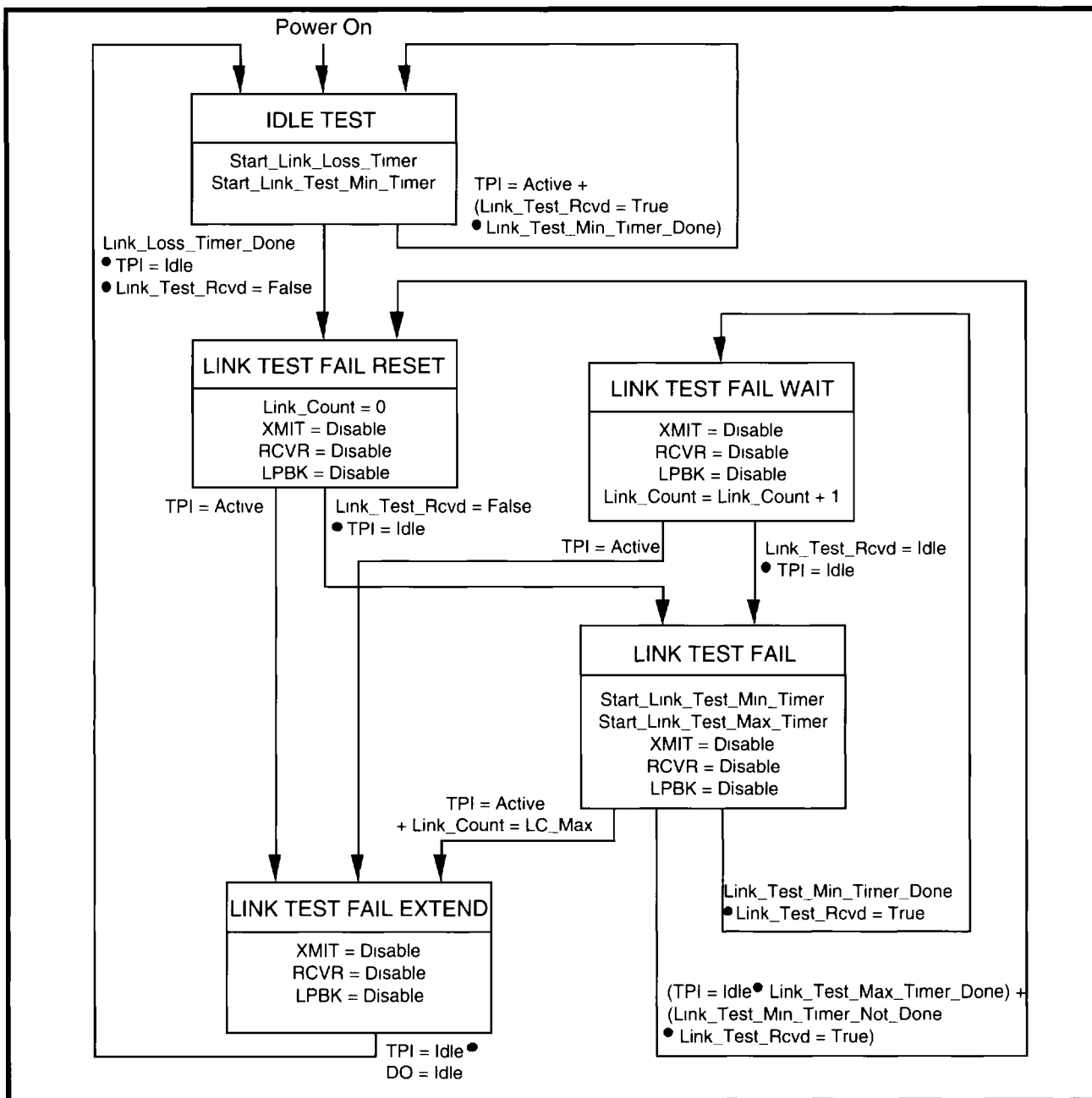
Figure 6: Link Integrity Test Function
