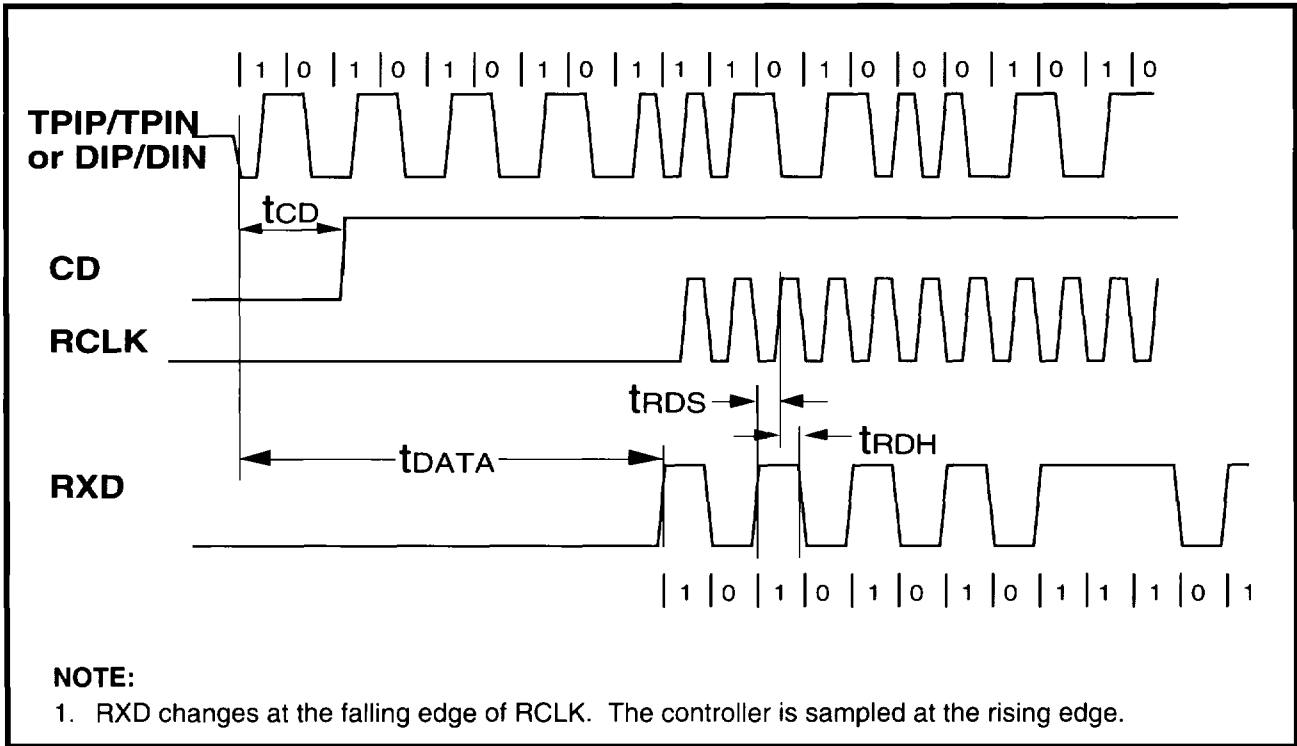
Figure 34: Mode 4 RCLK/Start-of-Frame Timing
