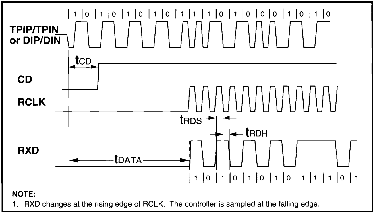
Figure 28: Mode 3 RCLK/Start-of-Frame Timing
