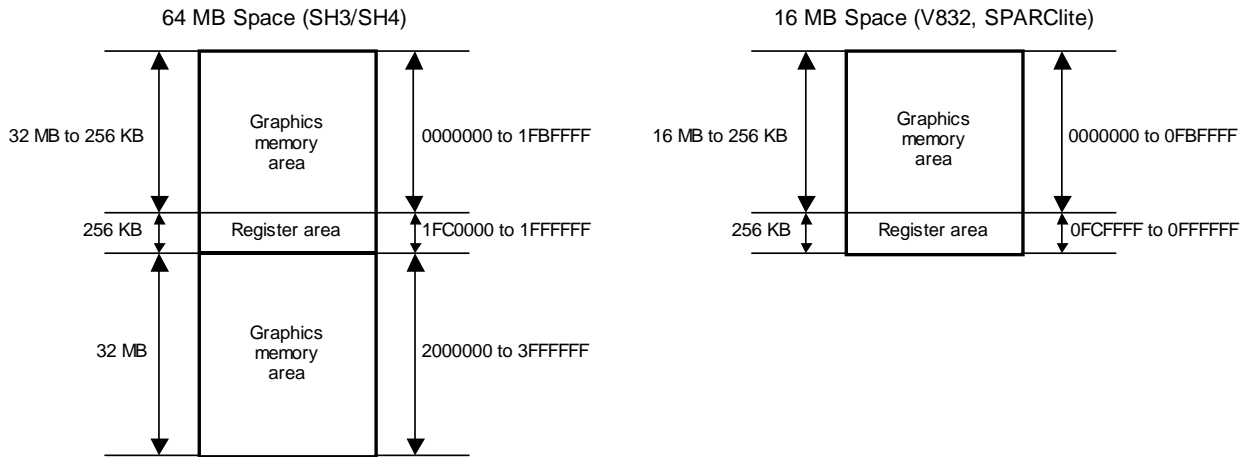
Fig. 4.1 Memory Map
