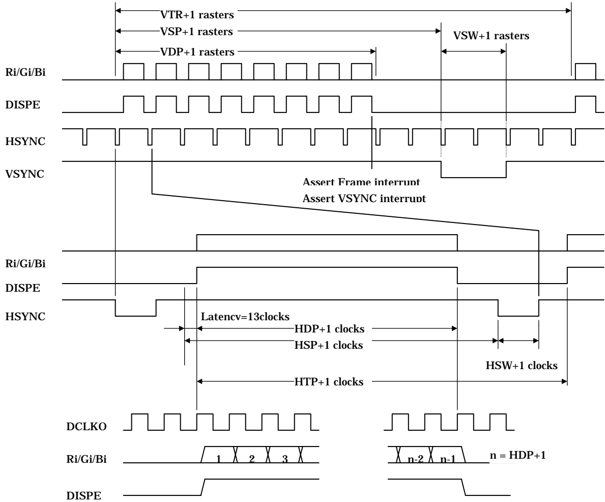
Fig. 10.26 Non-interlace Timing
