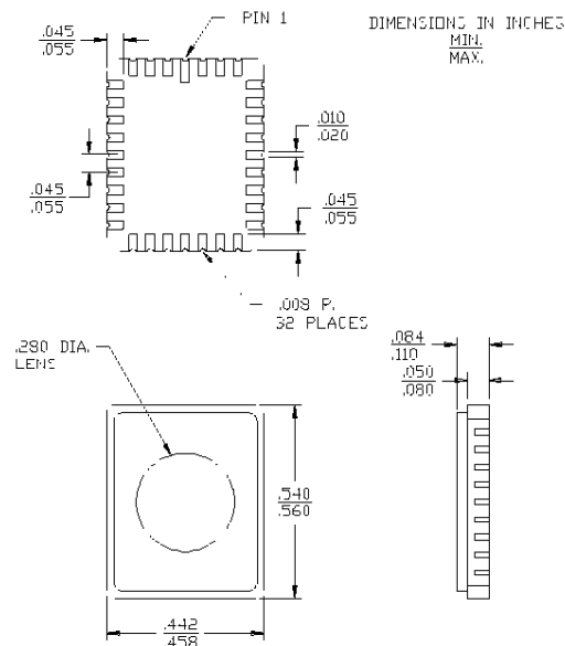
32-Pin Windowed Rectangular Leadless Chip Carrier Q55
