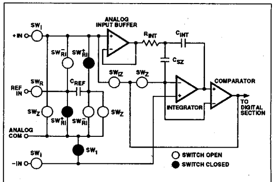
Figure 3D. Reference Voltage Integration Phase
