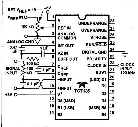
Figure 1. Test Circuit
