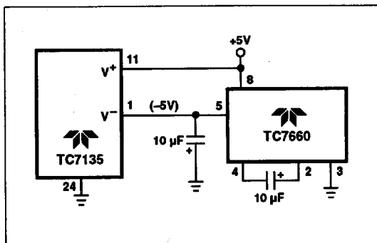
Figure 9. Negative Supply Voltage Generator
