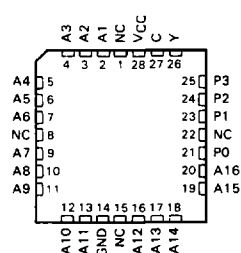
SN54HC678 . . . FK PACKAGE (TOP VIEW)
