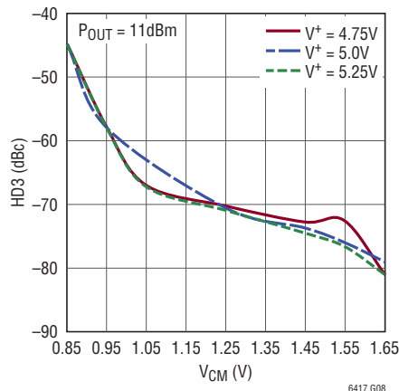
HD3 at 140MHz vs V_{CM} Over V^+
