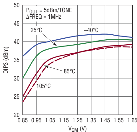
OIP3 at 380MHz vs V_{CM} Over Temperature
