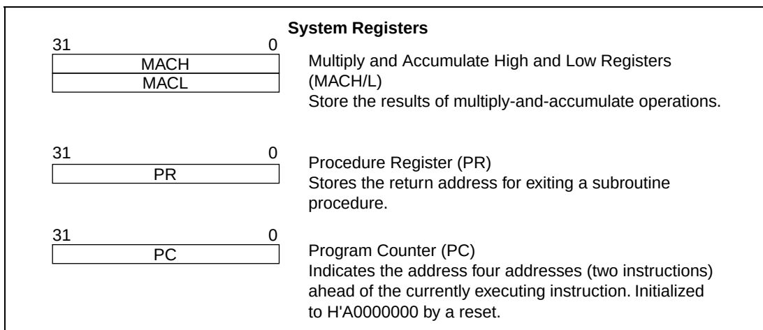
Figure 2.4 System Registers
