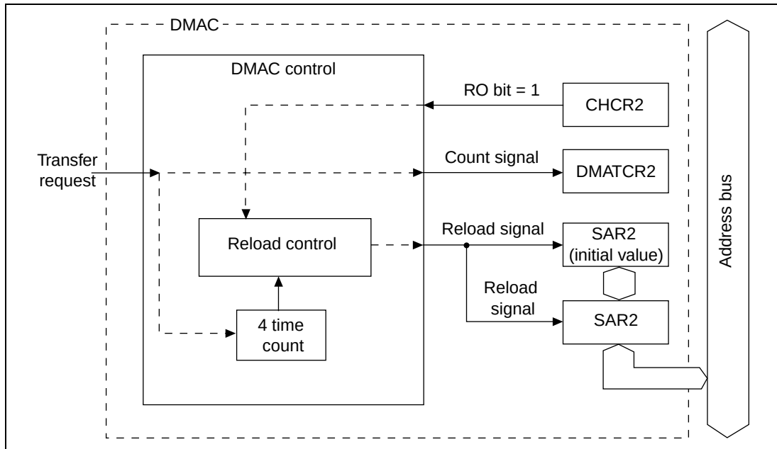
Figure 11.22 Source Address Reload Function Diagram
