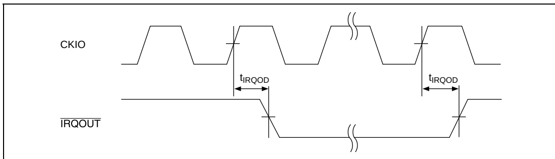
Figure 23.13 \overline{IRQOUT} Timing
