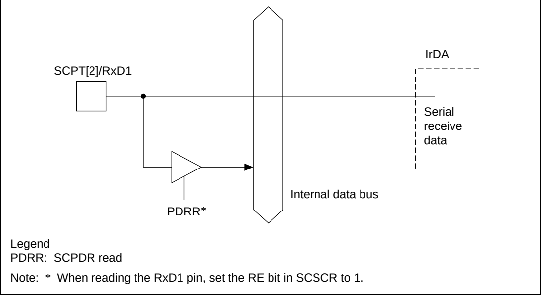
Figure 17.4 SCPT[2]/RxD1 Pin
