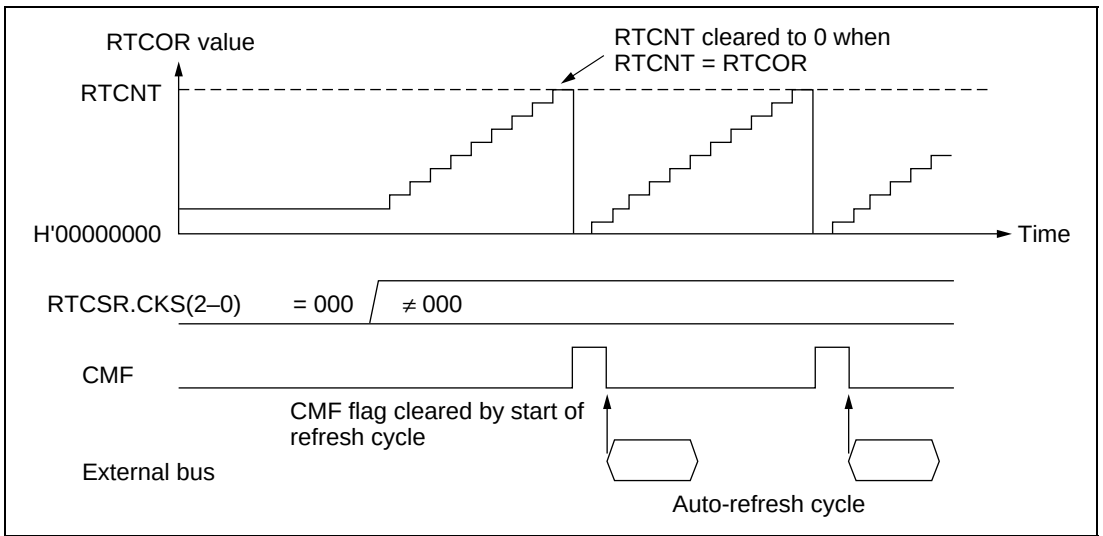
Figure 10.25 Auto-Refresh Operation
