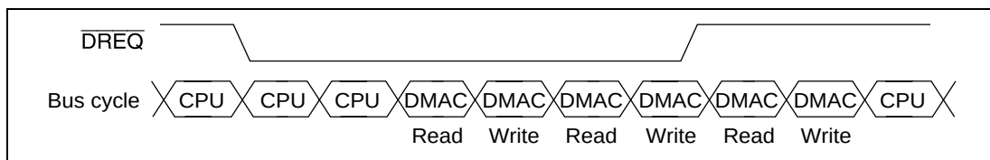
Figure 11.13 Example of Transfer in Burst Mode
