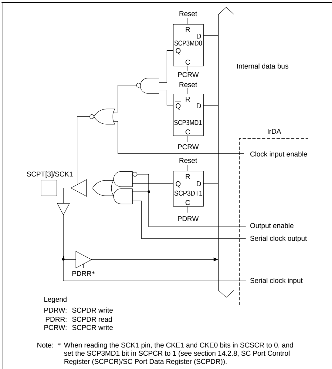
Figure 17.2 SCPT[3]/SCK1 Pin
