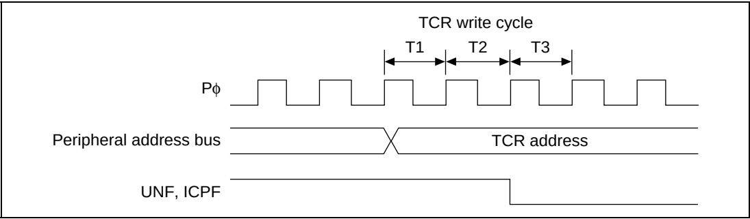
Figure 12.9 Status Flag Clearing Timing
