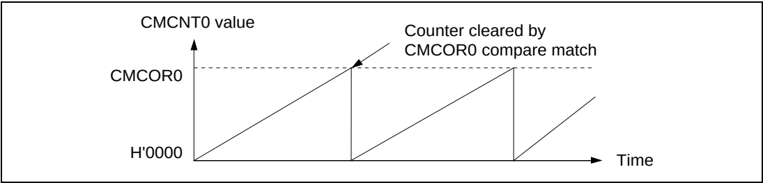
Figure 11.25 Counter Operation
