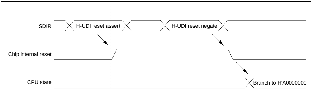
Figure 22.3 H-UDI Reset
