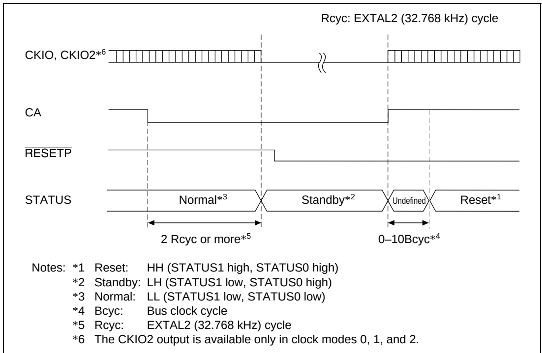
Figure 8.10 Hardware Standby Mode (When CA Goes Low in Normal Operation)
