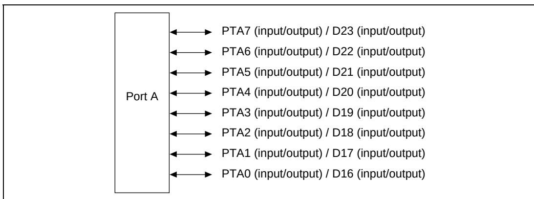
Figure 19.1 Port A
