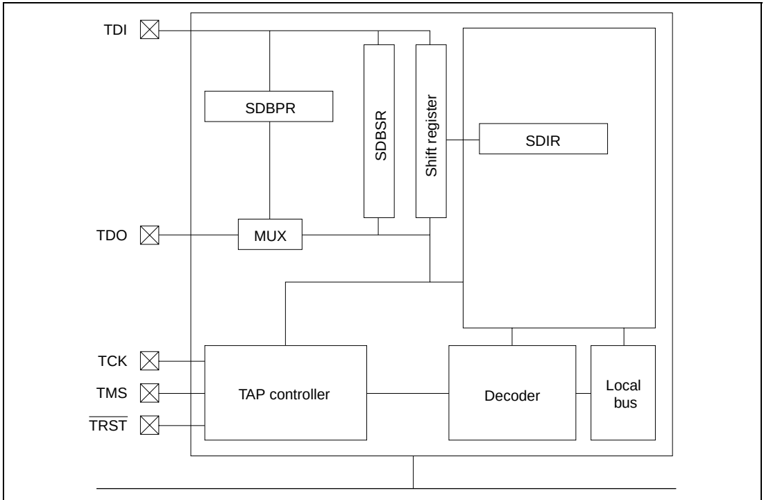
Figure 22.1 Block Diagram of H-UDI
