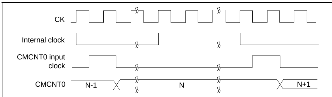
Figure 11.26 Count Timing
