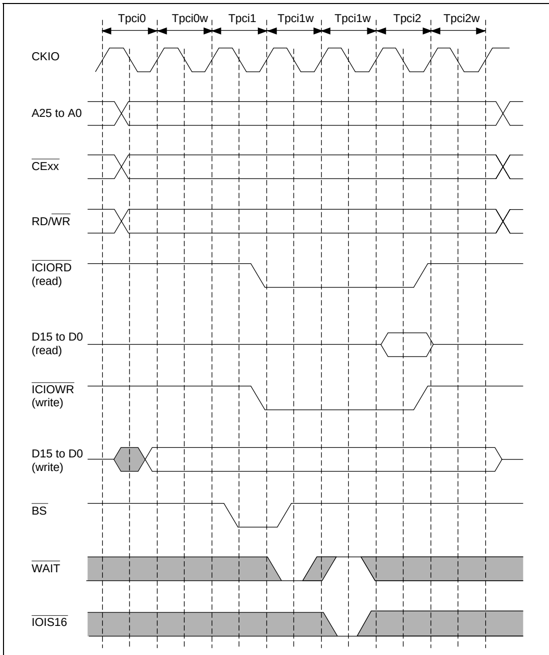
Figure 10.38 Wait Timing for PCMCIA I/O Card Interface
