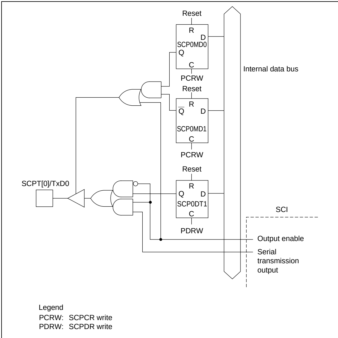
Figure 14.3 SCPT[0]/TxD0 Pin
