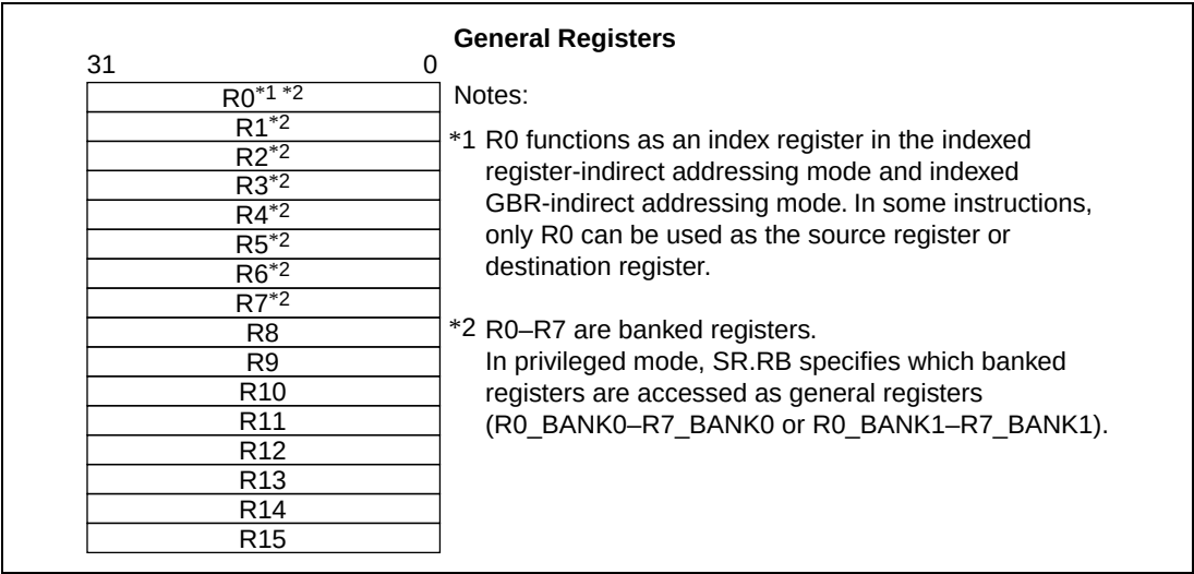
Figure 2.3 General Registers
