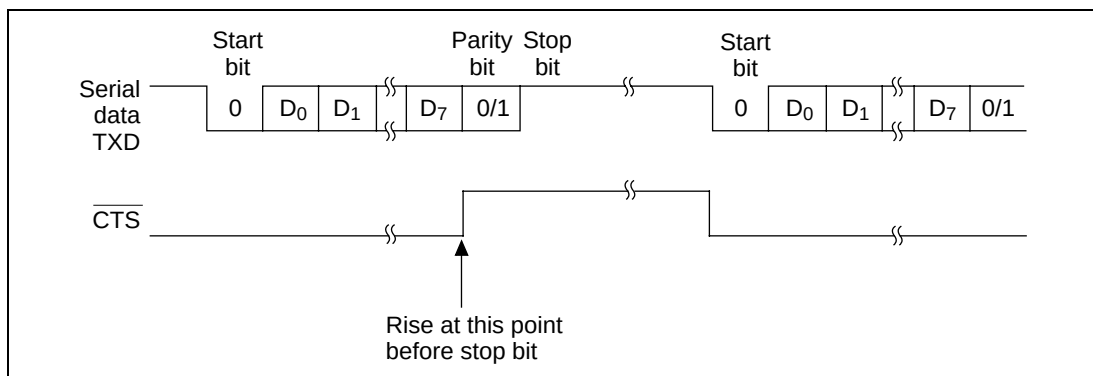
Figure 16.8 Example of Operation Using Modem Control ( \overline{\text{CTS}} )
