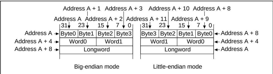
Figure 2.7 Data Format in Memory
