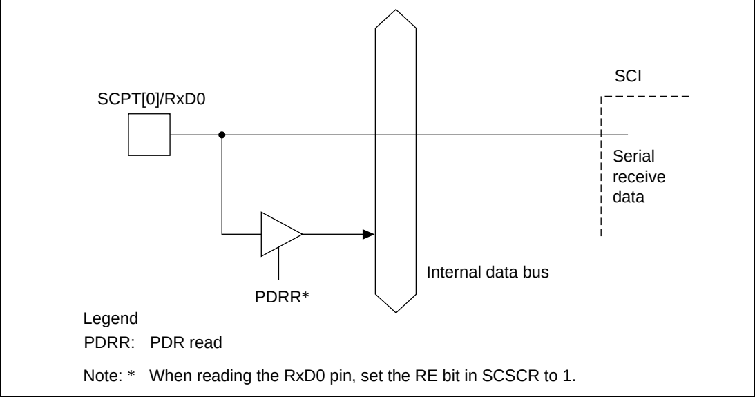
Figure 14.4 SCPT[0]/RxD0 Pin
