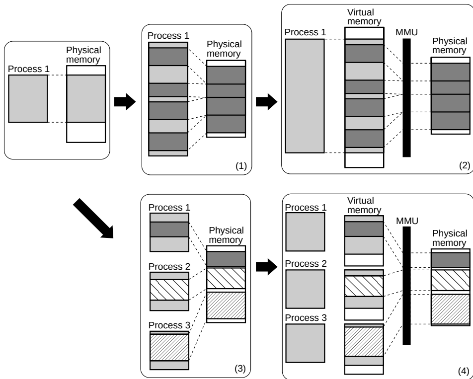
Figure 3.1 MMU Functions
