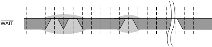
Figure 10.29 Burst ROM Wait Access Timing
